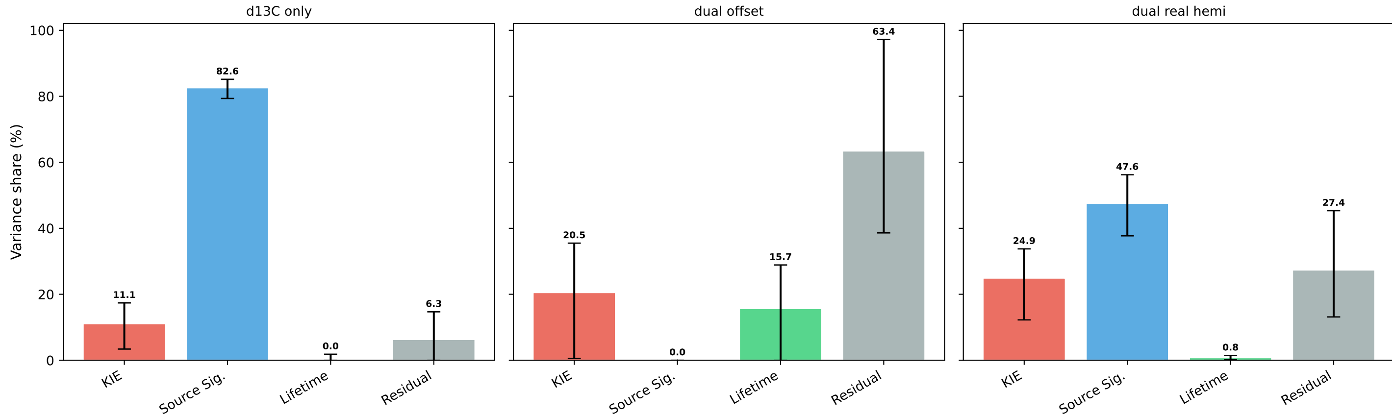
Fig. S6: Bootstrap 95% CIs on Variance Decomposition
