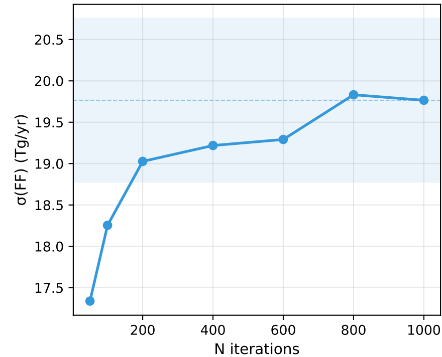
(a) \sigma(\text{FF})
