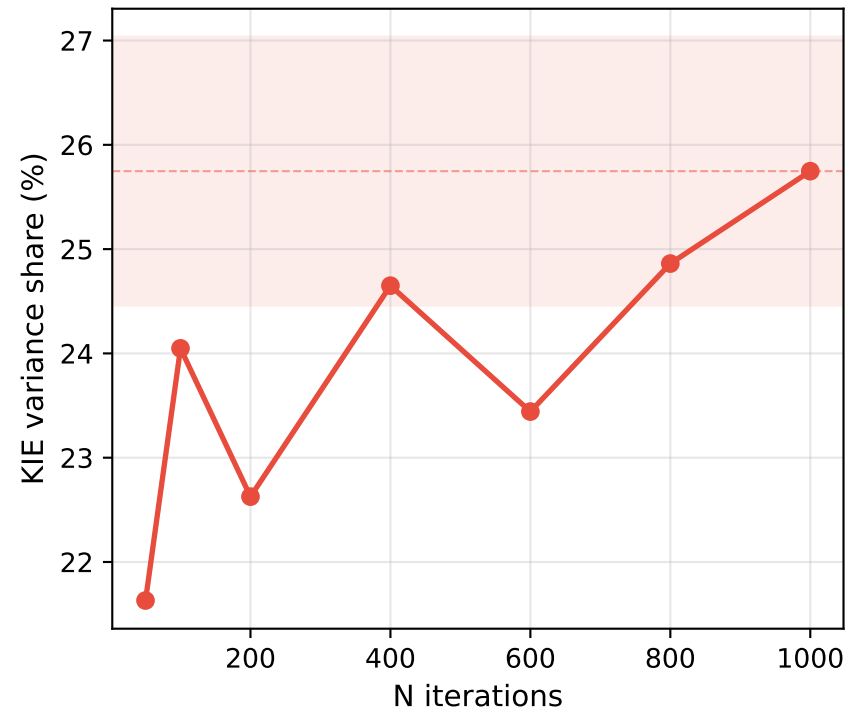
(c) KIE%
