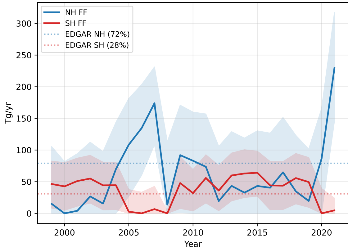
NH/SH FF Partition vs. EDGAR
