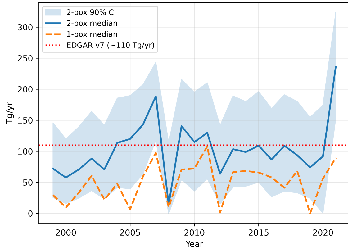
Global Fossil Fuel Emissions
