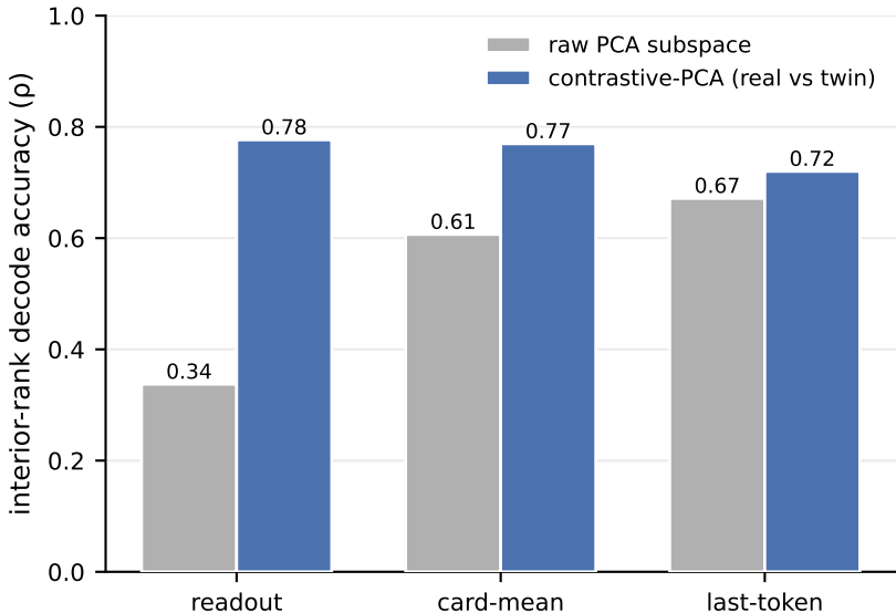
Fig 1 · Low-variance ordinal subspace: rank is PCA-invisible but cPCA-recoverable
