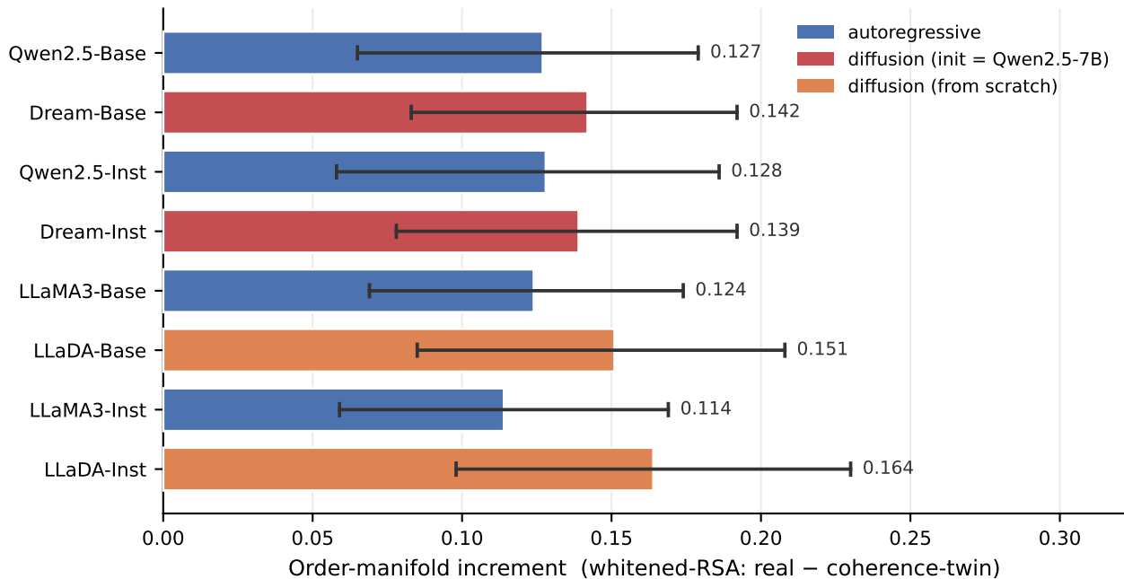
Fig 4 · The in-context order manifold is objective-invariant (E10)
