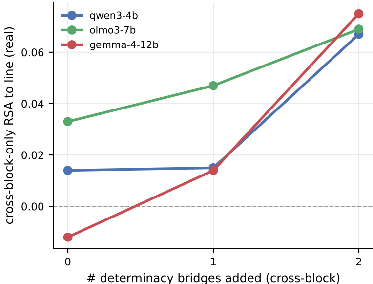
Fig 6 · E4 determinacy dose-response (cross-block map rises with bridges)
