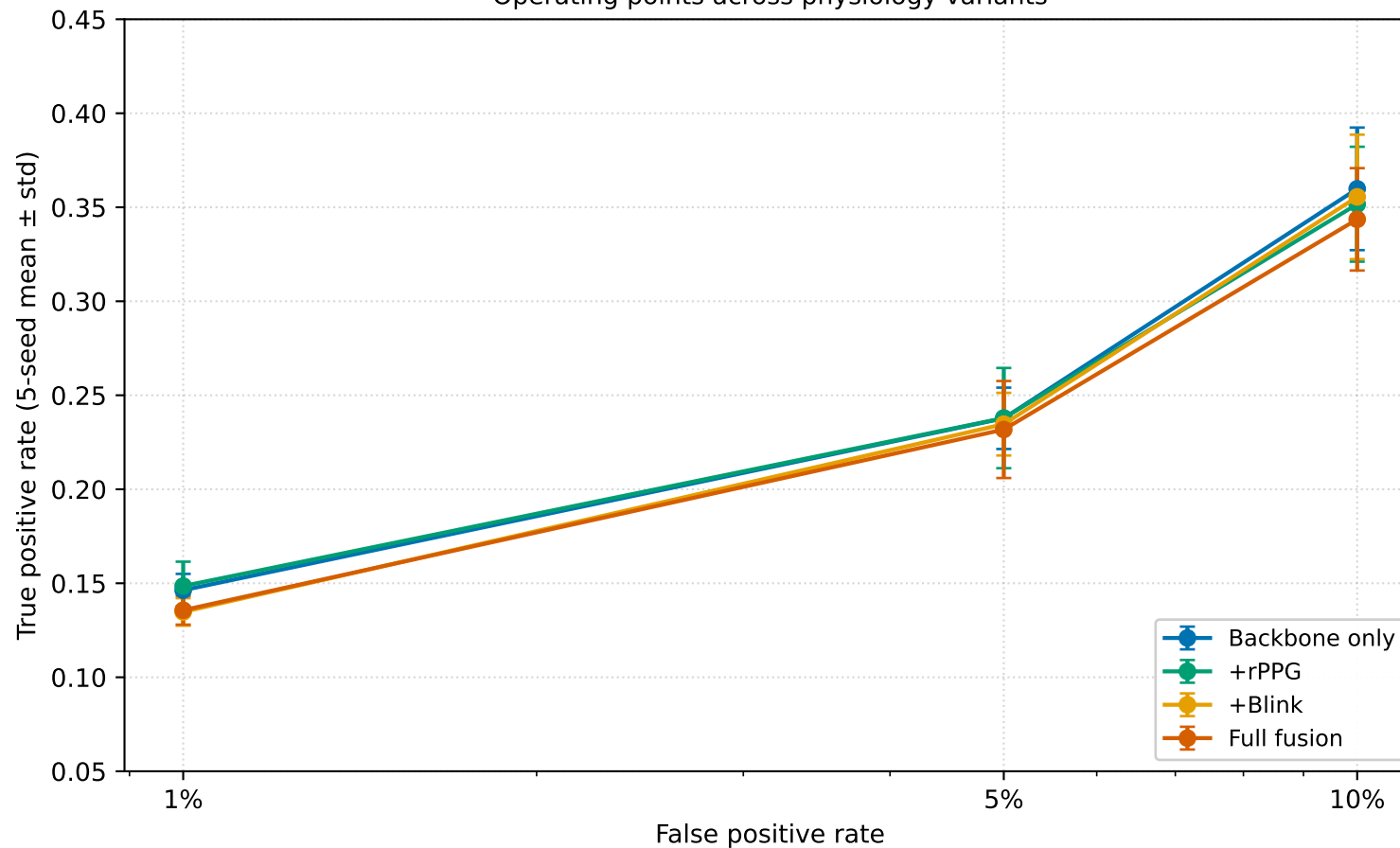
CLIP under strict LODO (CelebDF, n = 1758 , train FF + DFDC) Operating points across physiology variants
