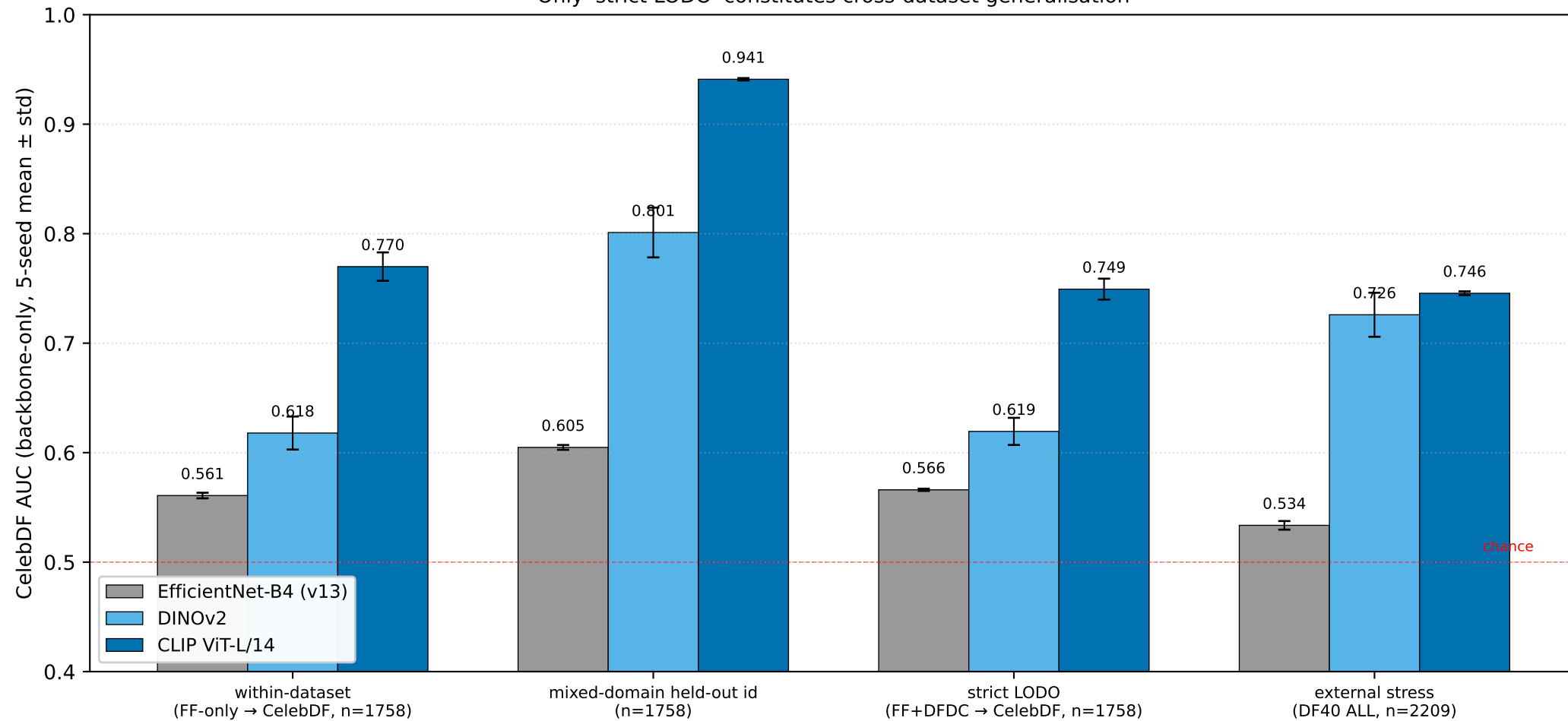
CelebDF detection across four evaluation protocols Only 'strict LODO' constitutes cross-dataset generalisation
