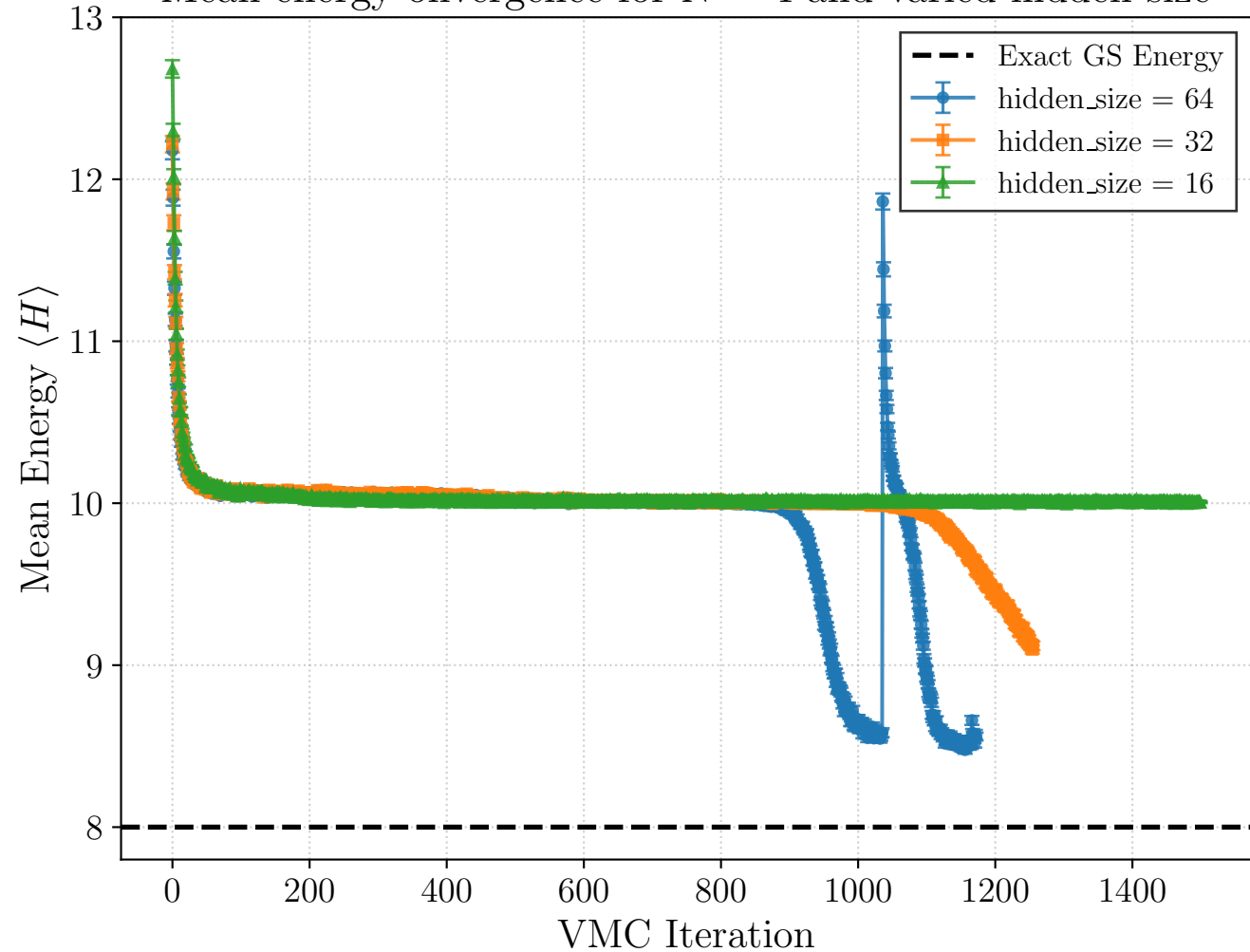
Mean energy convergence for N = 4 and varied hidden size
