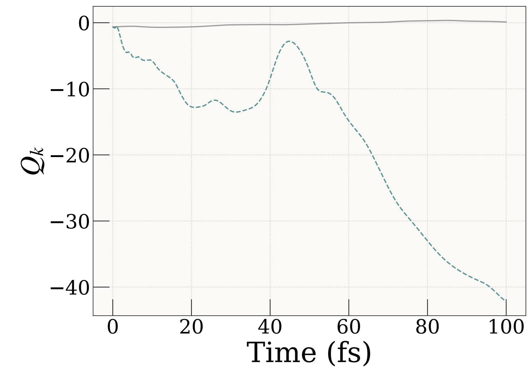
Mode 7 (779 \text{cm}^{-1} )
