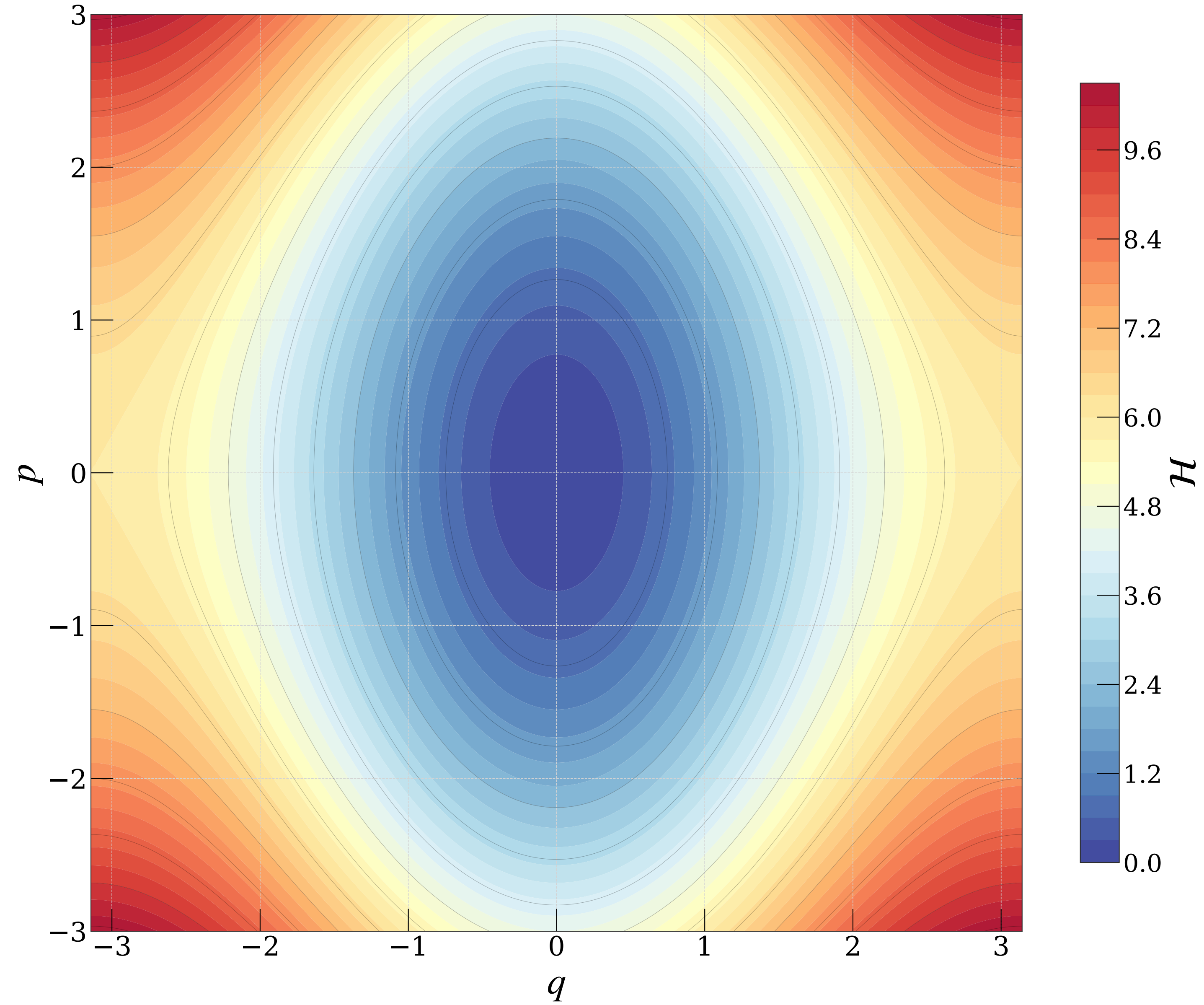
Ideal Pendulum \mathcal{H} = 3(1 - \cos q) + p^2/2
