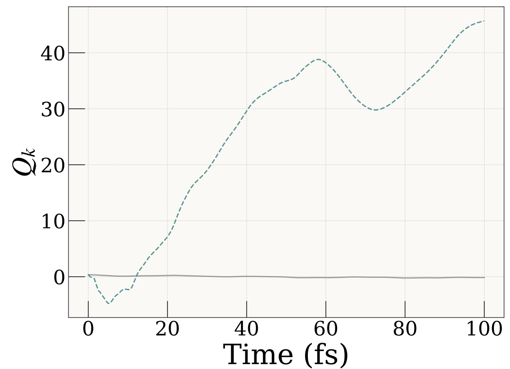
Mode 6 (510 \text{cm}^{-1} )
