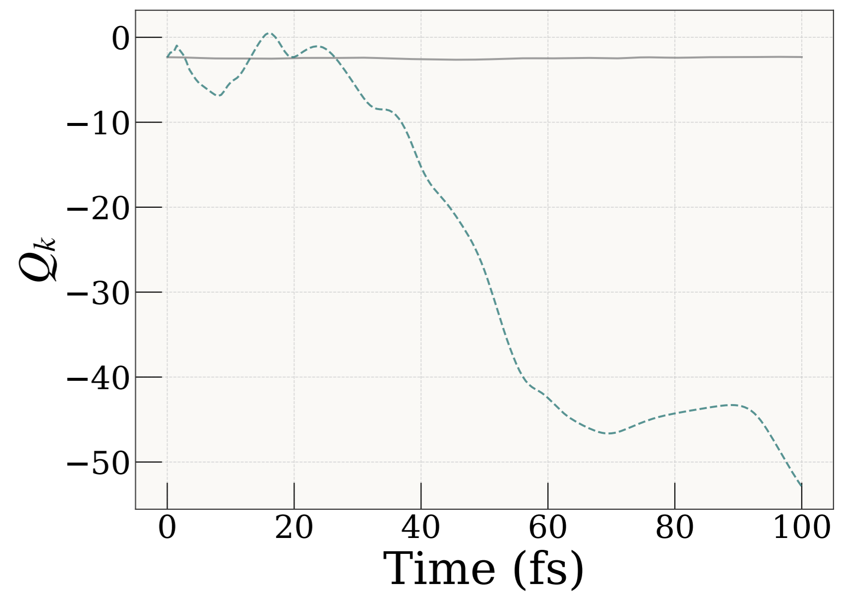
Mode 9 (1070 \text{cm}^{-1} )
