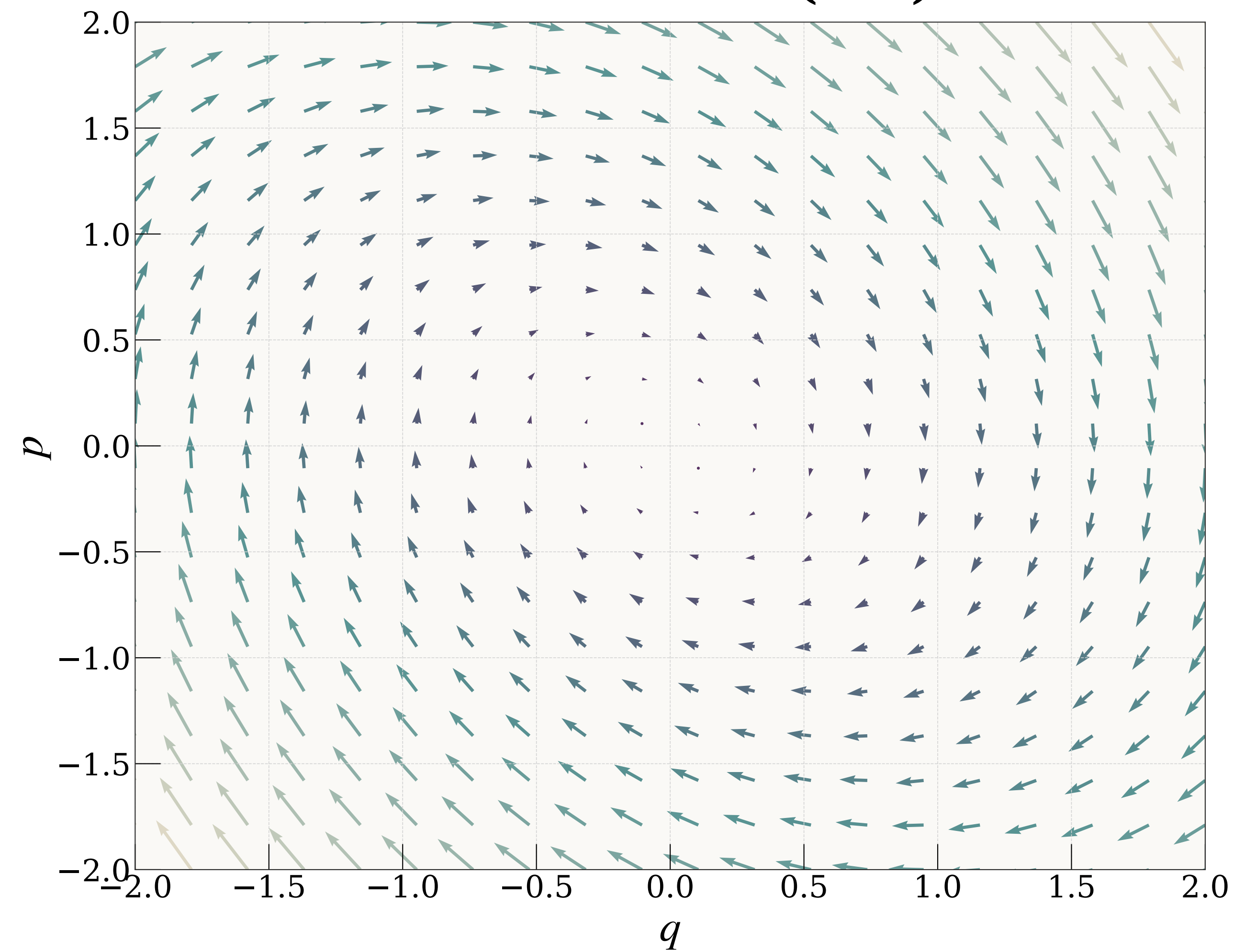
D-HNN Dissipative \rho \nabla D
