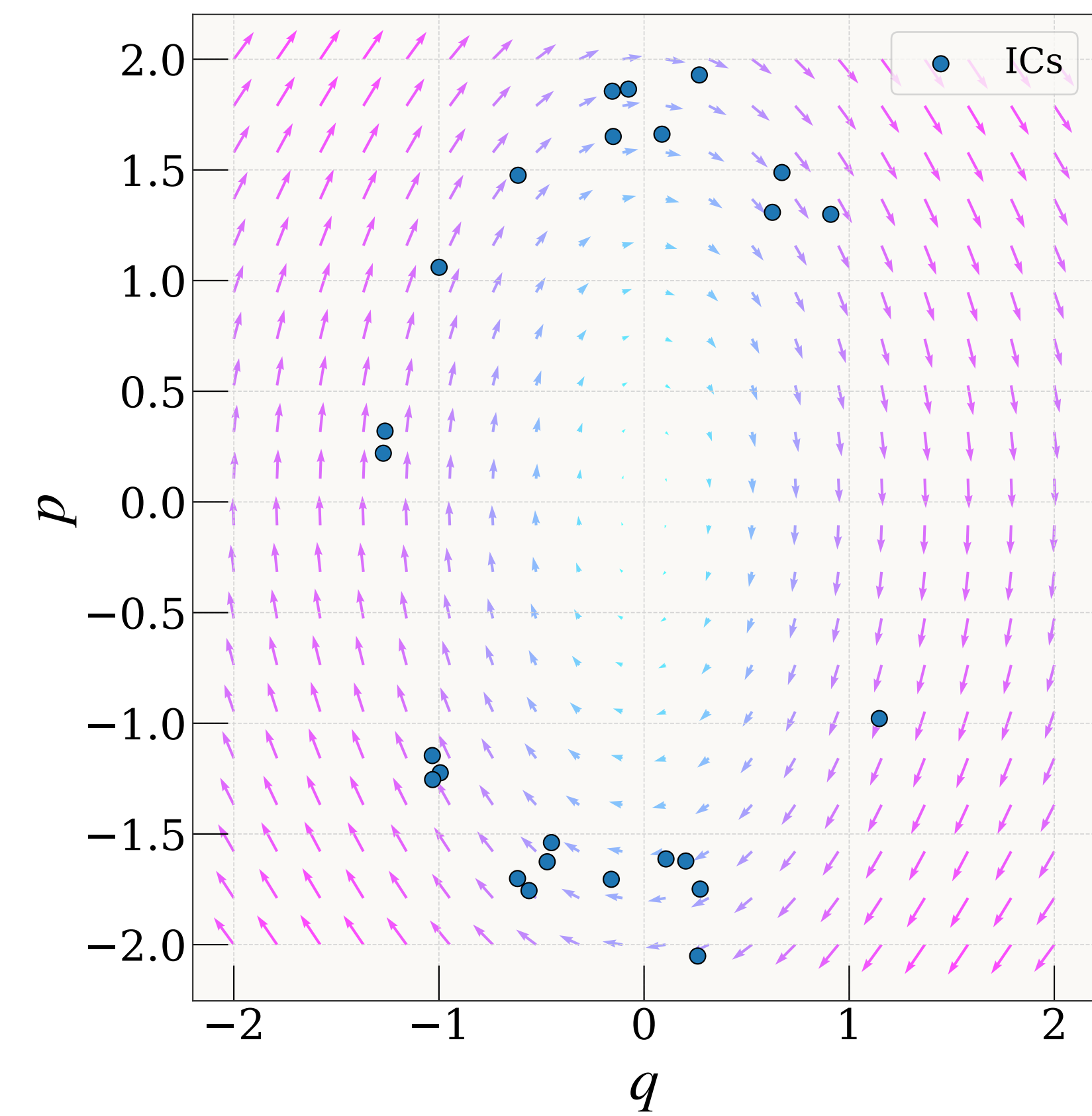
Pendulum — Vector Field
