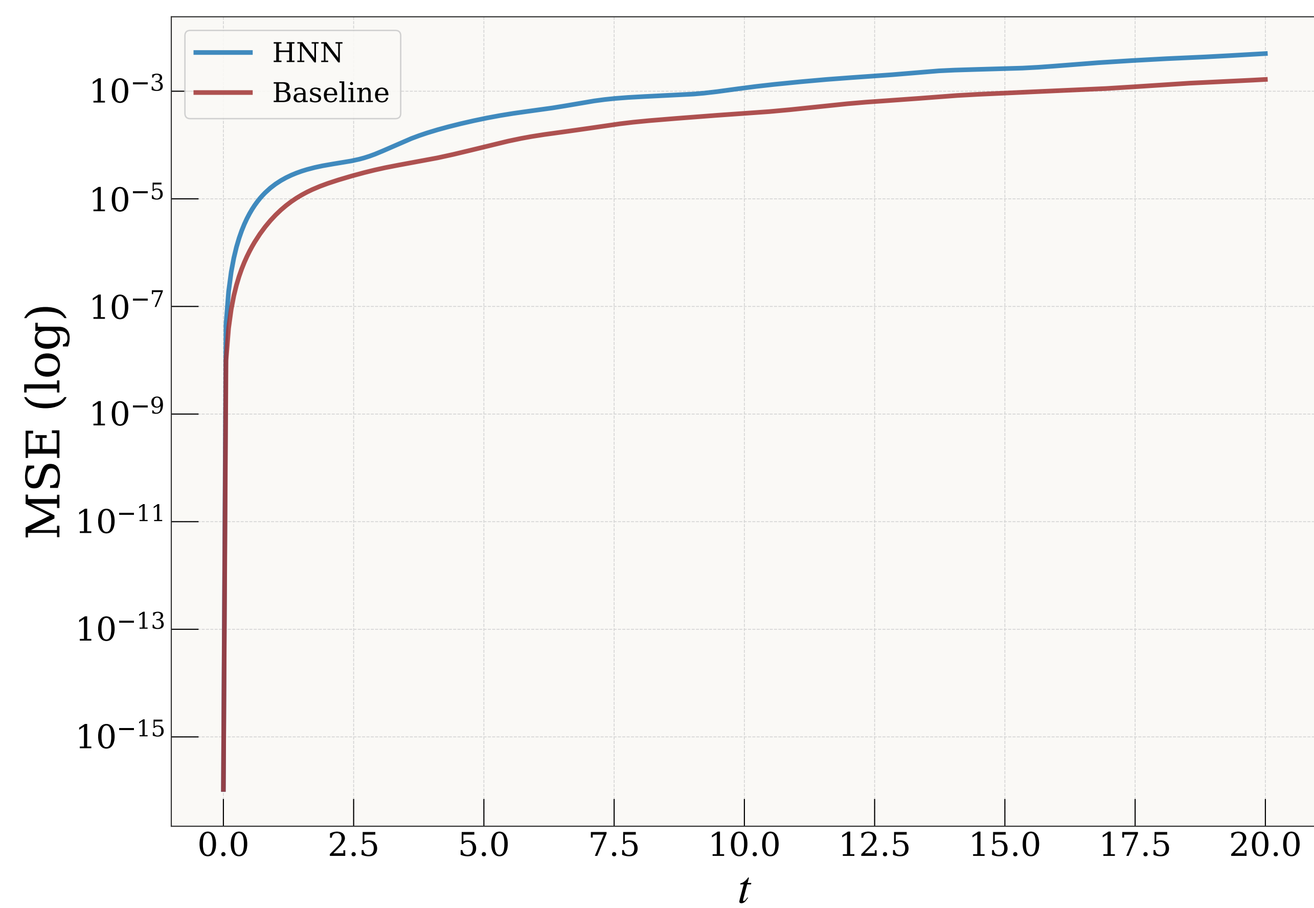
Coordinate MSE
