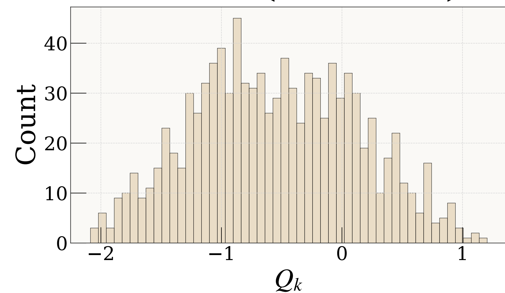
Mode 9 (1083 cm -1 )
