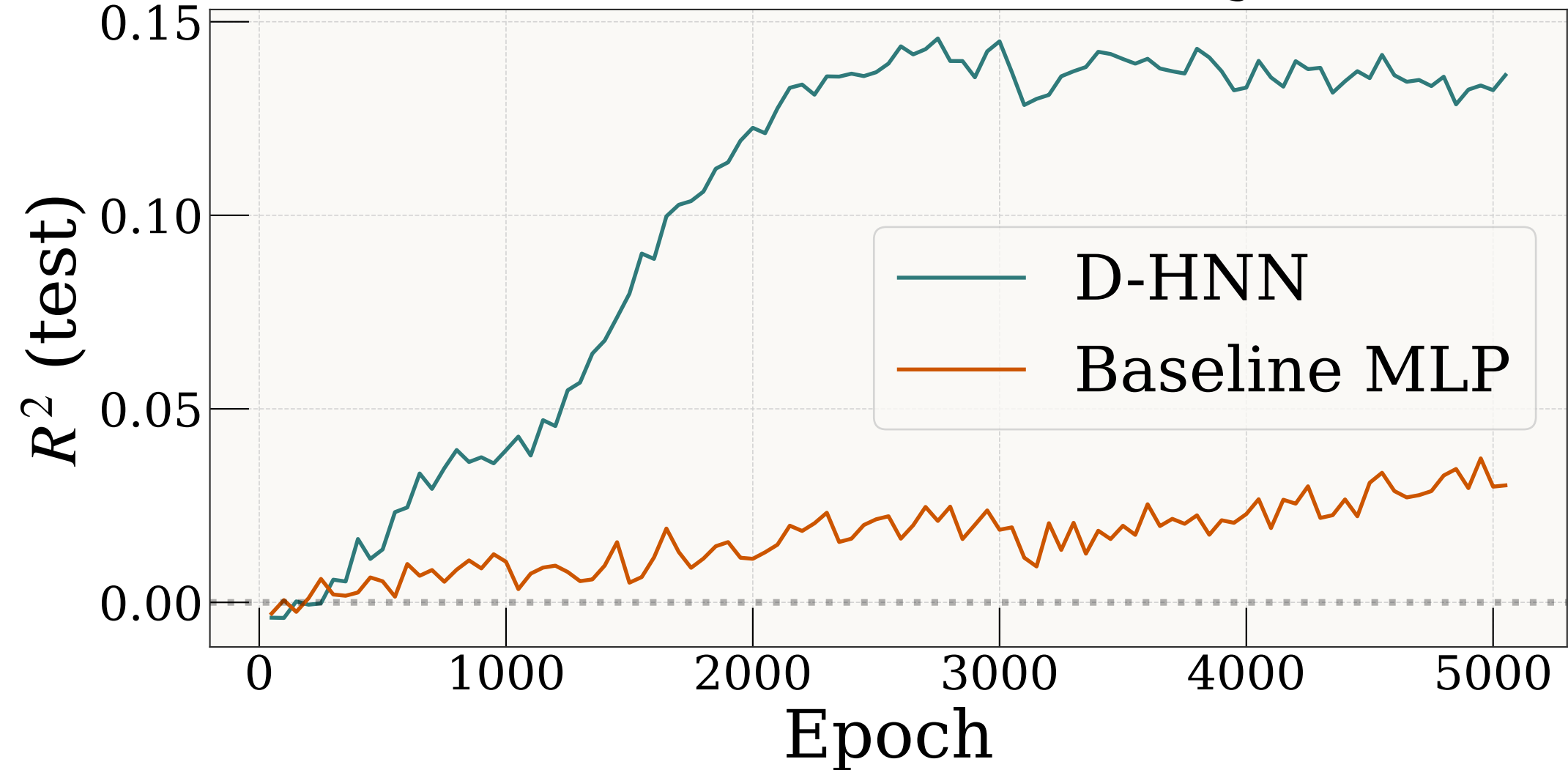
Prediction Quality
