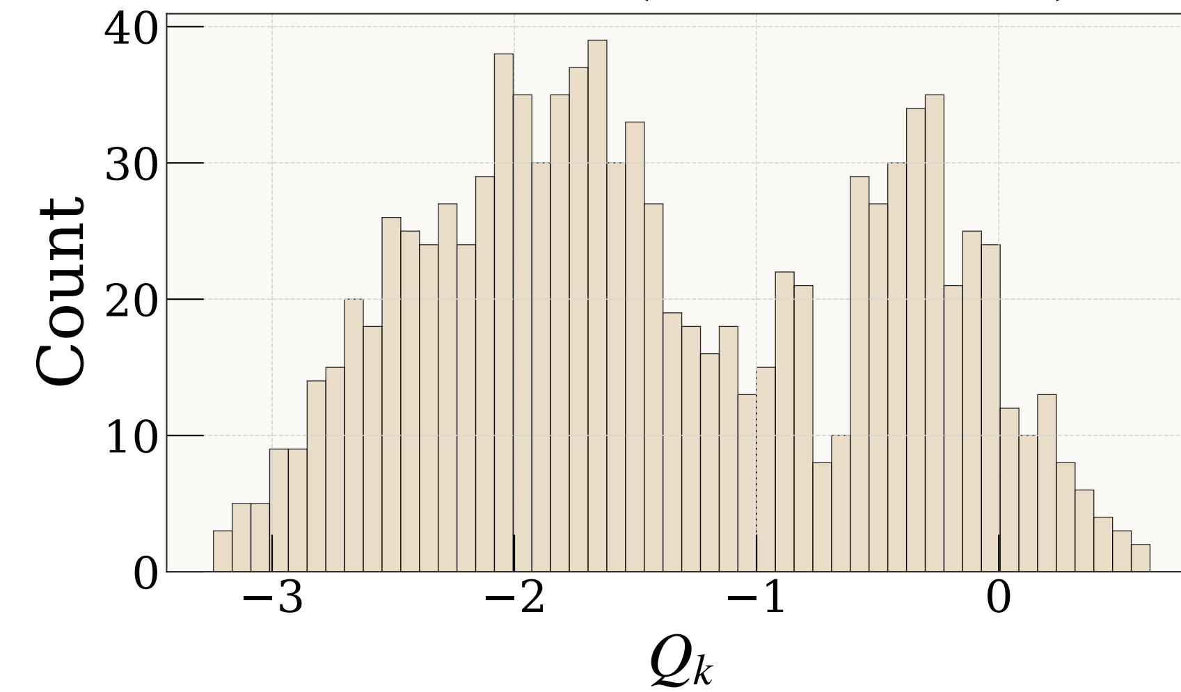
Mode 9 (1070 \text{cm}^{-1} )
