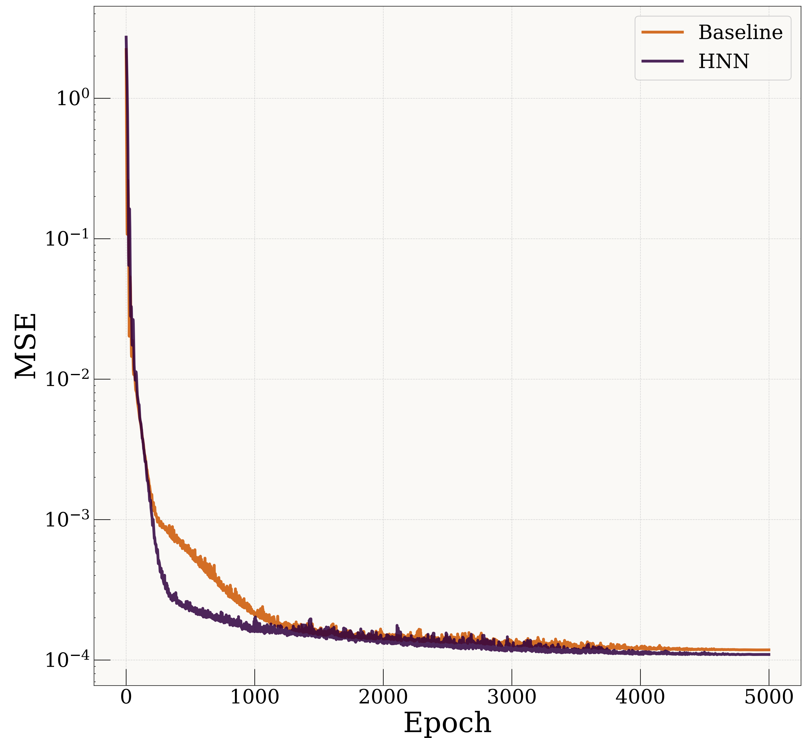
Test Loss
