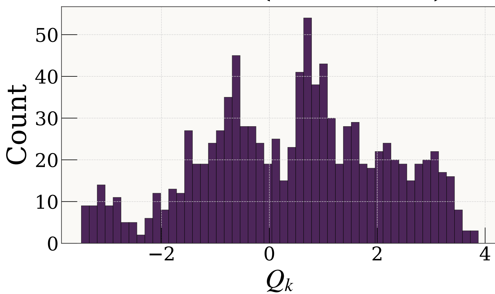
Mode 1 (-216 cm -1 )
