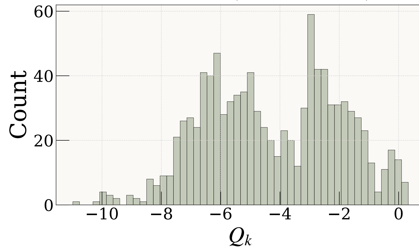
Mode 8 (883 \text{cm}^{-1} )
