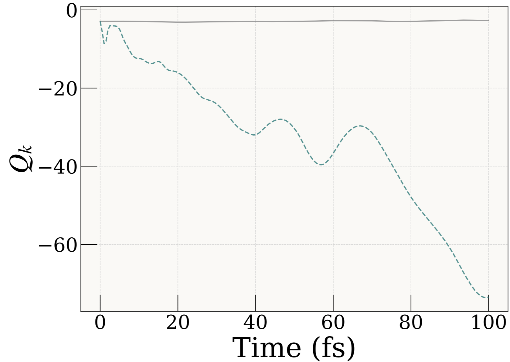
Mode 8 (883 \text{cm}^{-1} )
