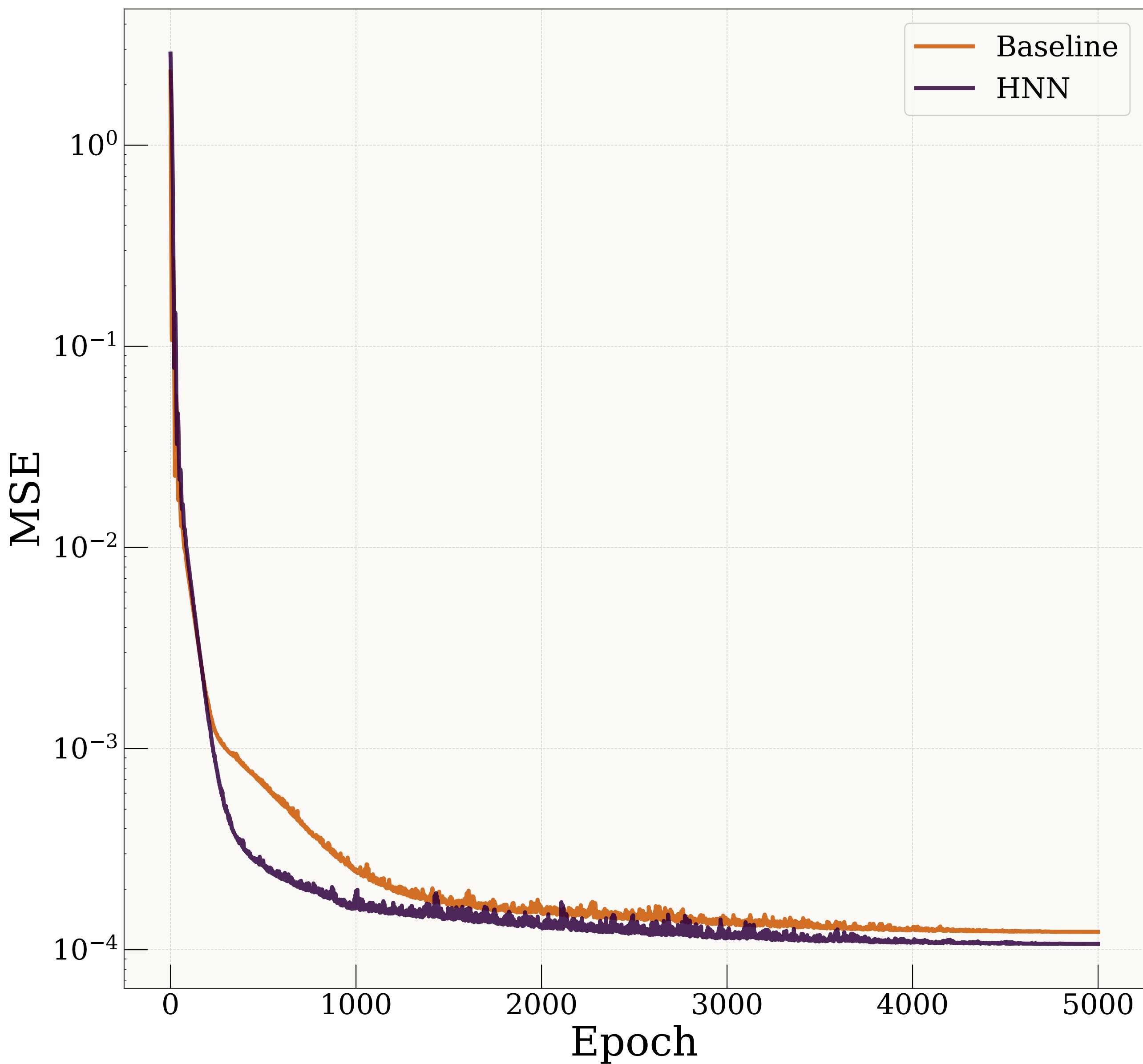
Train Loss
