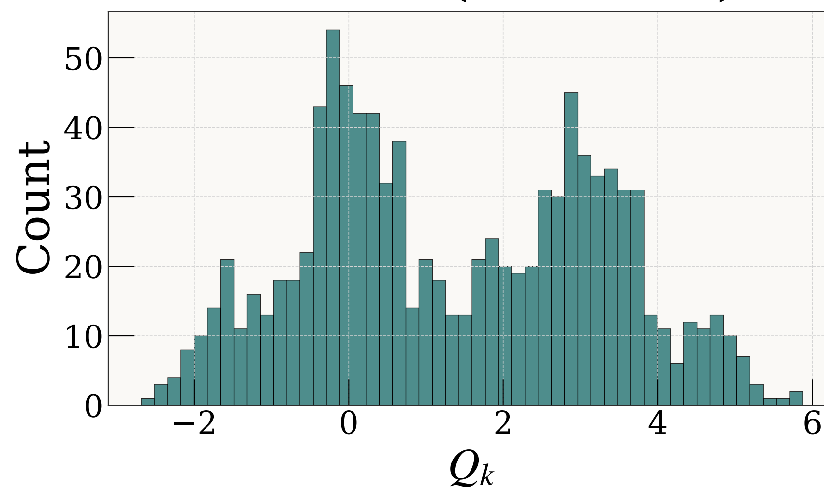
Mode 5 (442 cm -1 )
