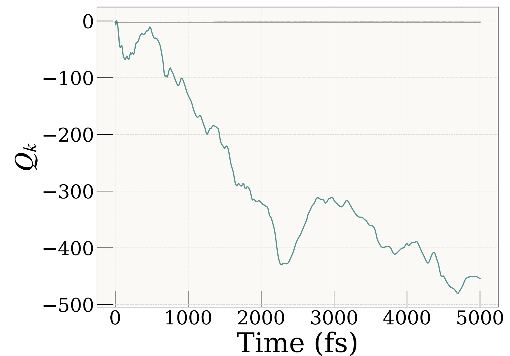
Mode 9 (1070 \text{cm}^{-1} )
