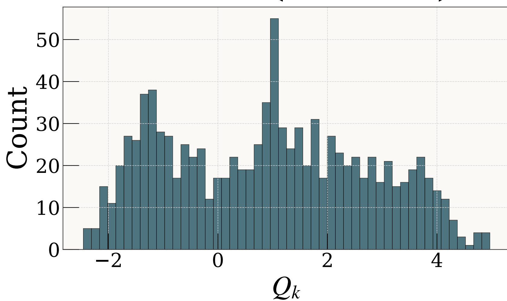
Mode 4 (420 cm -1 )
