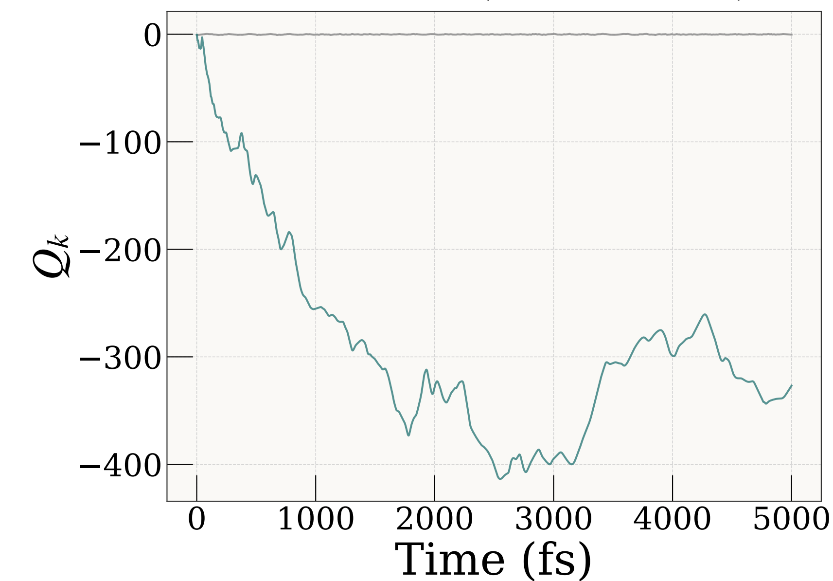
Mode 7 (779 \text{cm}^{-1} )
