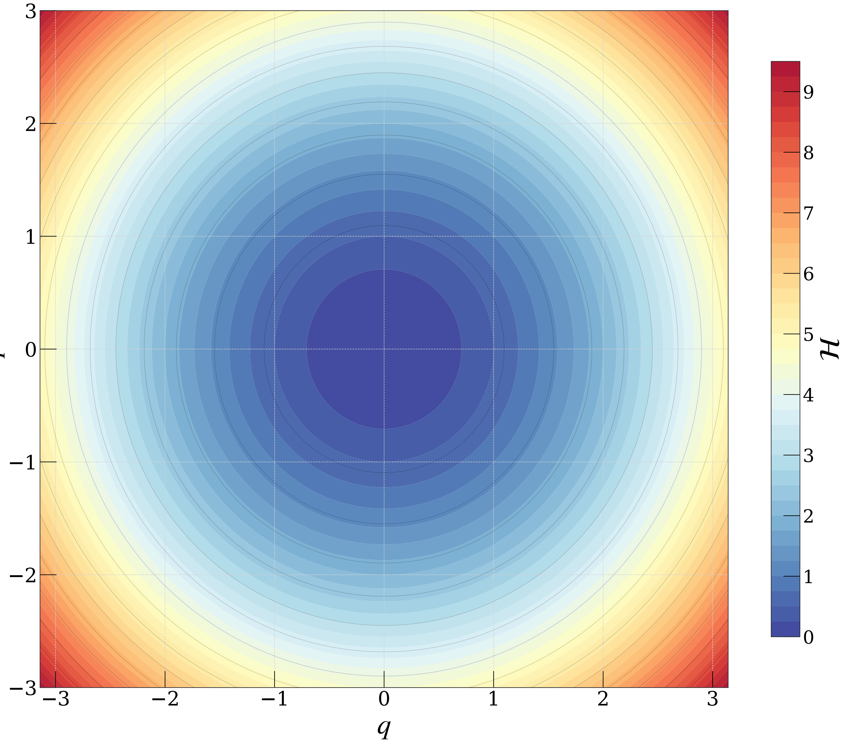
Harmonic Oscillator \mathcal{H} = q^2/2 + p^2/2
