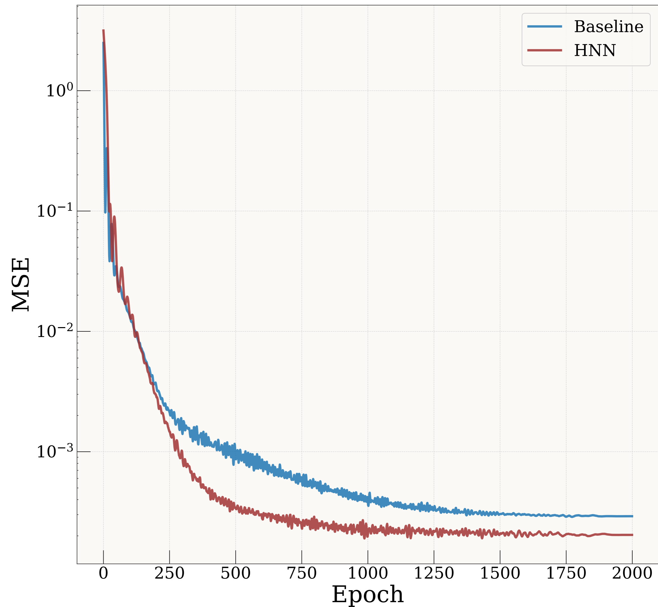
Test Loss
