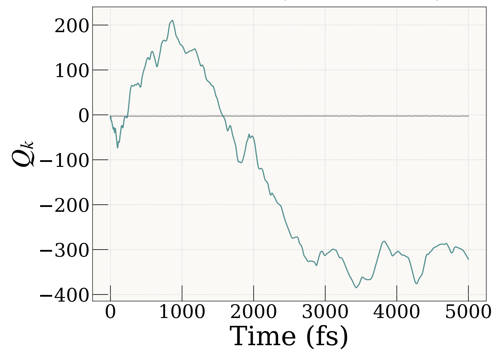
Mode 8 (883 \text{cm}^{-1} )
