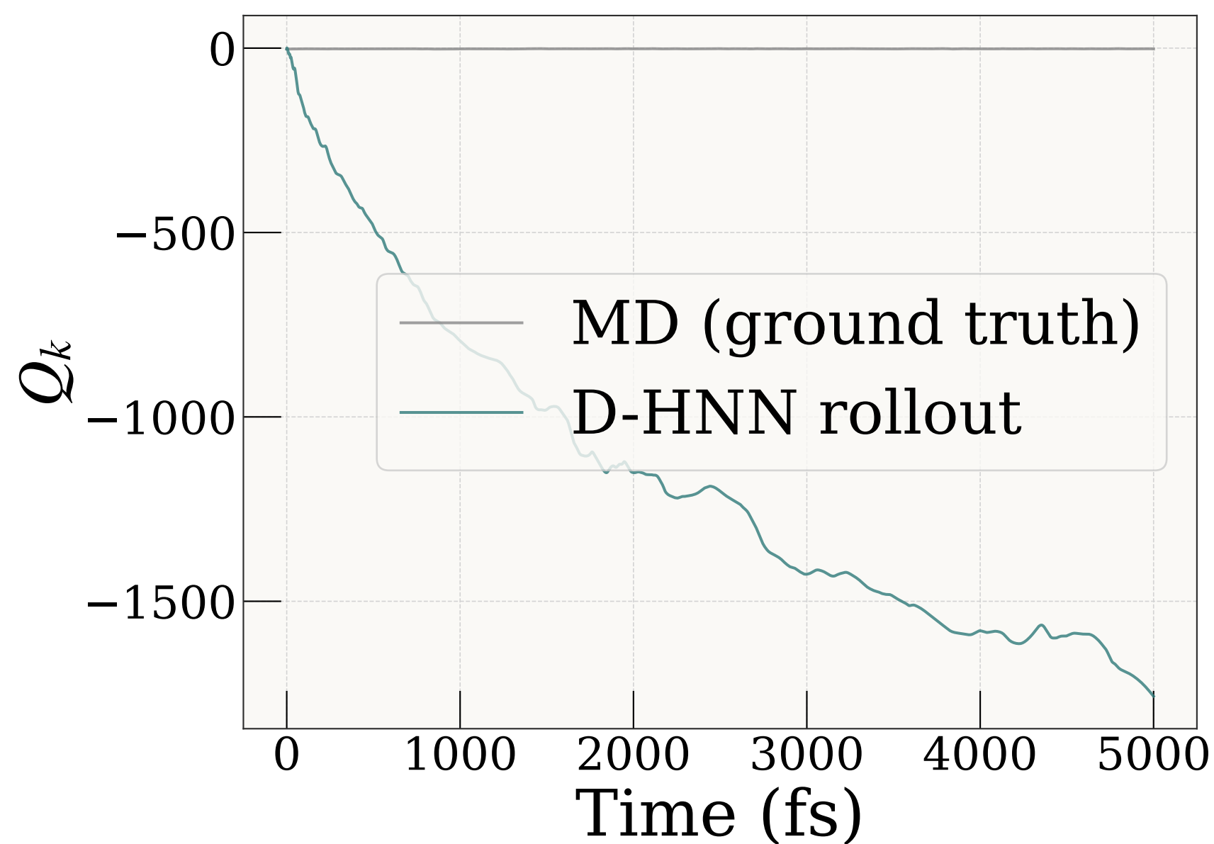
Mode 4 (415 \text{cm}^{-1} )
