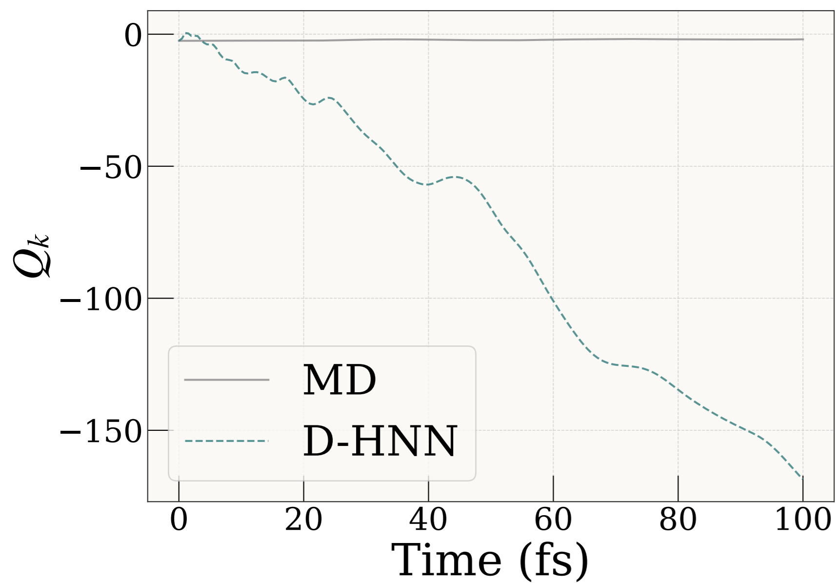
Mode 4 (415 \text{cm}^{-1} )
