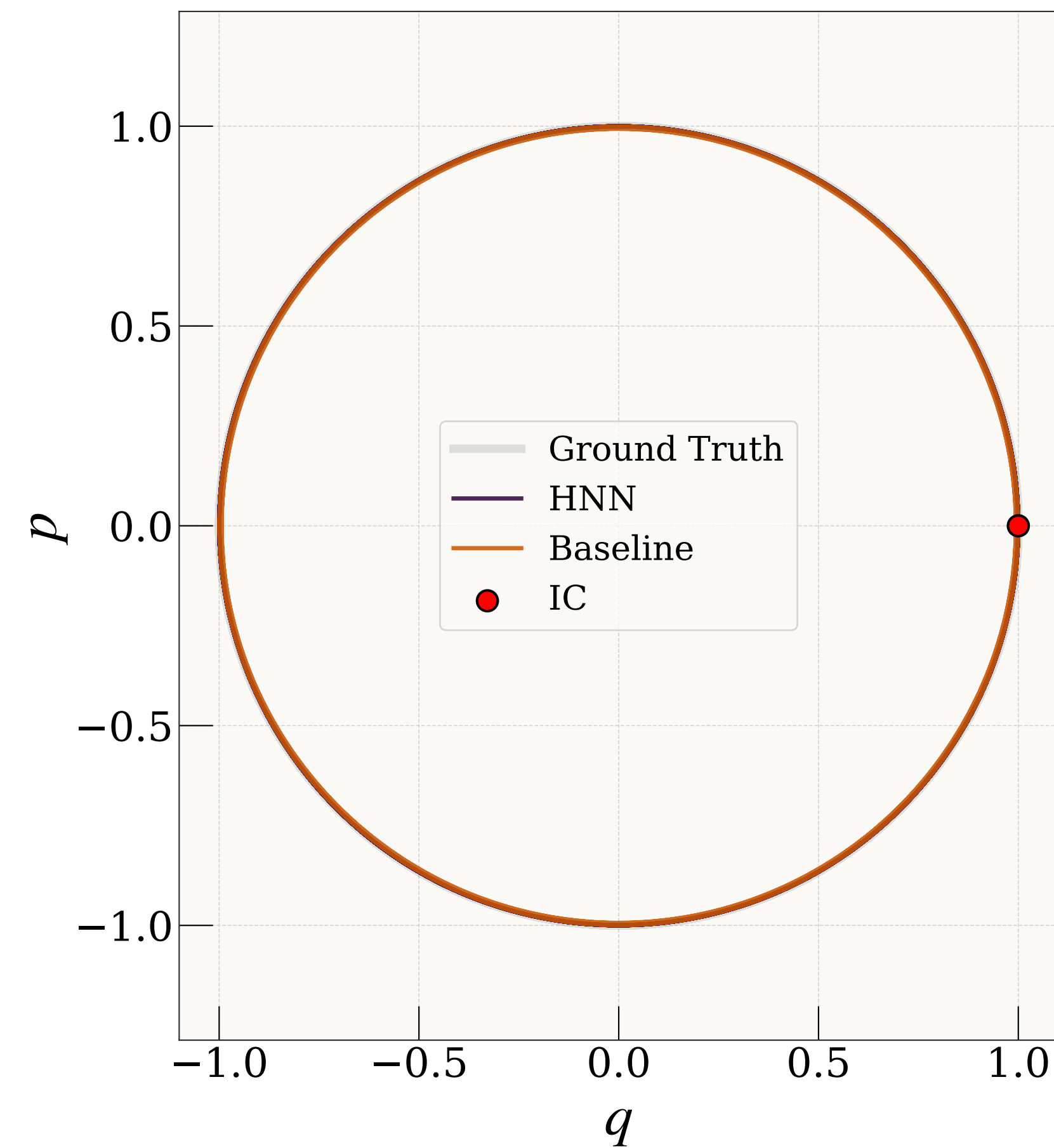
Phase Portrait ( T=100 )
