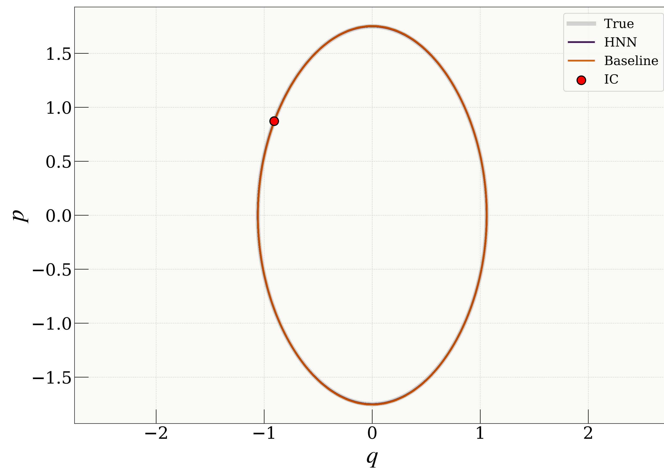
Phase Portrait
