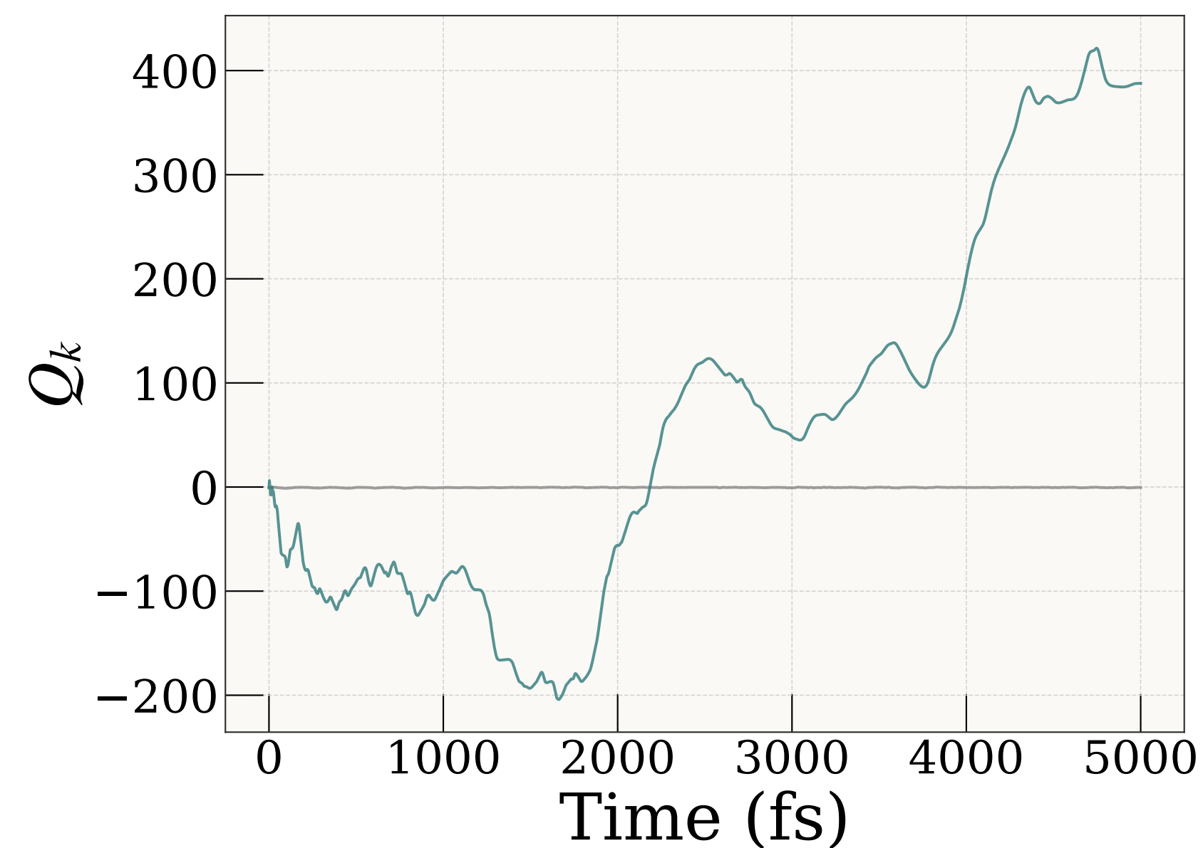
Mode 5 (441 \text{cm}^{-1} )
