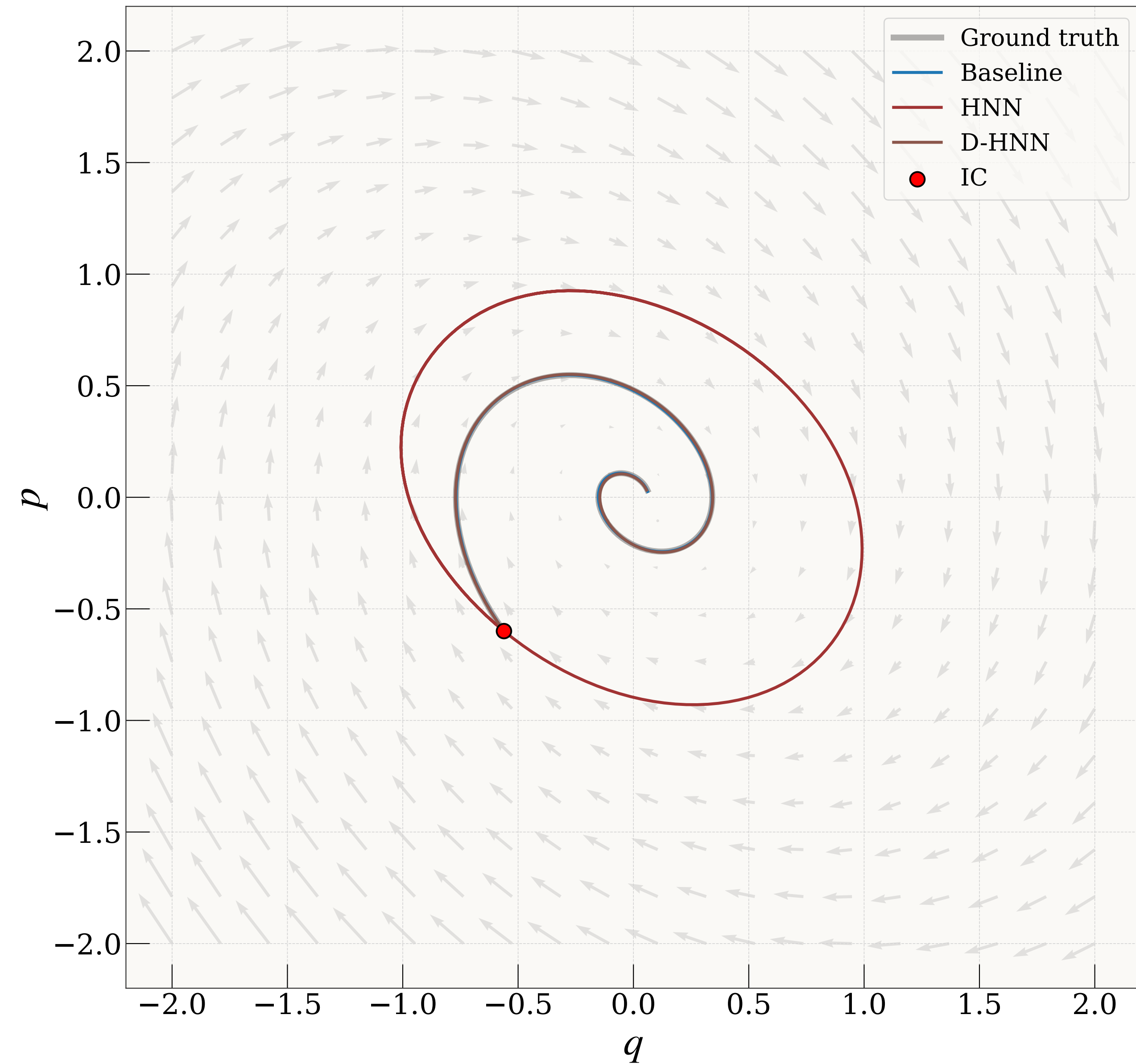
Damped Spring — Phase Portrait
