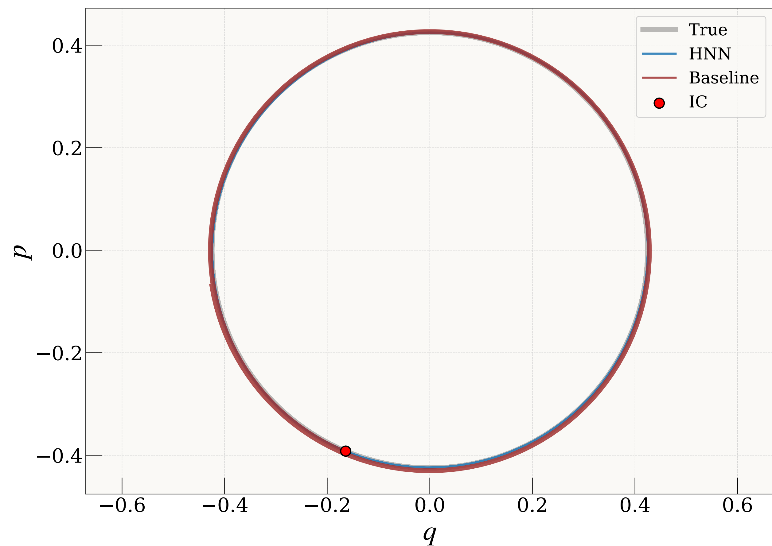
Phase Portrait
