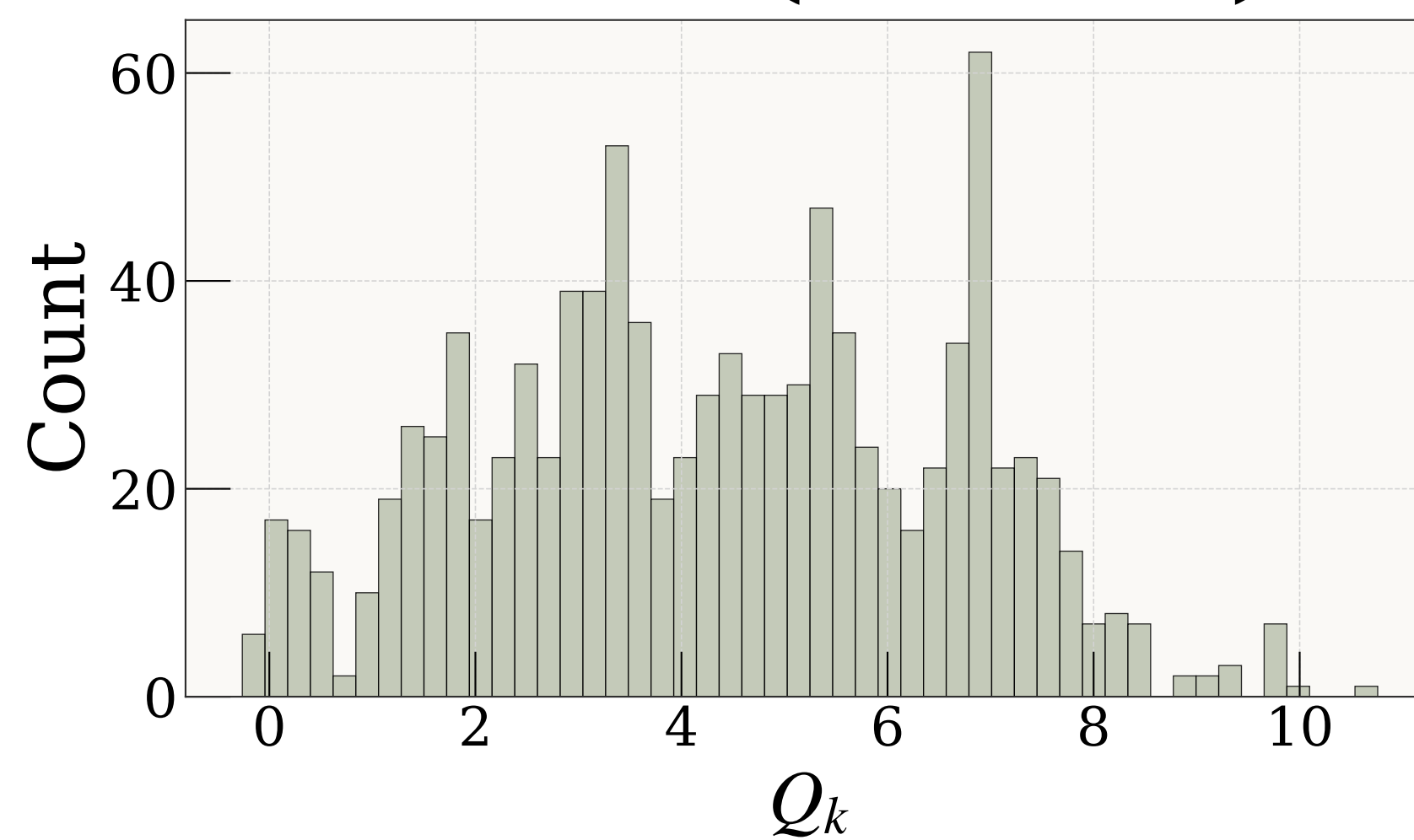
Mode 8 (880 cm -1 )
