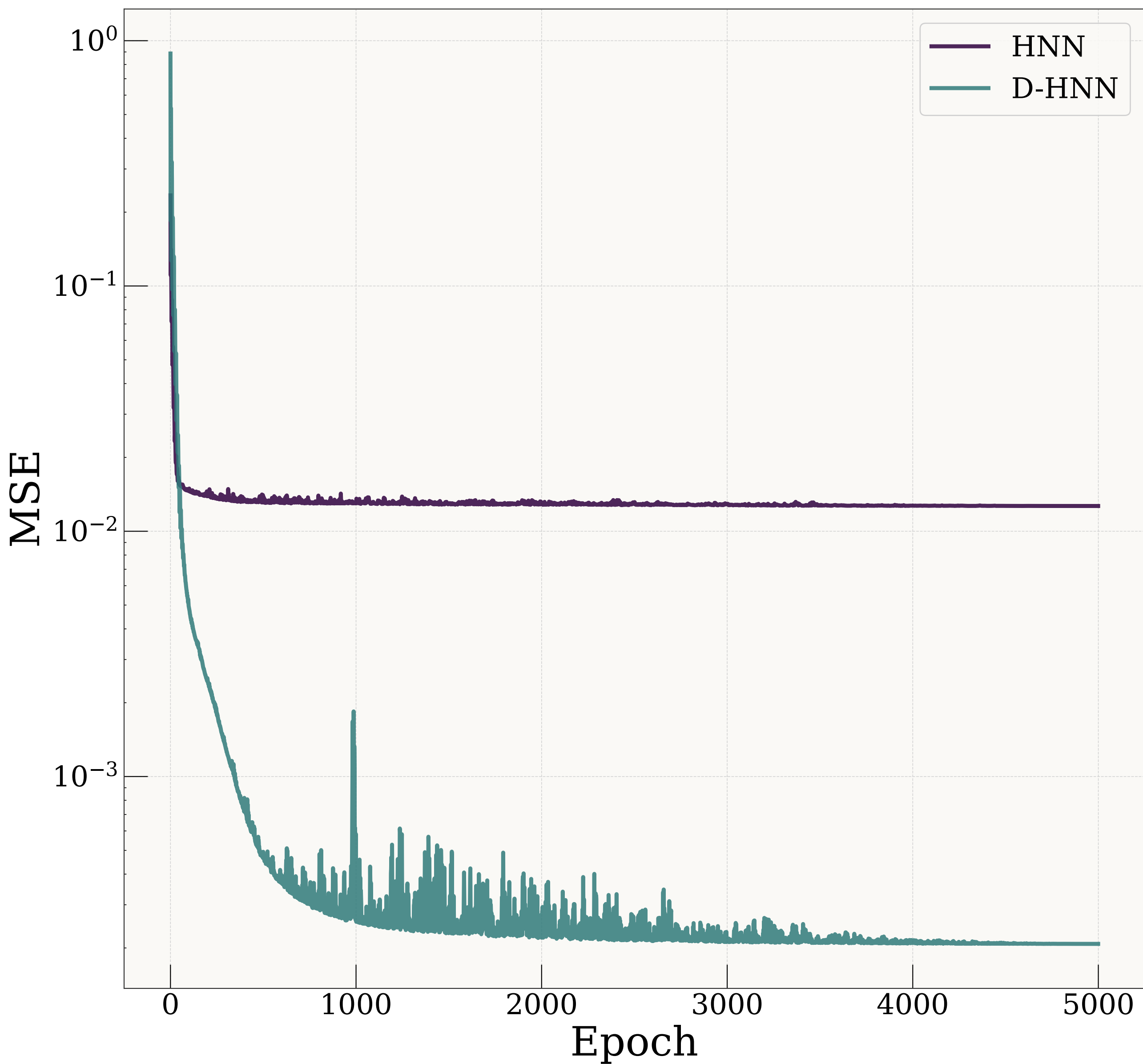
Train Loss
