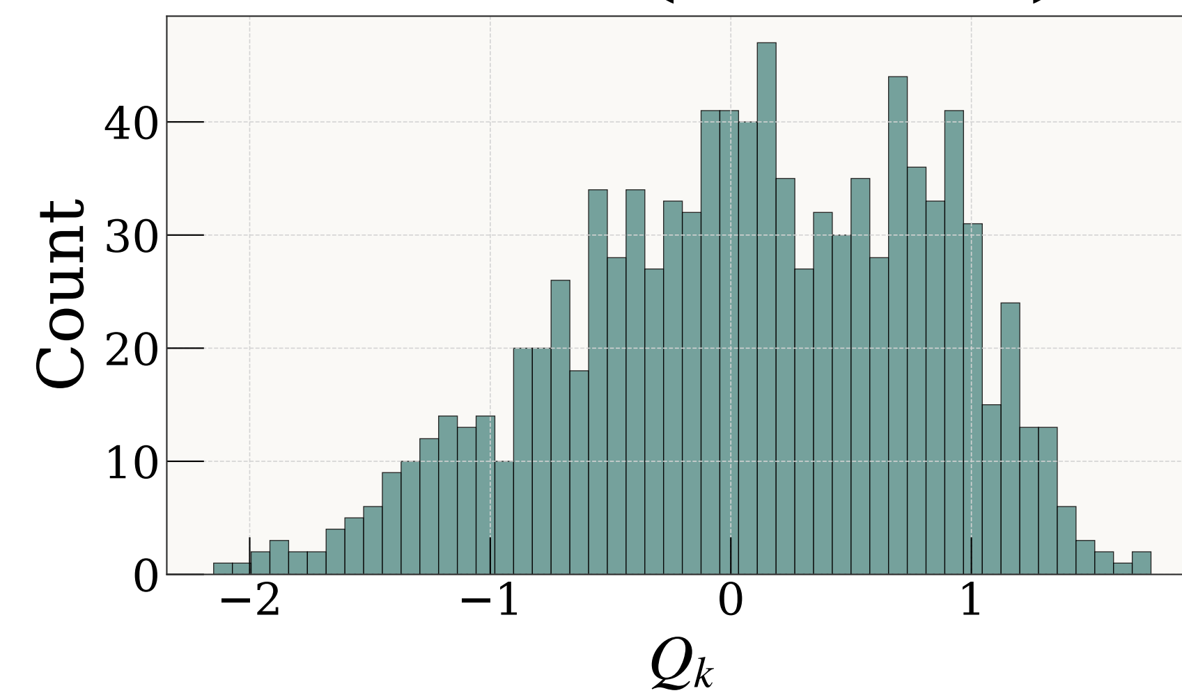
Mode 6 (510 \text{cm}^{-1} )
