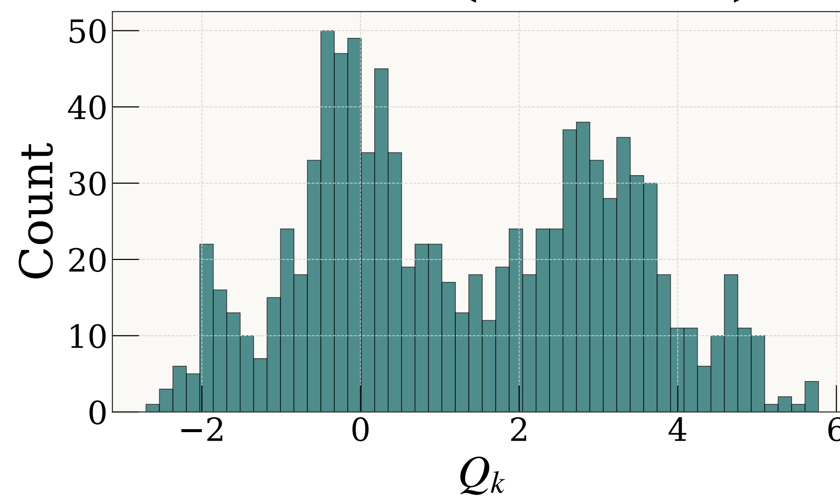
Mode 5 (441 \text{cm}^{-1} )
