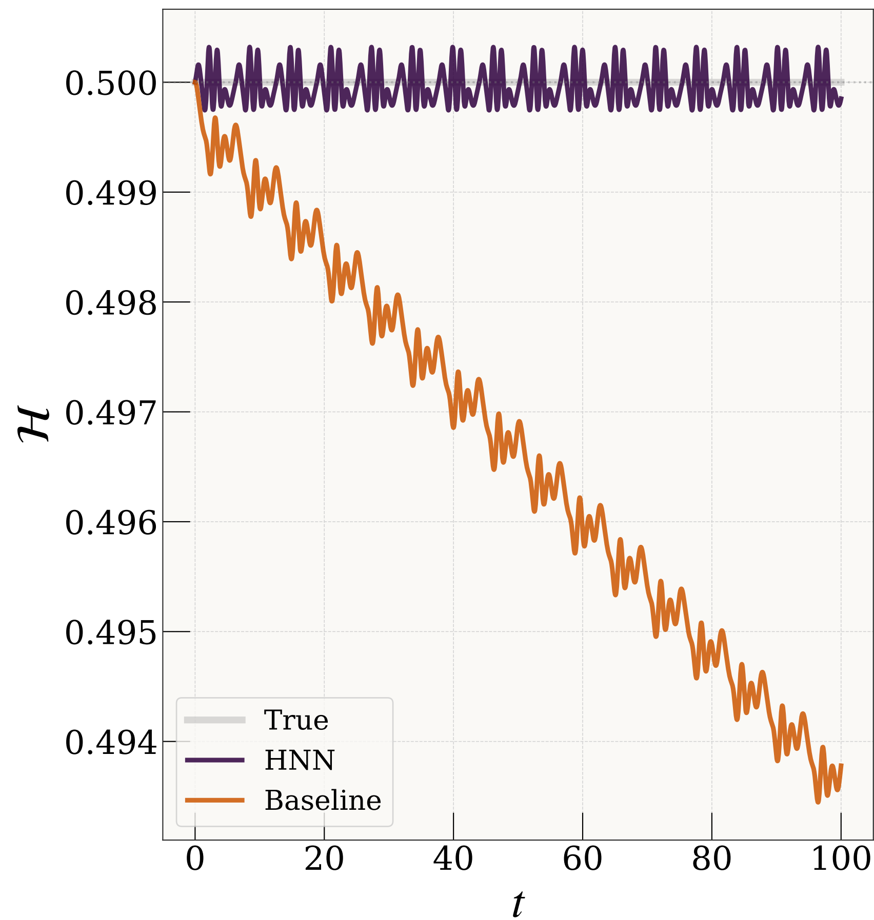
Energy Conservation
