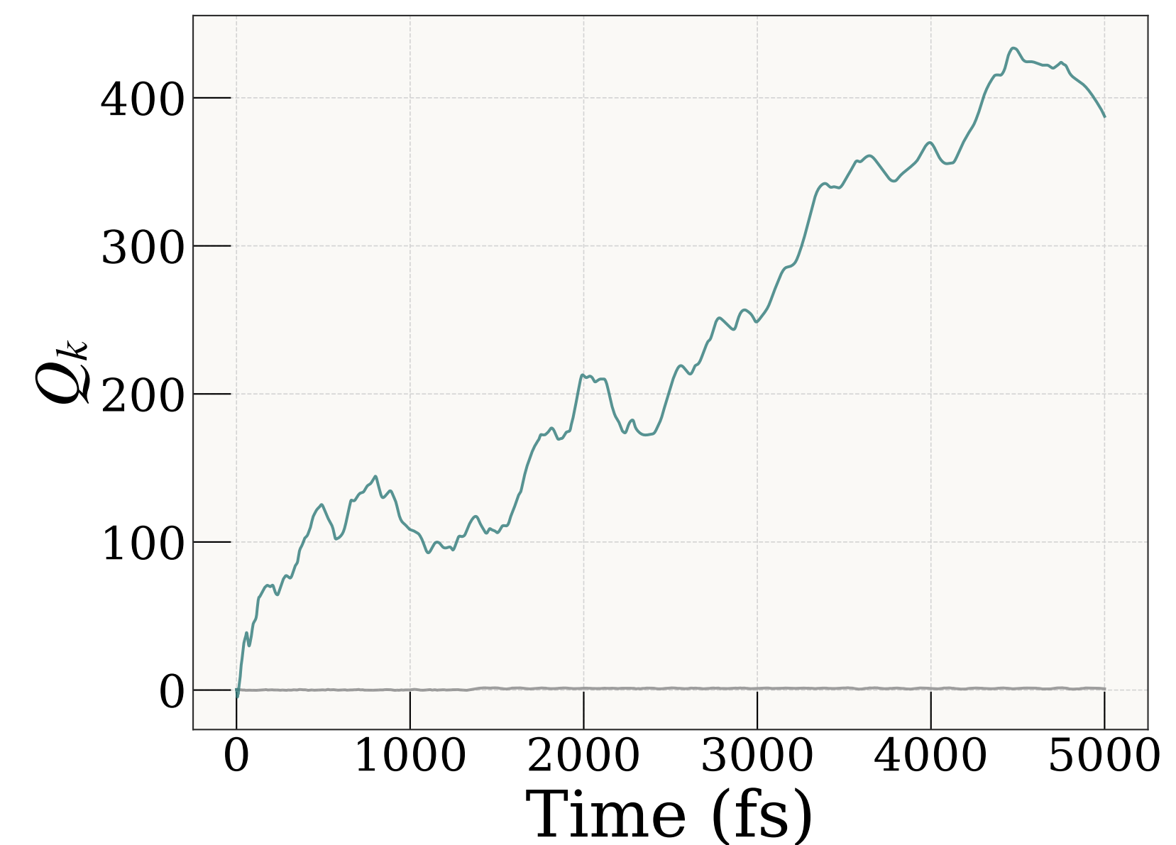
Mode 6 (510 \text{cm}^{-1} )
