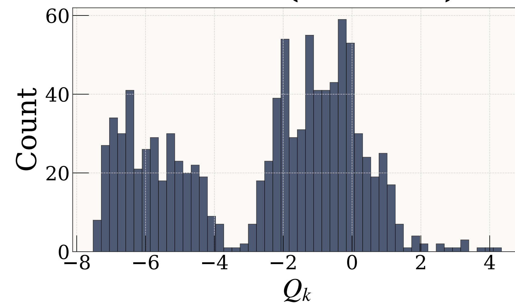
Mode 3 (-54 \text{cm}^{-1} )
