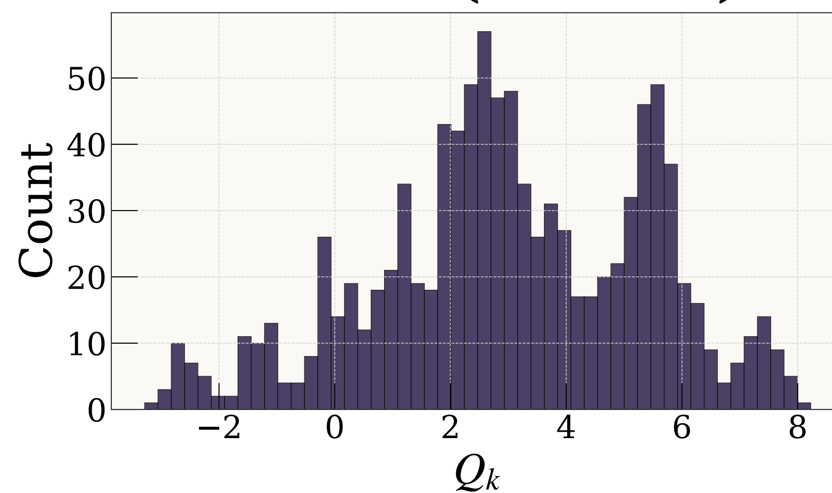
Mode 2 (-83 \text{cm}^{-1} )
