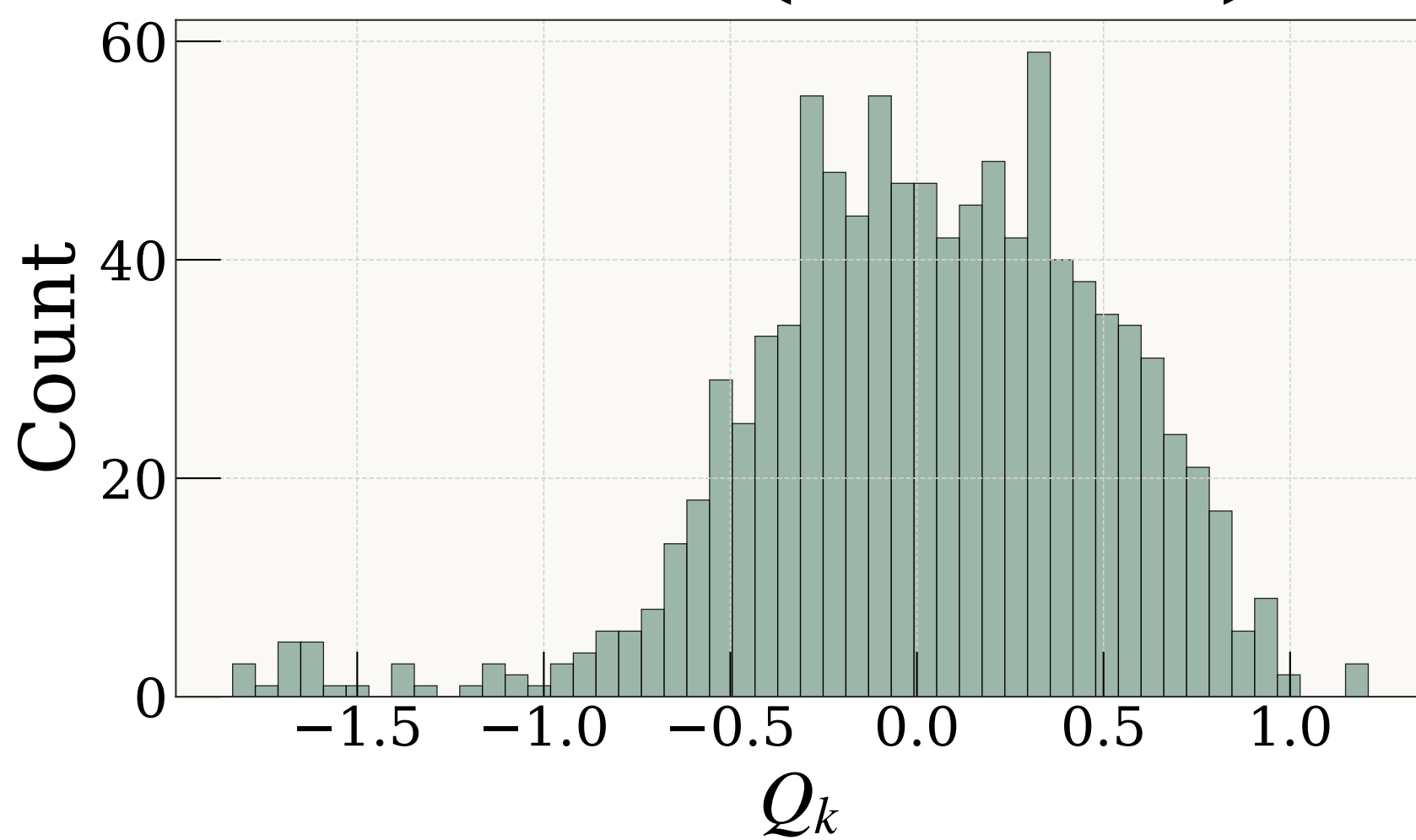
Mode 7 (759 cm -1 )
