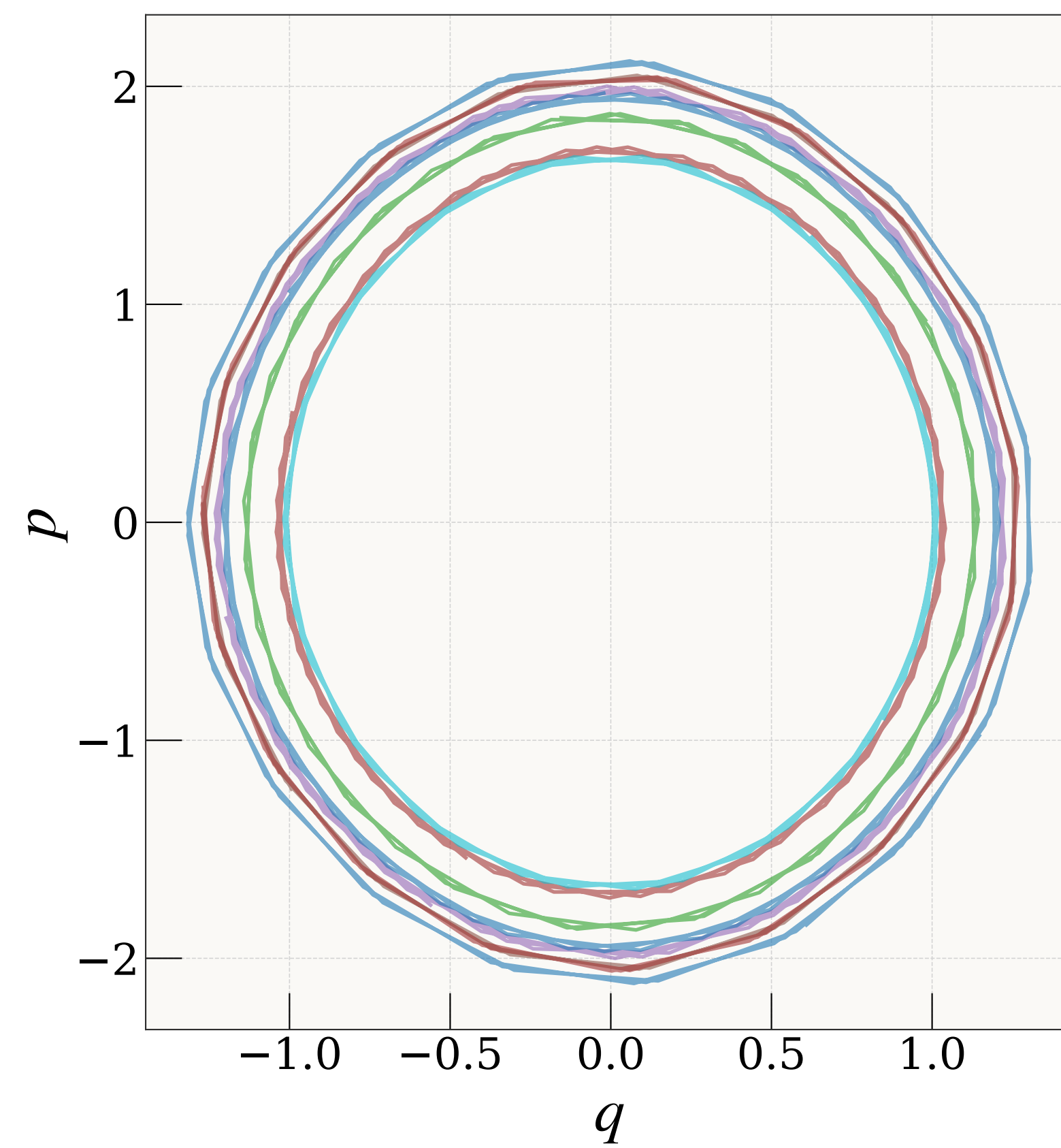
Pendulum — Phase Space
