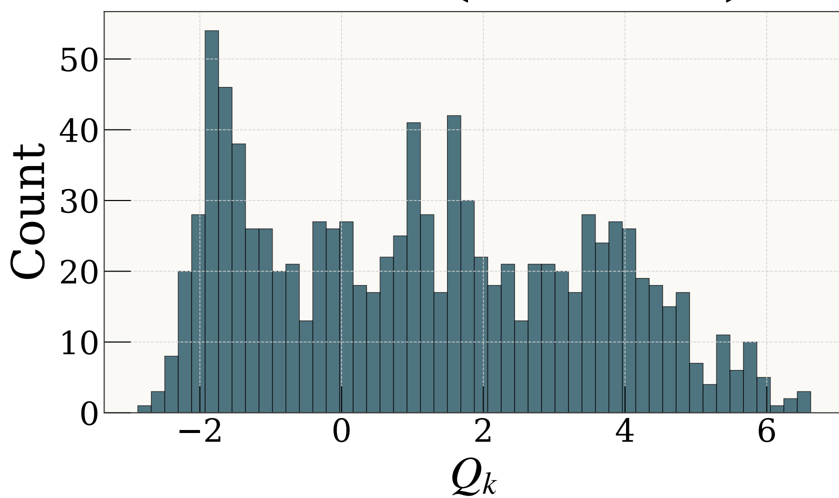
Mode 4 (415 \text{cm}^{-1} )
