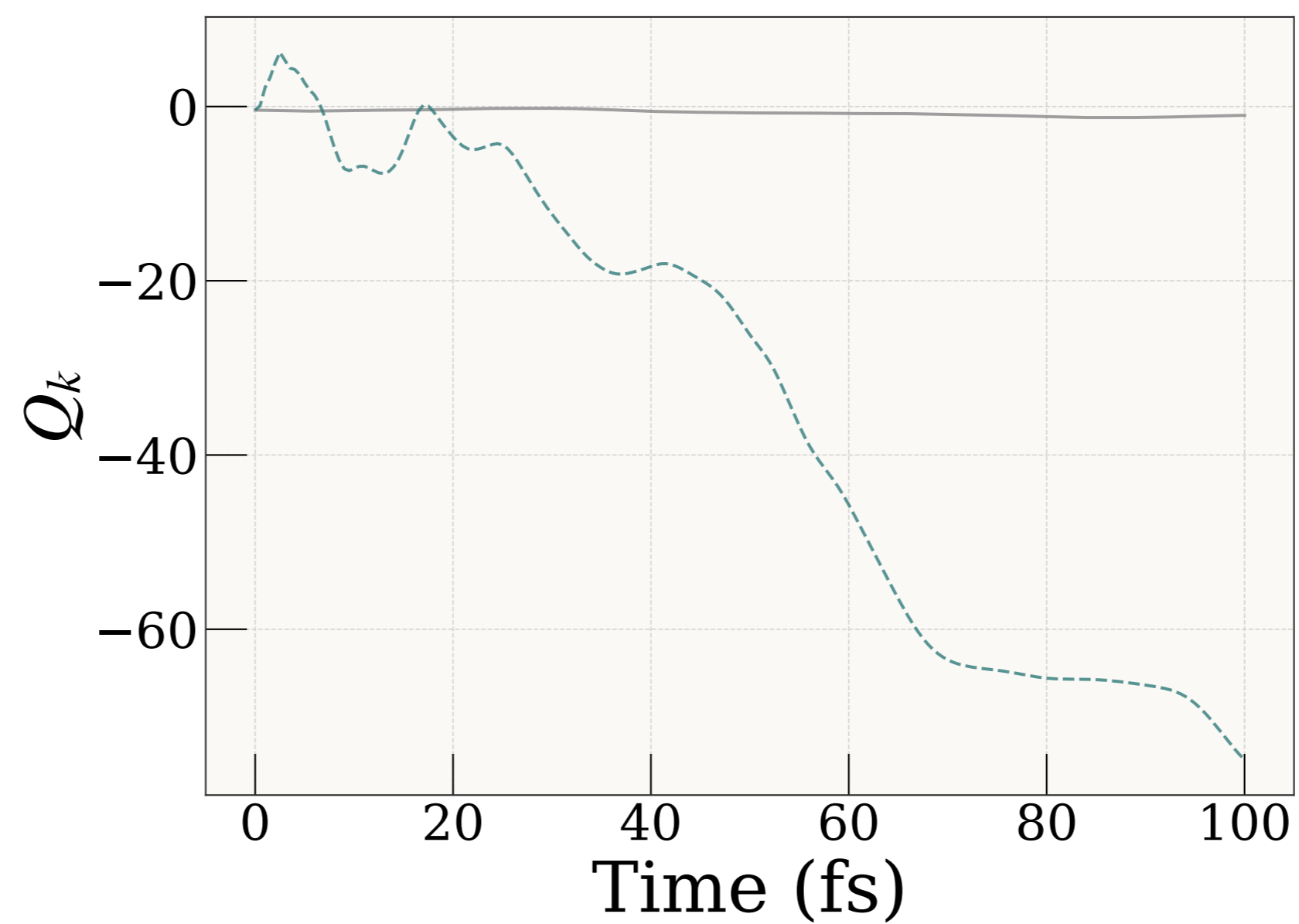
Mode 5 (441 \text{cm}^{-1} )
