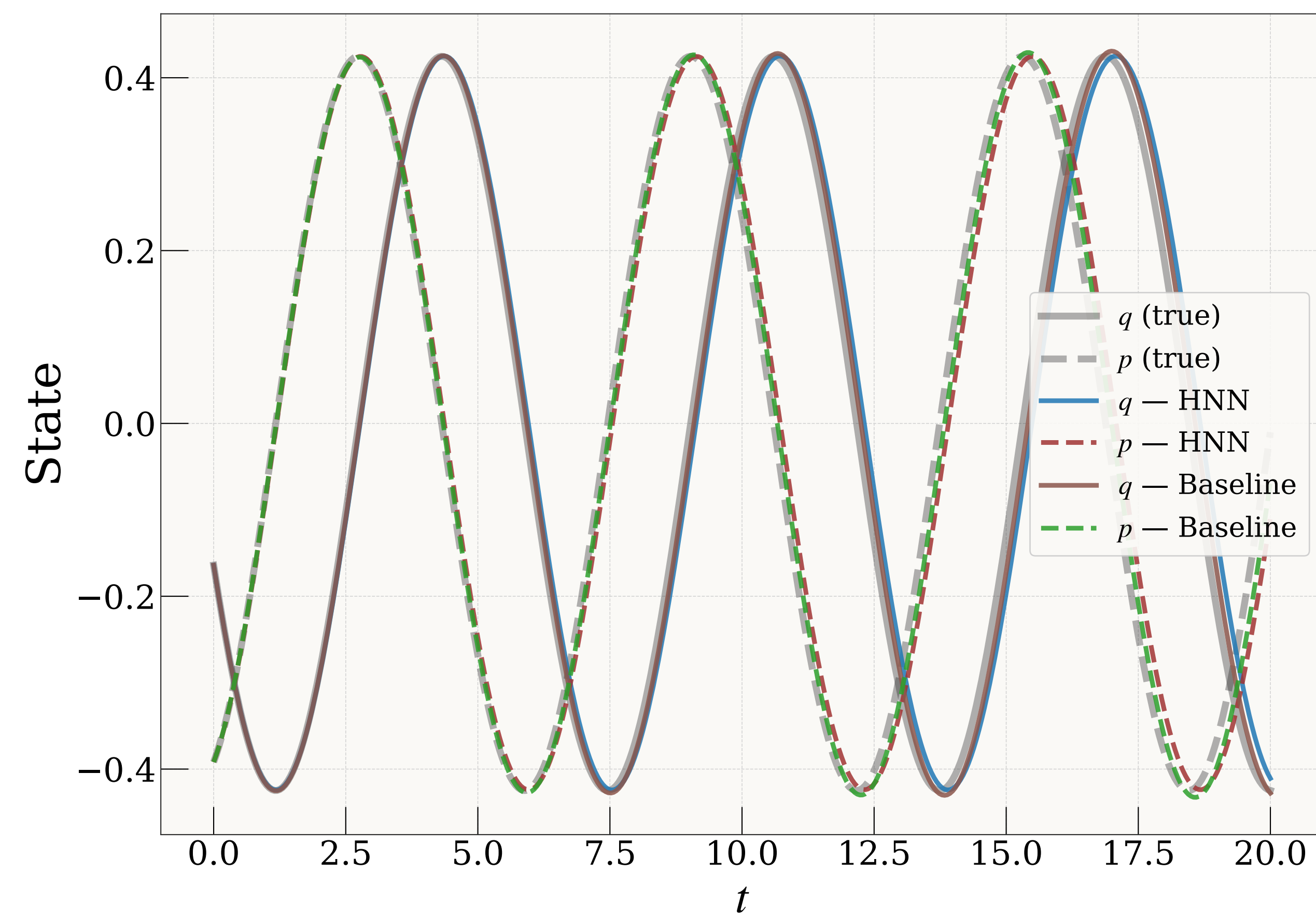
Time Series
