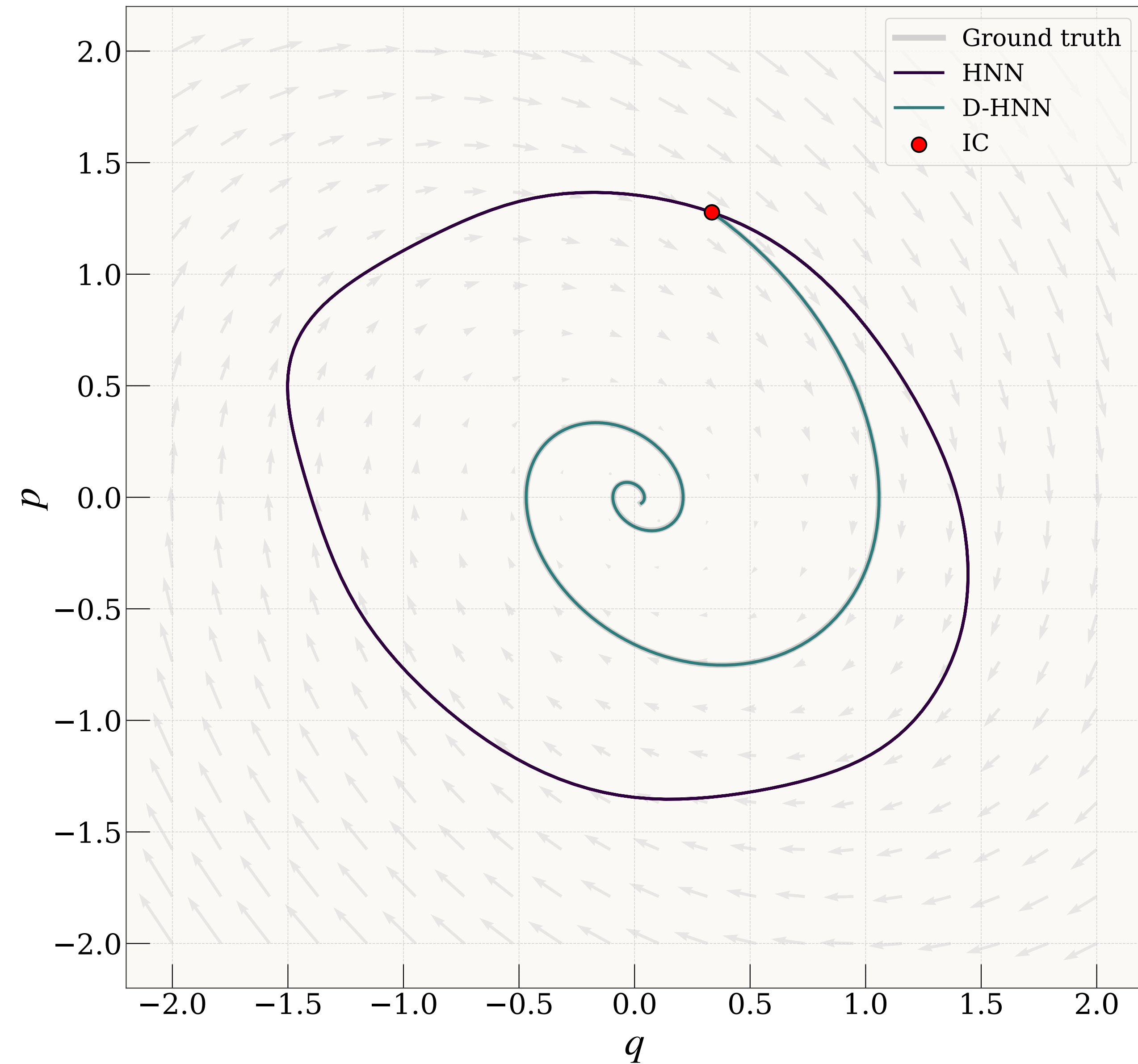
Damped Spring — Phase Portrait ( \rho=0.5 )
