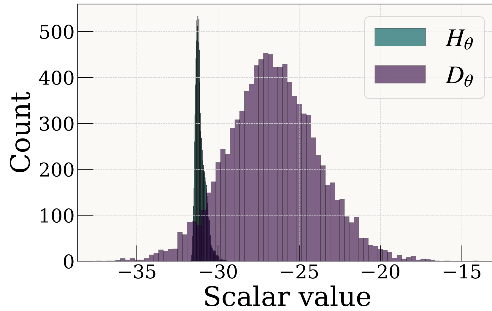
H_\theta and D_\theta Distributions
