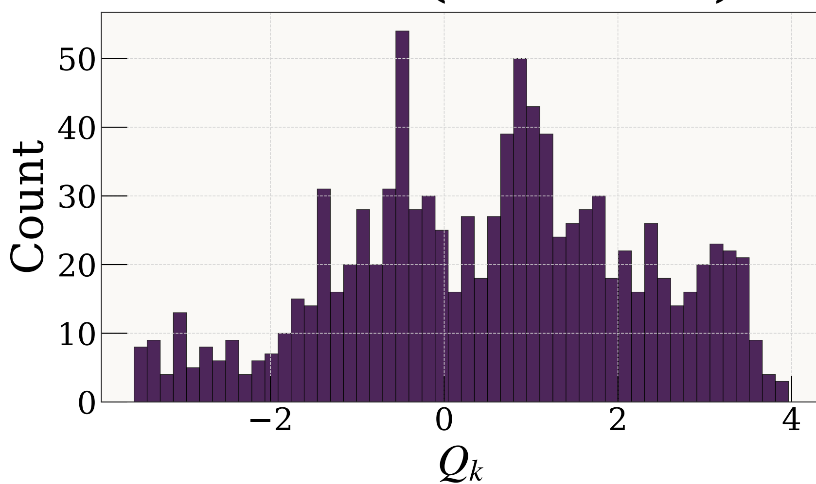
Mode 1 (-210 \text{cm}^{-1} )
