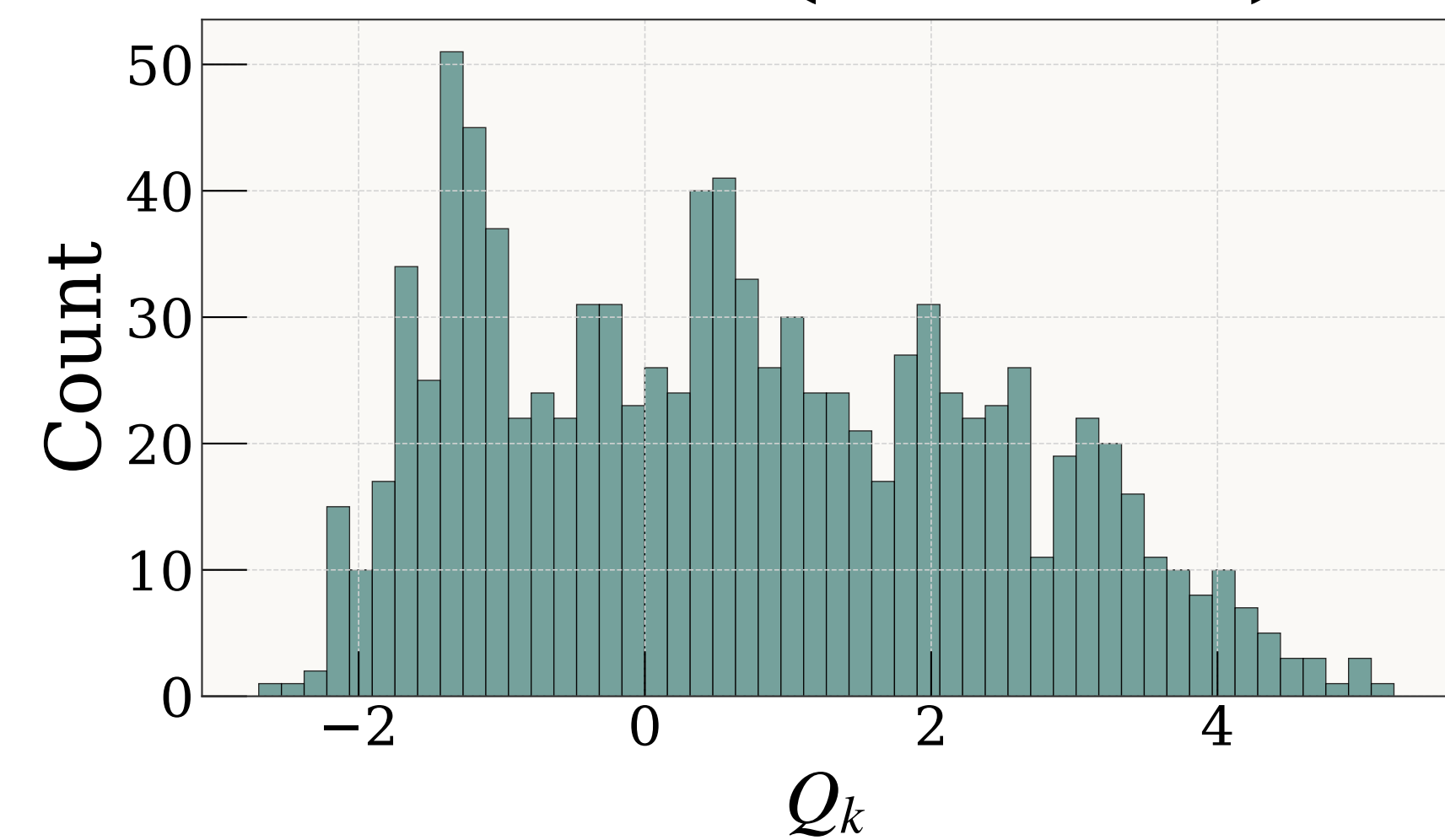
Mode 6 (493 cm -1 )
