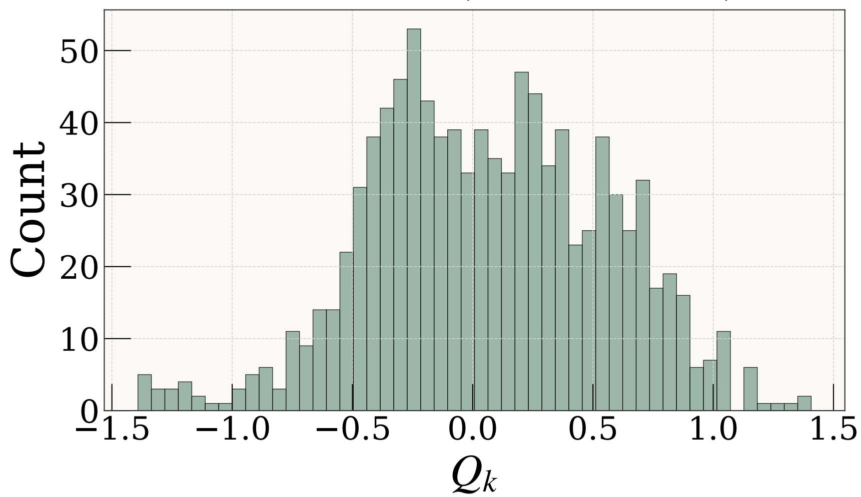
Mode 7 (779 \text{cm}^{-1} )
