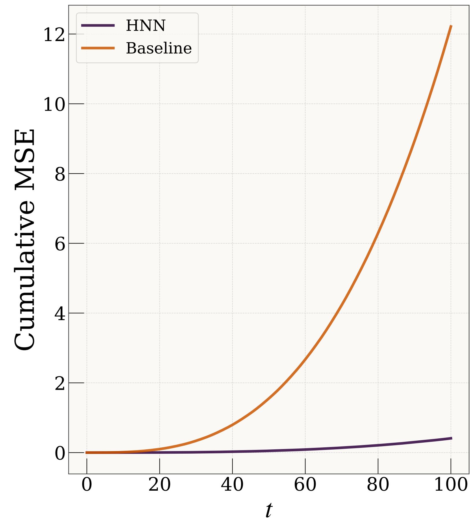
Error Accumulation
