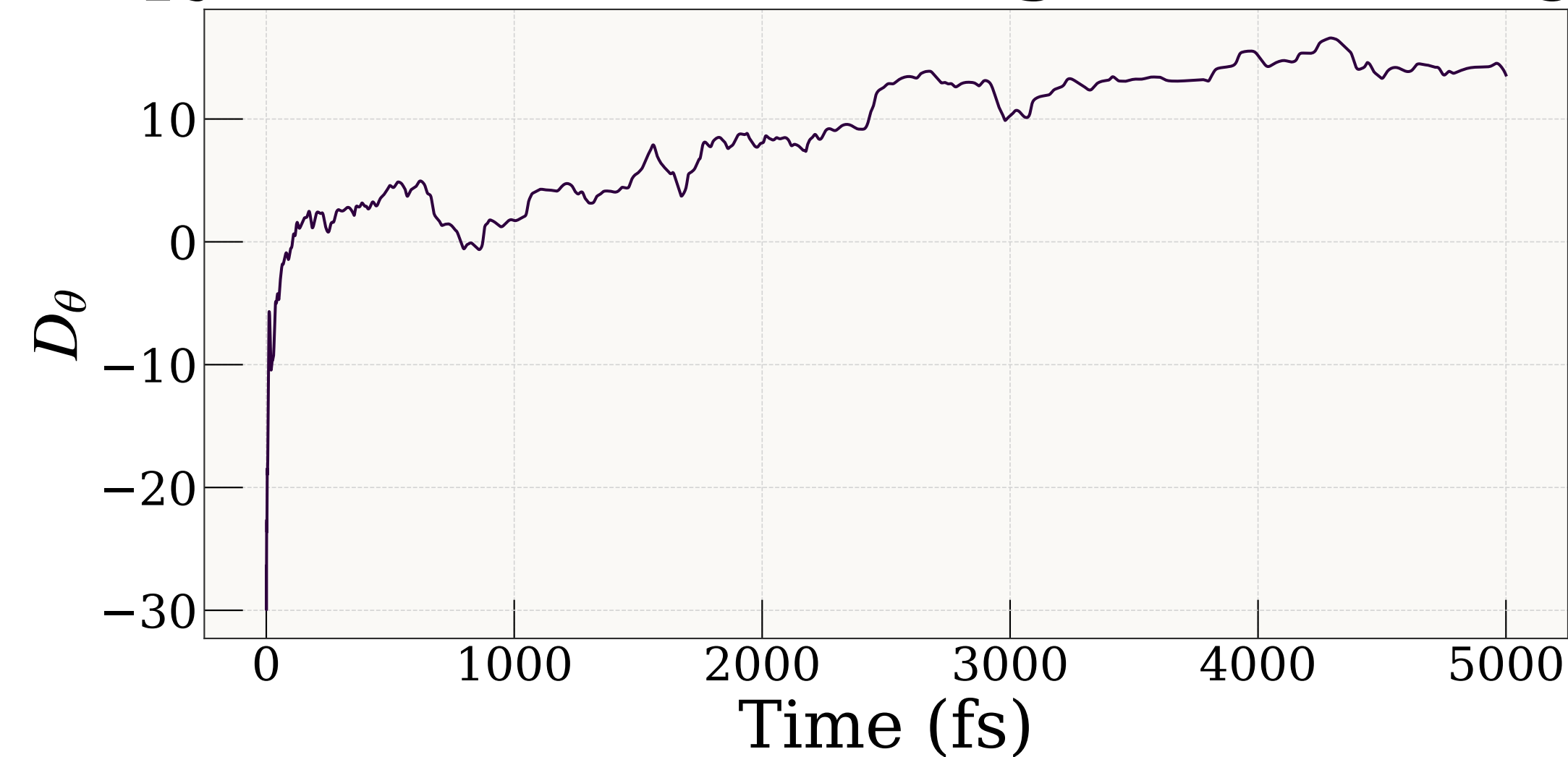
Learned Hamiltonian Along D-HNN Trajectory Dissipation Function Along D-HNN Trajectory
