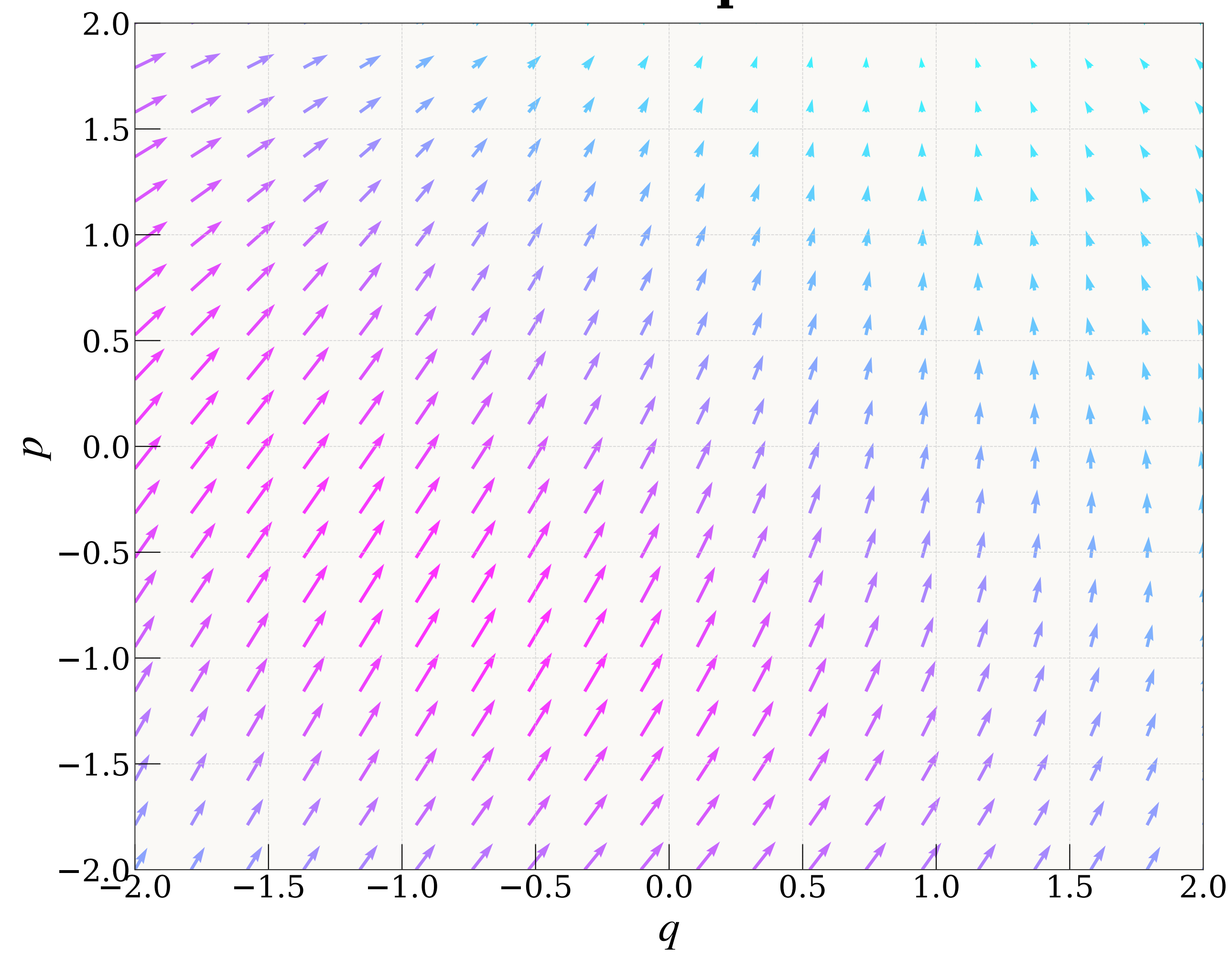
D-HNN Dissipative \nabla D
