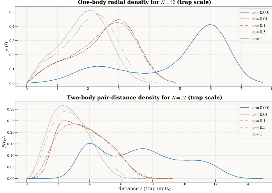
Figure 6.8: Twelve-electron radial densities P(r) across \omega .
