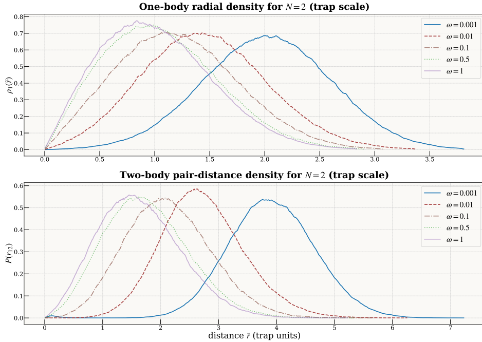
Figure 6.5: Two-electron radial densities P(r) across \omega .
