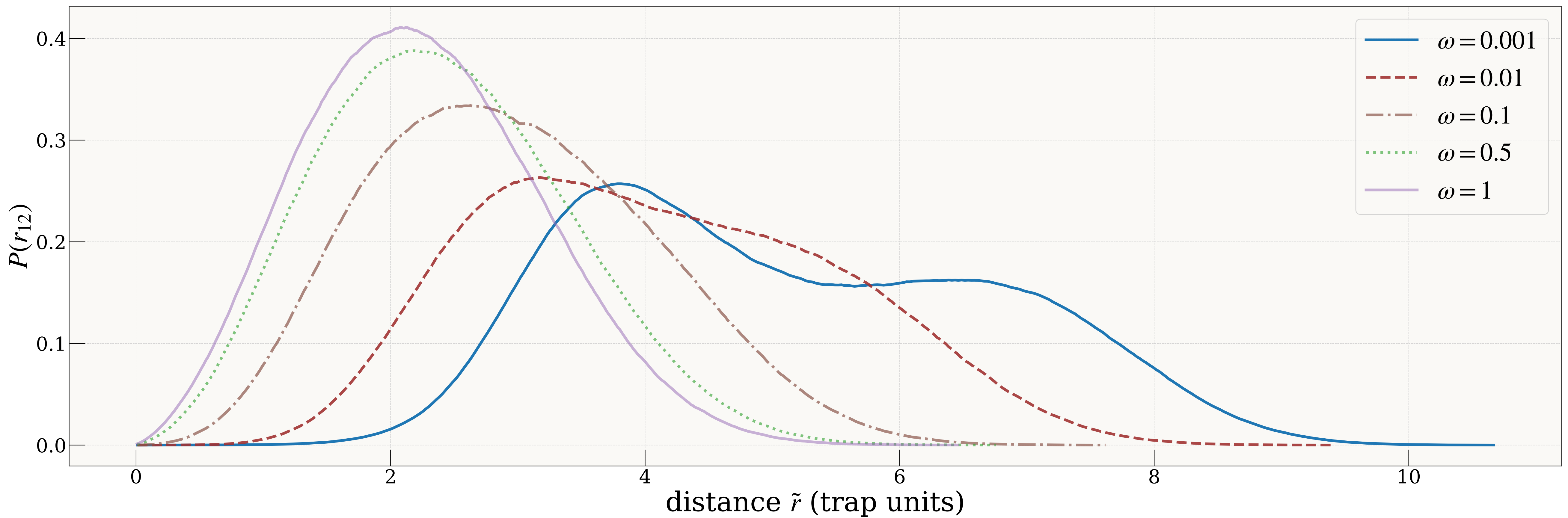
Two-body pair-distance density for N=6 (trap scale)
