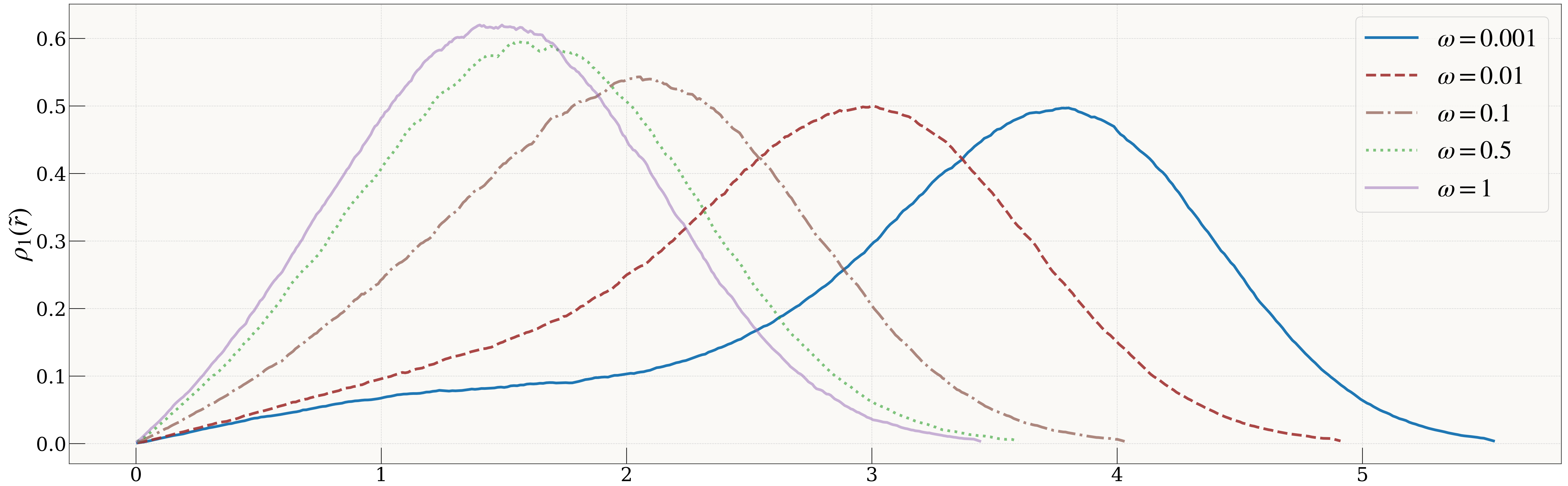
One-body radial density for N=6 (trap scale)
