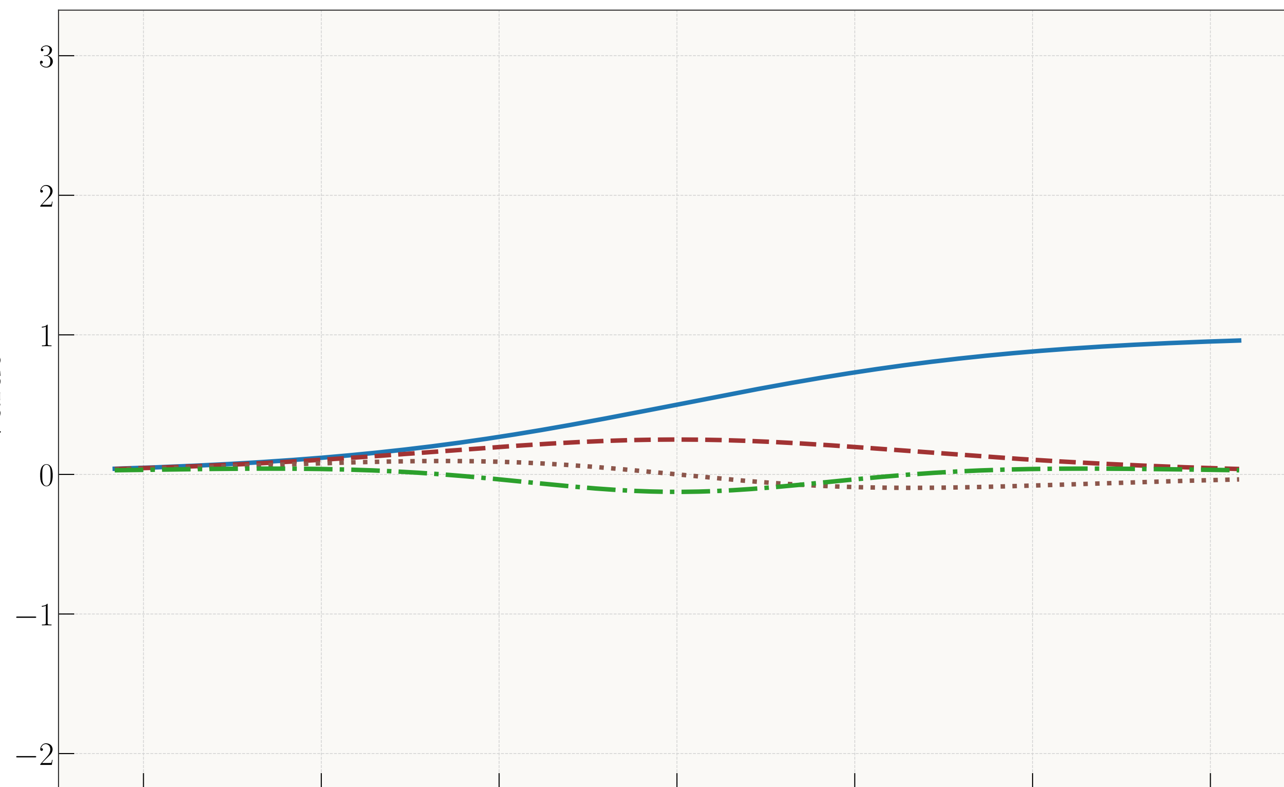
Mish
