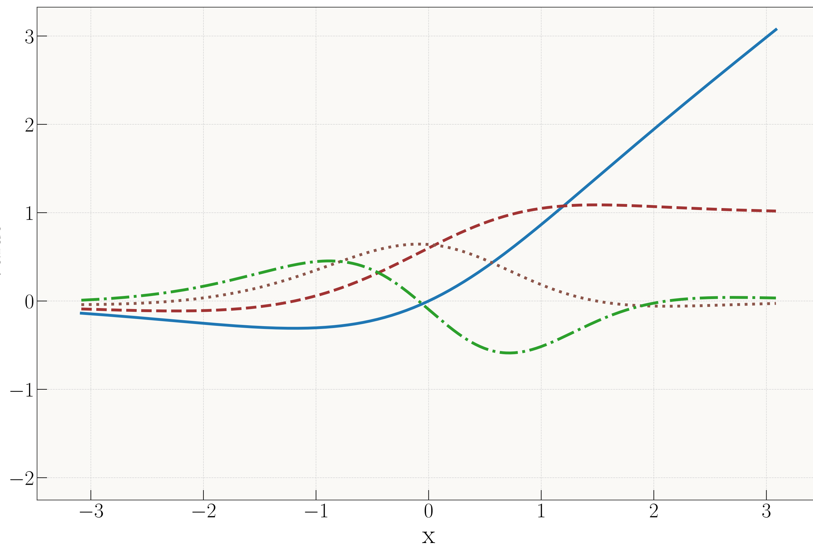
Mish
