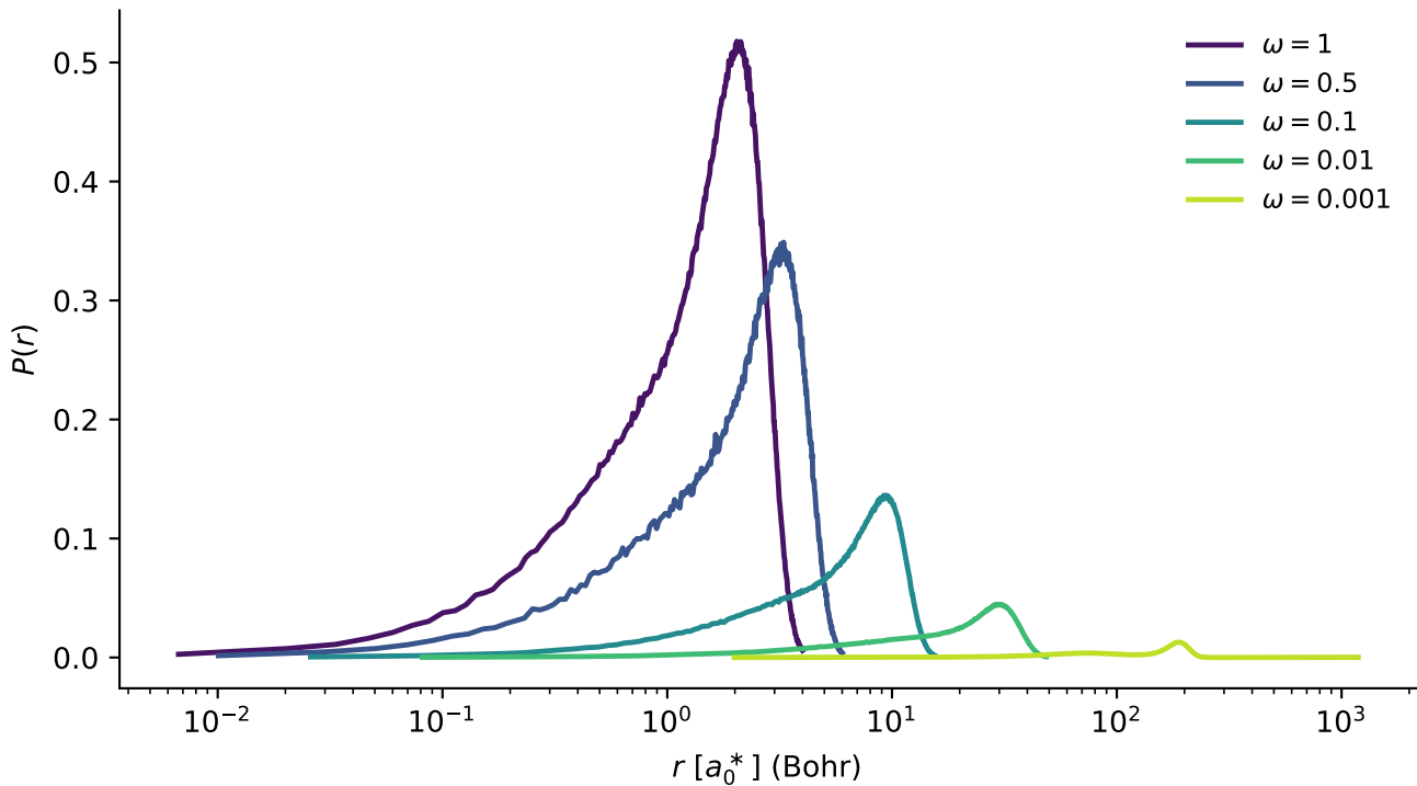
N = 12 : single-particle radial density across \omega
