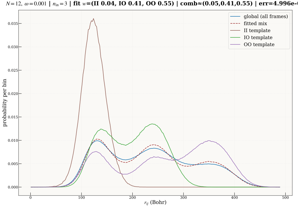
Figure 6.7: Shell-resolved reconstruction of g(r) at \omega = 10^{-3} for N=12 . The global pair distribution is reproduced by a convex mixture of inner–inner (II), inner–outer (IO) and outer–outer (OO) histograms with weights set by the observed (n_{\text{in}}, n_{\text{out}}) statistics.
