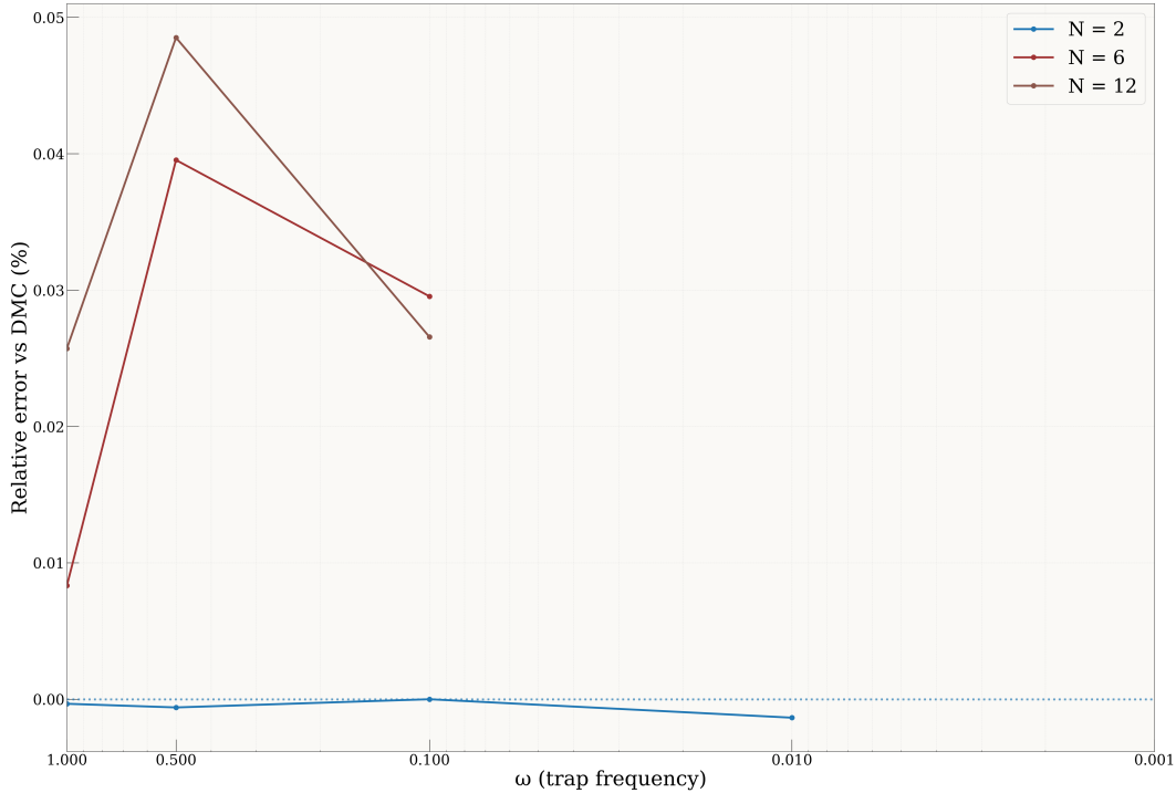
Figure 6.1: Relative deviation of the conv.-BF energies from the external references (Table 6.2) at every (N, \omega) where one exists: fixed-node DMC [52] for N=6 and 12 , and the compiled DMC and analytic [54] values for N=2 . Deviations are at the 10^{-3} % level for N=2 , comparable to the reference’s own precision, and 0.008 – 0.05 % for N=6 and 12 , with no trend in \omega .
