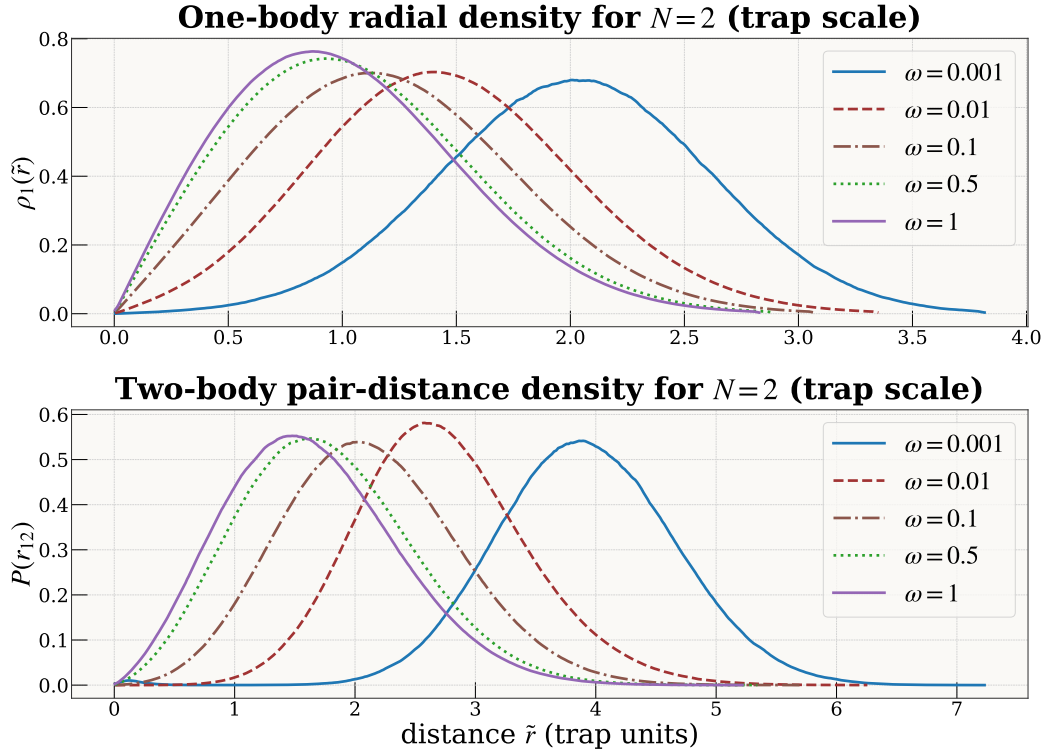
Figure 6.5: One-body radial density \rho_1(\tilde{r}) (top) and pair-distance density P(r_{12}) (bottom) for N=2 across \omega , in trap units \tilde{r} = \sqrt{\omega} r .
