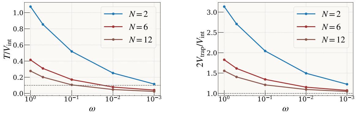
Figure 6.4: Energy-based Wigner diagnostics as functions of trap frequency. As \omega decreases the dots become interaction dominated ( T/V_{\text{int}} \ll 1 ) and the trap–interaction partition approaches the classical virial form, most clearly for N=12 .
