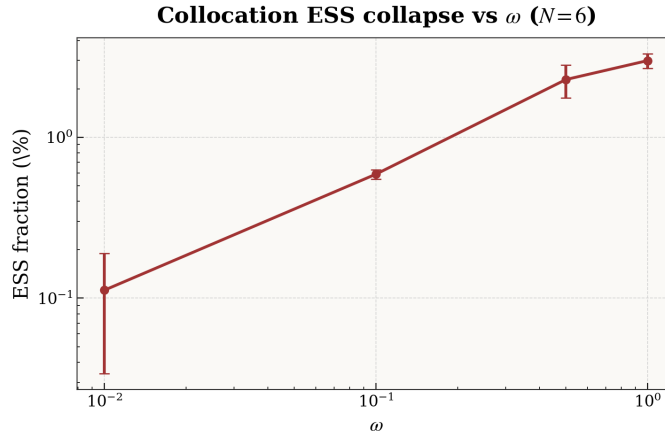
Figure 7.3: The naive collocation proposal collapses in the Wigner regime ( N=6 ). The effective sample size (as a percentage of the batch) falls by more than an order of magnitude from \omega=1 to \omega=0.01 , where it reaches \sim 0.1\% —about five usable points in a batch of 4096. This is a property of the sampling measure, not of optimisation, and it is what the physics-informed ring proposal (§7.4) is designed to repair.
