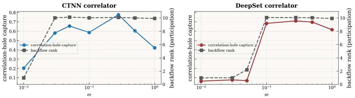
Figure 7.5: Correlator physicality and backflow rank collapse together ( N=6 ; the backflow architecture is held fixed, only the correlator changes). For each correlator, the correlation-hole capture (left axis) and the backflow displacement rank (right axis) give way at the same \omega : \omega \approx 0.05 for the DeepSet, \omega \approx 0.01 for the CTNN. A correlator that keeps its physical structure lets the backflow keep its rank.
