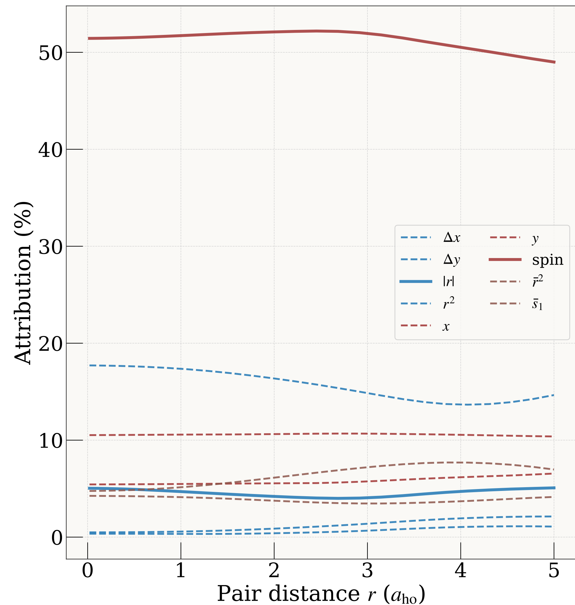
Per-channel attribution vs pair distance (REINFORCE, \omega=0.1 ) — unsafe channels \Delta \mathbf{x} , \Delta \mathbf{y} suppressed globally
