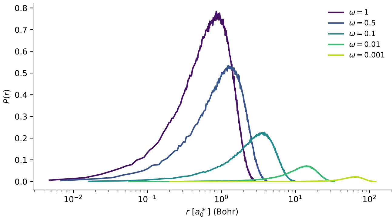
N = 2 : single-particle radial density across \omega
