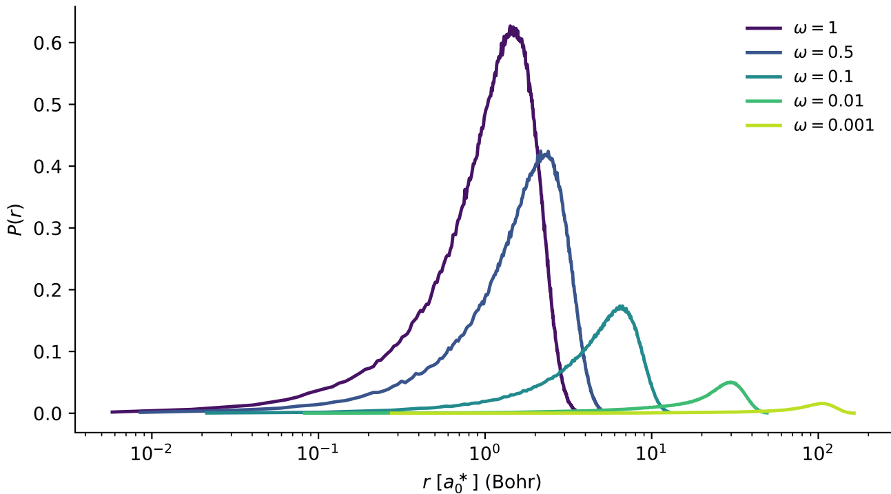
N = 6 : single-particle radial density across \omega
