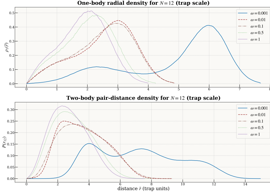
Figure 6.8: Twelve-electron radial densities P(r) across \omega .
