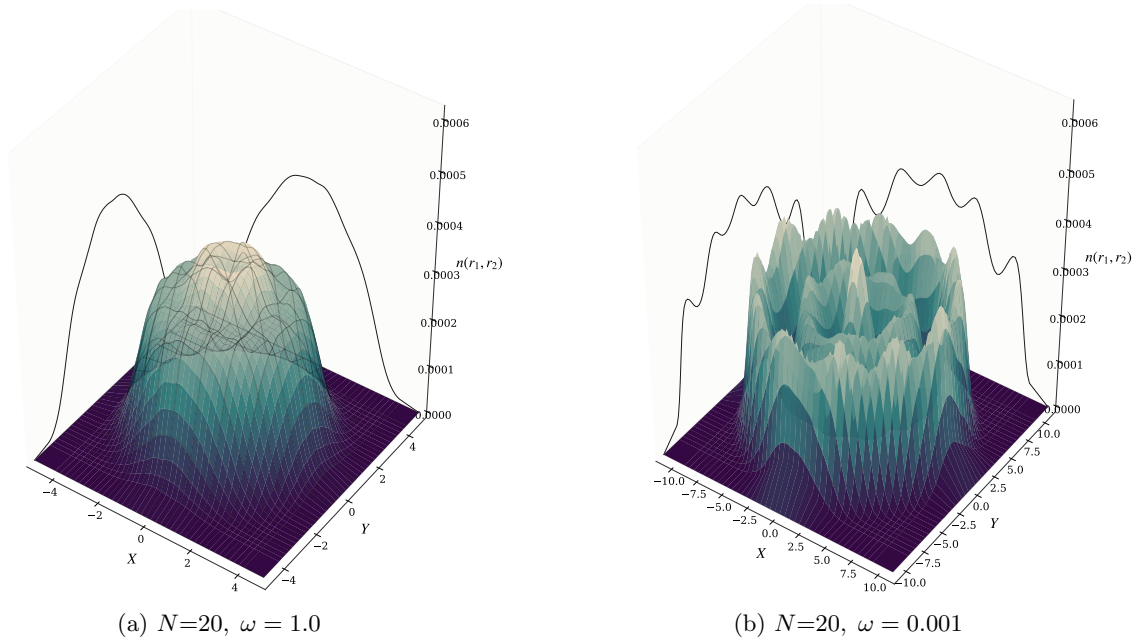
Figure 6.3: One-body densities for N=20 at strong and weak confinement. The weak-trap case shows strong radial broadening and clear multi-shell organization, consistent with deep Wigner-molecule ordering.
