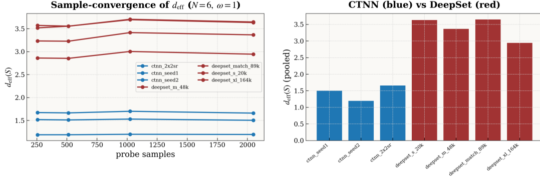
Figure 7.1: Message passing compresses the correlator (Q1a, N=6 , \omega=1 ). Left : the effective rank of the quantum geometric tensor on a common pooled probe, converged in the number of probe samples. Right : the same pooled measure per model. The CTNN (blue) reaches the ground state in d_{\text{eff}} \approx 1.2 – 1.7 , while every DeepSet (red) needs \approx 2.9 – 3.6 —and the gap does not close as the DeepSet is scaled from 20k to 164k parameters. The compression is architectural, not a matter of capacity.
