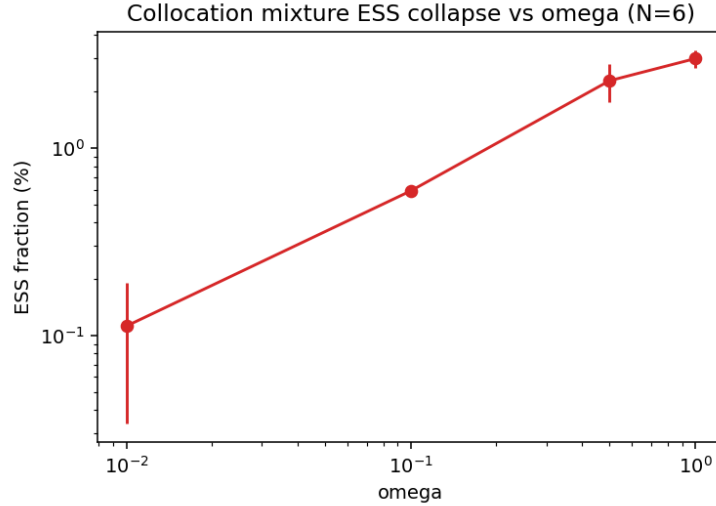
Figure 7.4: The naive collocation proposal collapses in the Wigner regime ( N=6 ). The effective sample size (as a percentage of the batch) falls by more than an order of magnitude from \omega=1 to \omega=0.01 , where it reaches \sim 0.1\% —about five usable points in a batch of 4096. This is a property of the sampling measure, not of optimisation, and it is what the physics-informed ring proposal (§7.4) is designed to repair.
