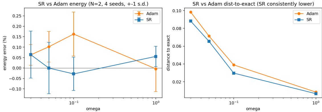
Figure 7.3: Under |\Psi|^2 sampling, SR and Adam are statistically indistinguishable ( N=2 , 4 seeds, \pm 1 s.d.). Left : relative energy error—the two optimisers overlap within error bars at every \omega . Right : distance to the exact state, where SR is consistently but marginally lower. The whitening SR performs is redundant here because the VMC metric is already well conditioned; its decisive advantage appears only for the ill-conditioned weak-form collocation objective.
