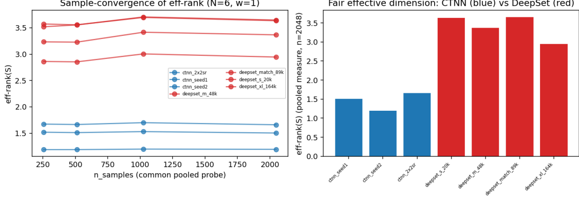
Figure 7.1: Message passing compresses the correlator (Q1a, N=6 , \omega=1 ). Left : the effective rank of the quantum geometric tensor on a common pooled probe, converged in the number of probe samples. Right : the same pooled measure per model. The CTNN (blue) reaches the ground state in d_{\text{eff}} \approx 1.2\text{--}1.7 , while every DeepSet (red) needs \approx 2.9\text{--}3.6 —and the gap does not close as the DeepSet is scaled from 20k to 164k parameters. The compression is architectural, not a matter of capacity.
