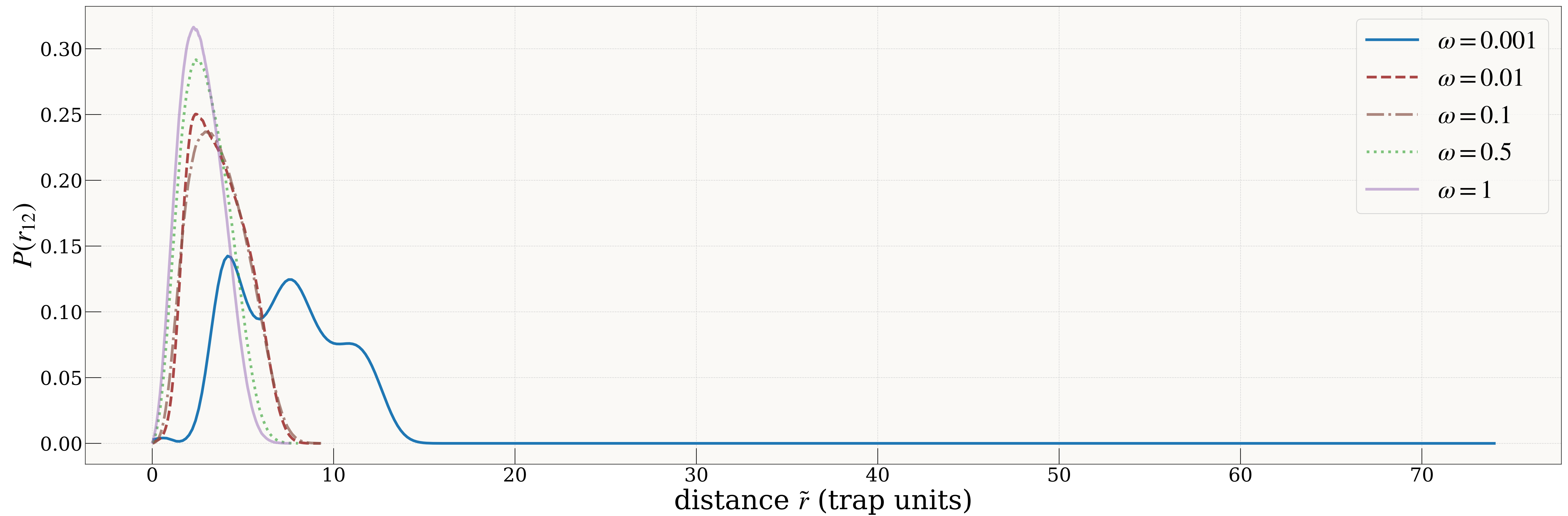
Two-body pair-distance density for N=12 (trap scale)
