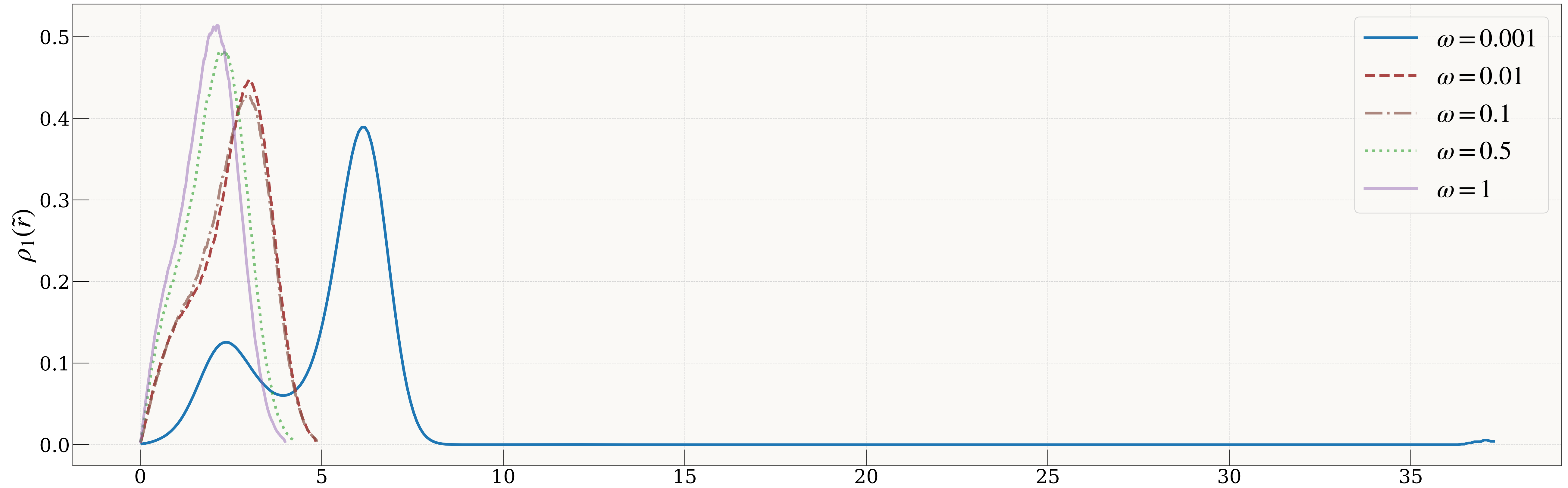
One-body radial density for N=12 (trap scale)
