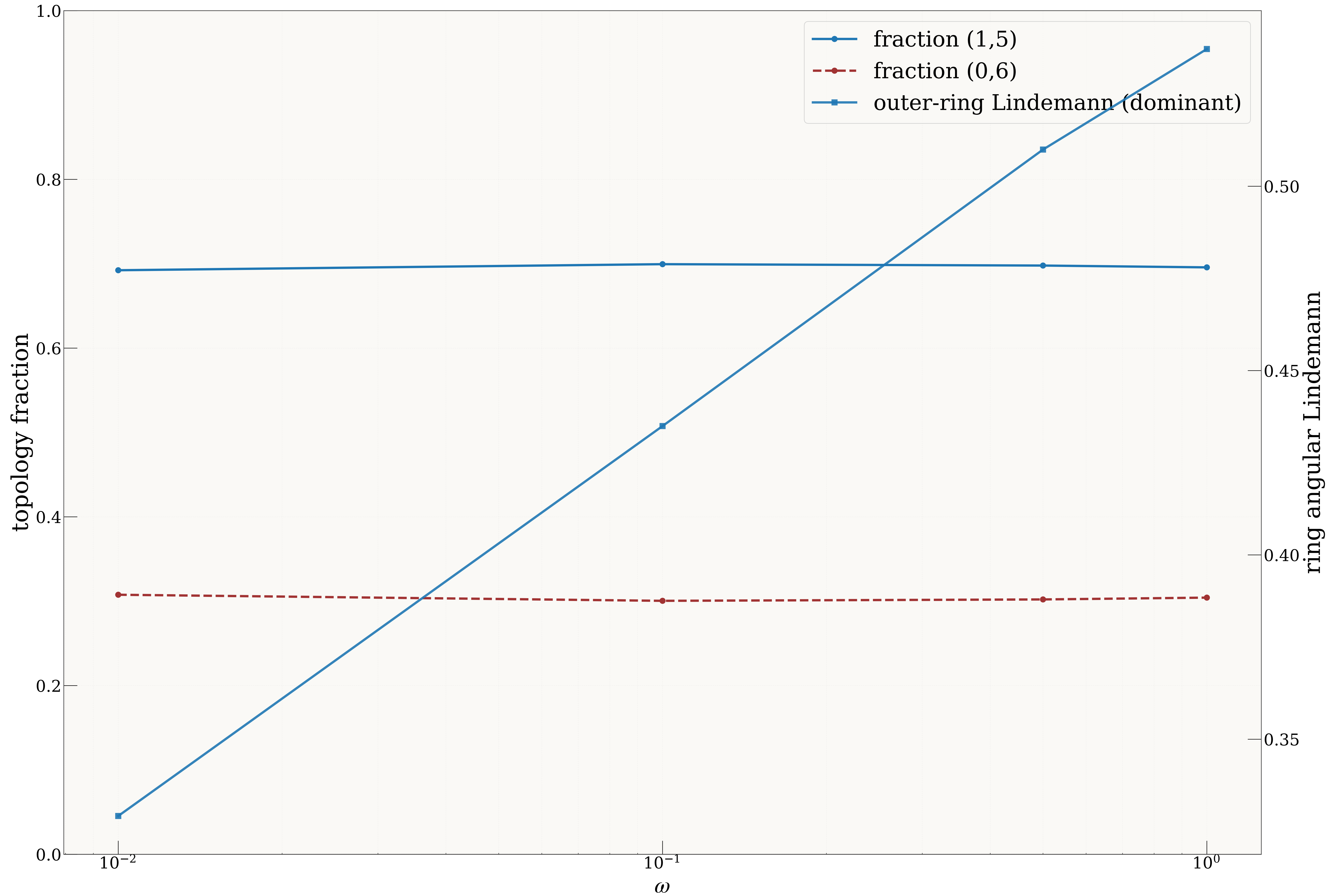
N=6: topology fractions and ring stiffness vs \omega
