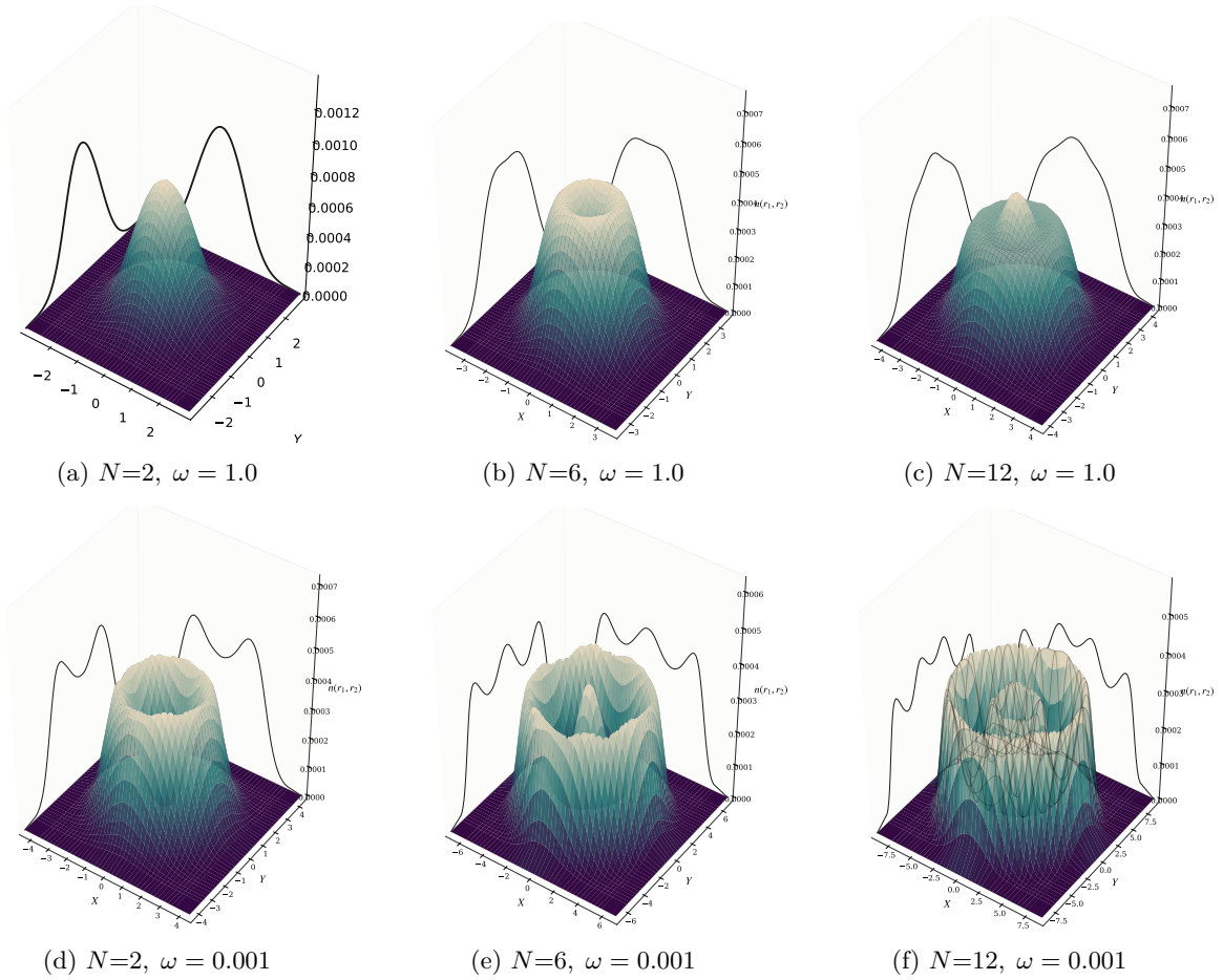
Figure 6.2: One-body densities for N = 2, 6, 12 at \omega = 1.0 (top) and \omega = 0.001 (bottom). As confinement weakens, the densities broaden and develop pronounced shell structures characteristic of Wigner molecules.
