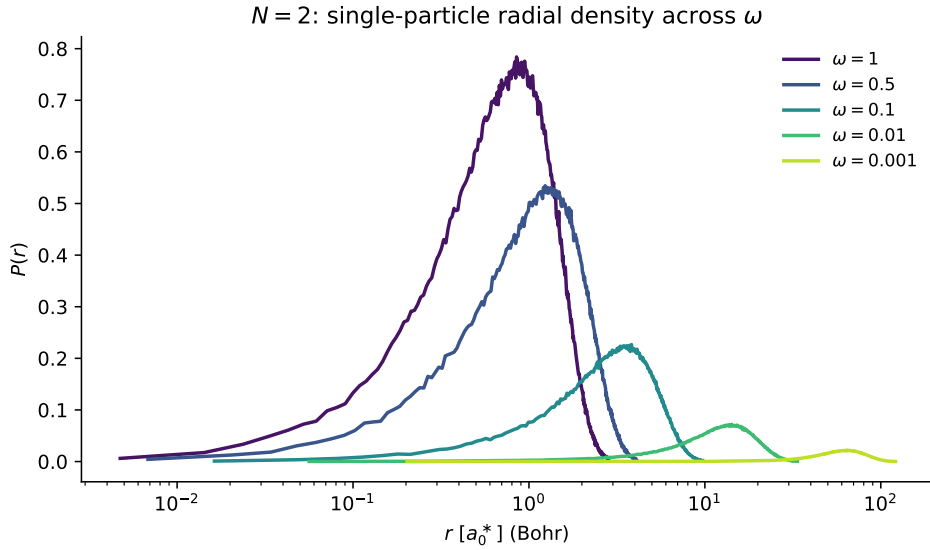
Figure 6.5: Two-electron radial densities P(r) across \omega .
