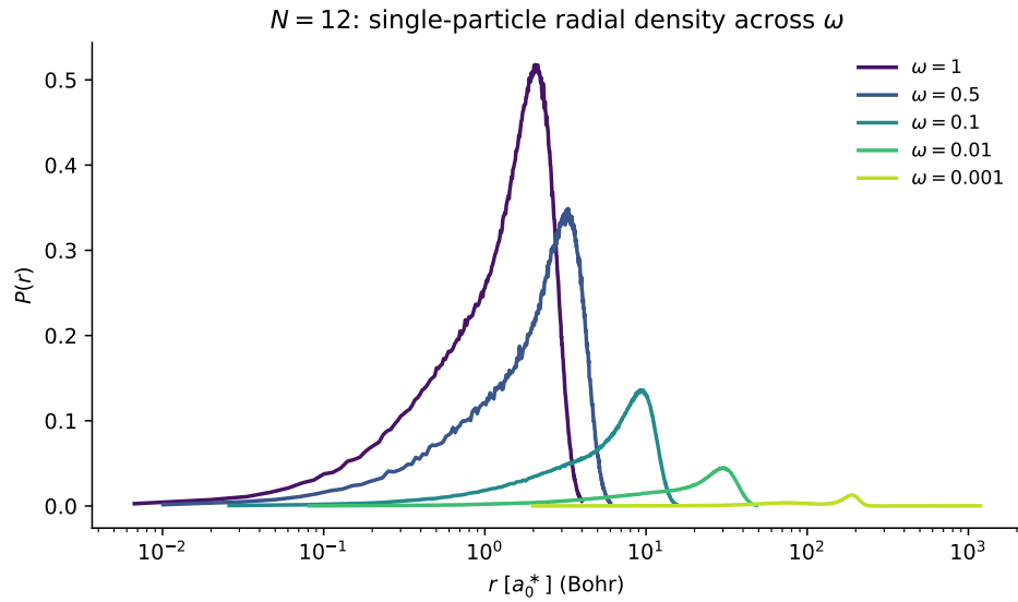
Figure 6.8: Twelve-electron radial densities P(r) across \omega .
