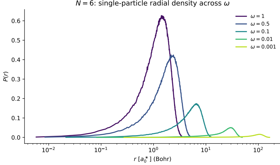
Figure 6.6: Six-electron radial densities P(r) across \omega .
