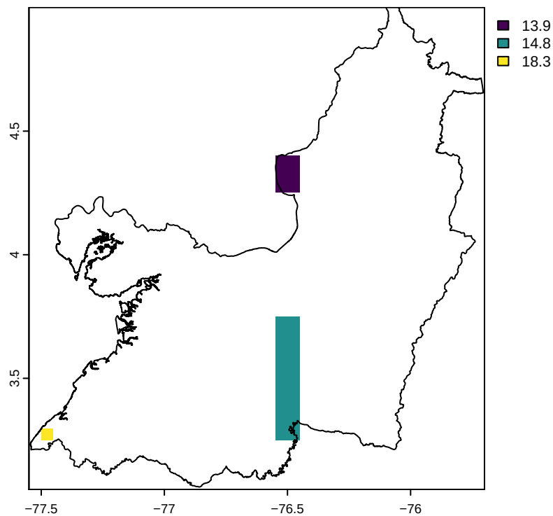
POWER: radiacion semanal
