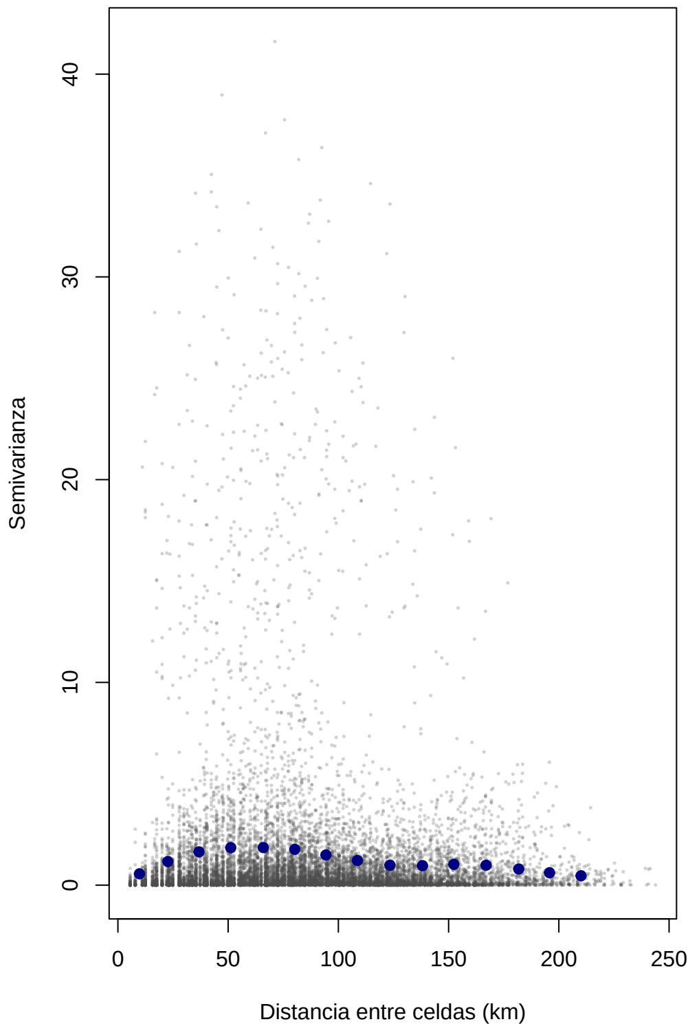
Nube de semivariograma residual
