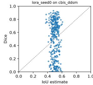
Fig. 4. IoU estimate against true Dice for LoRA on CBIS-DDSM at tight boxes: the estimate stays near 0.5 whether the mask is right or wrong.
