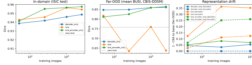
Fig. 3. Adapters trained for a fixed 6000 steps on nested subsets (log axis), zero-shot dashed. Left: in-domain Dice. Centre: far-OOD Dice, mean of BUSI and CBIS-DDSM. Right: far-OOD representation drift ( 1 - \text{CKA} to the base model) of the decoder’s up-scaled embedding (circles) and of the encoder neck output (squares, dashed); decoder-only fine-tuning leaves the encoder untouched. Single seed.
