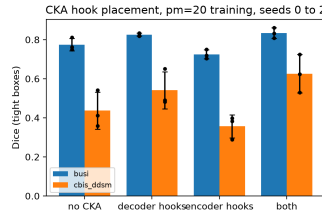
Fig. 2. Hook placement (LoRA, 20 px training, tight-box evaluation): far-OOD Dice with no regulariser, decoder hooks, encoder hooks, and both; bars are means over seeds 0 to 2 with one std, dots the individual seeds.
