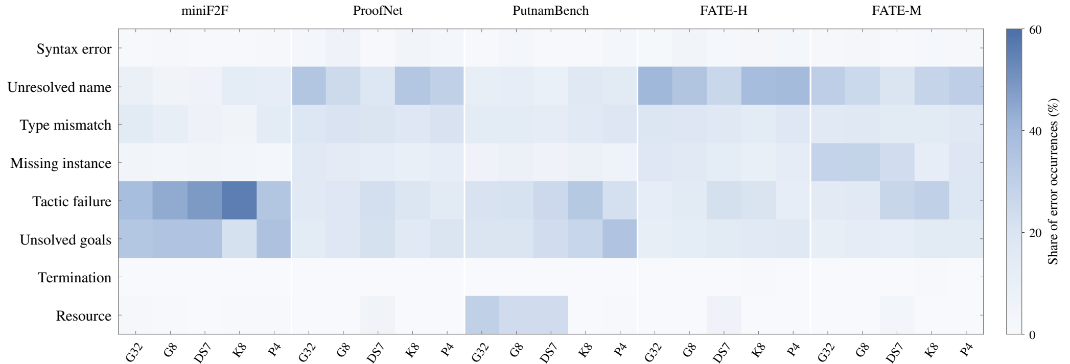
Diagnostic categories by model and benchmark
