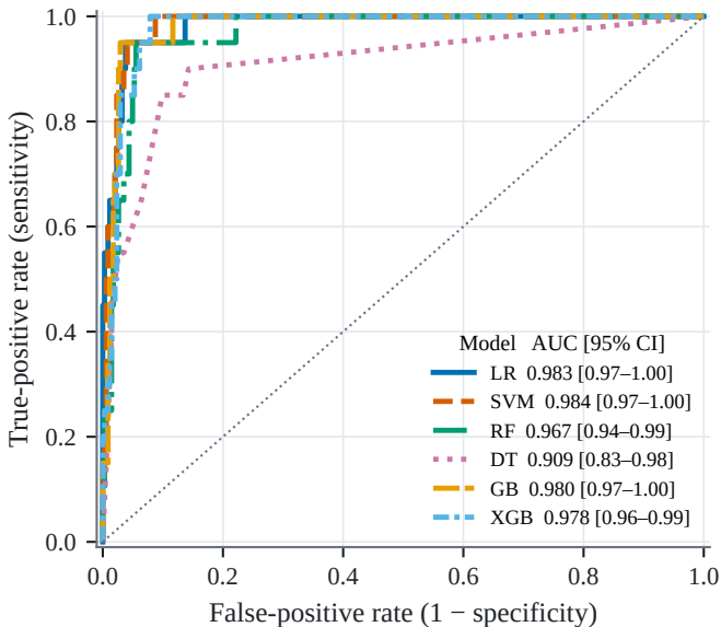
(a) ROC curves
