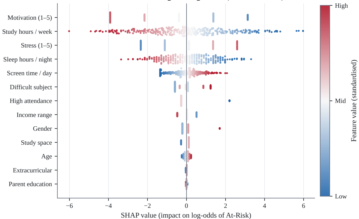
Global SHAP attributions — Logistic Regression (test set, n = 363)
