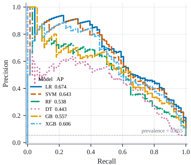
(b) Precision–recall
