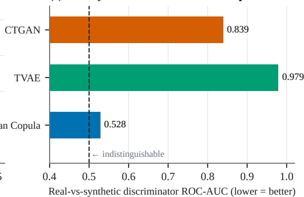
(c) Fidelity: can a classifier tell them apart?
