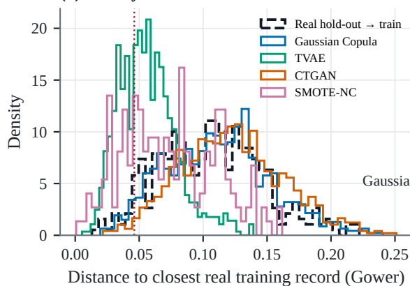
(b) Privacy: distance to closest record
