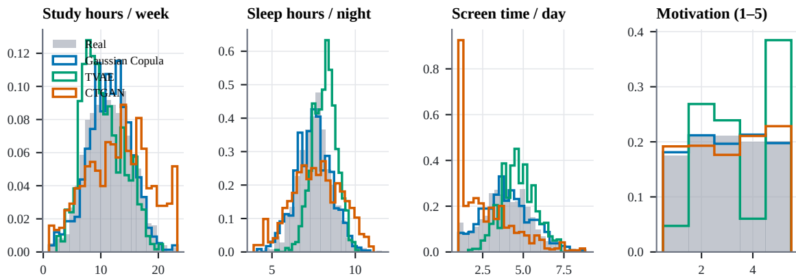
(a) Marginal distributions: real vs synthetic (training partition)
