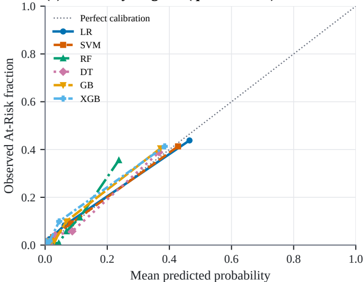
(a) Reliability diagram (quantile bins)
