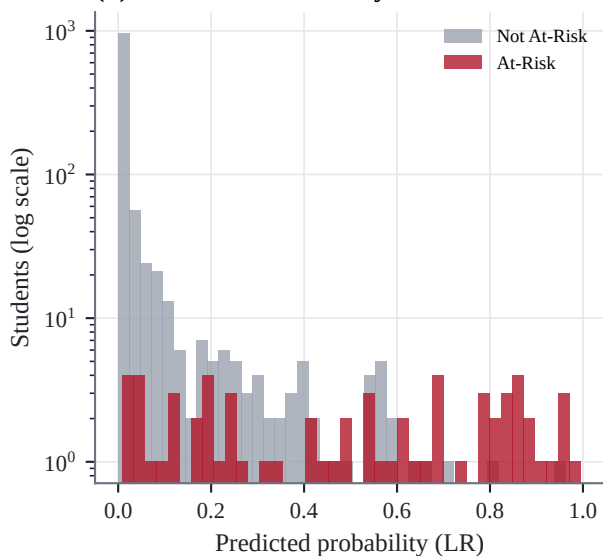
(b) Score distribution by class
