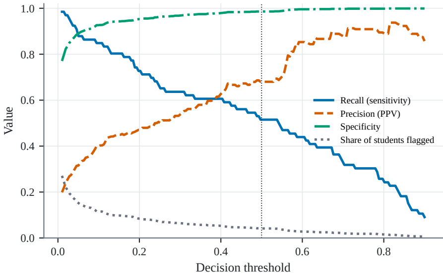
Threshold trade-off — Logistic Regression (out-of-fold)
