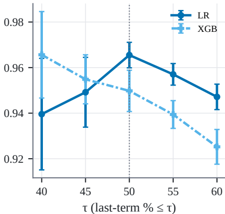
(a) ROC-AUC
