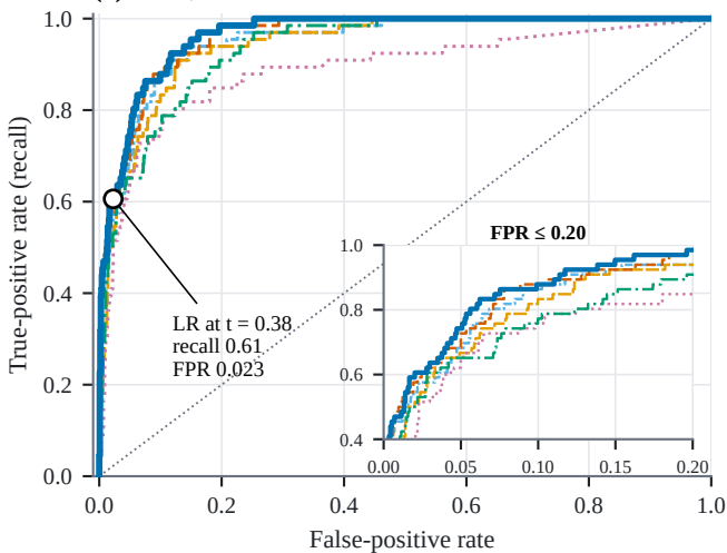
(a) ROC, out-of-fold
