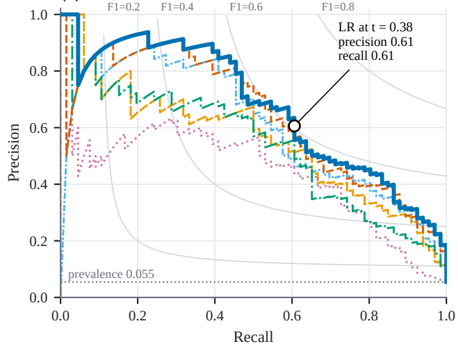
(b) Precision–recall, out-of-fold
