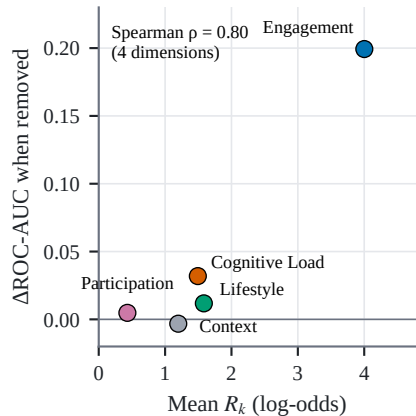
(c) Dimension ablation
