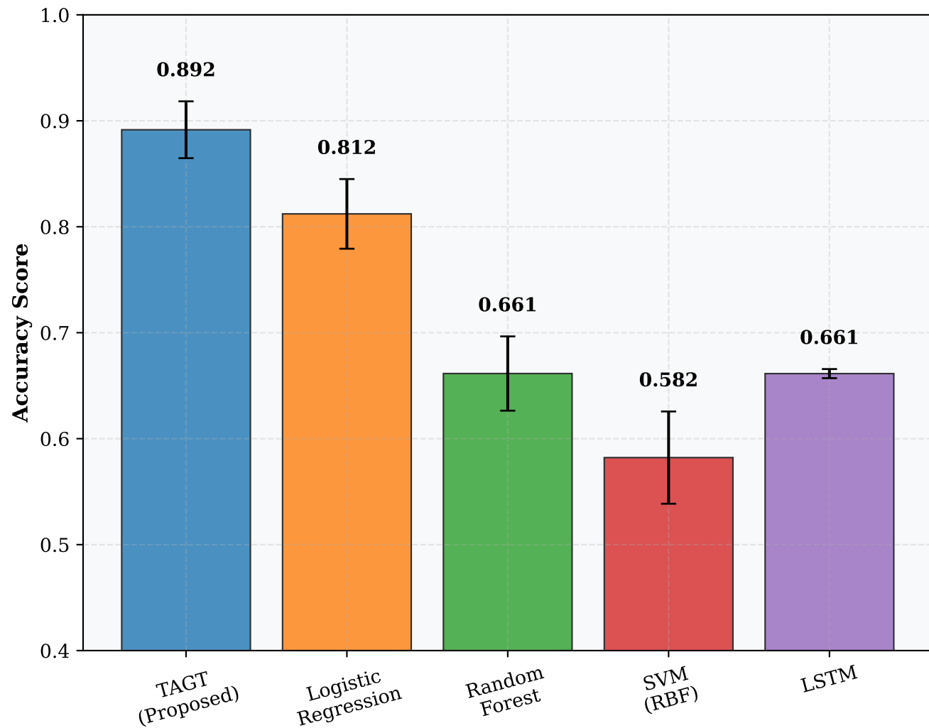
(B) Accuracy Performance Comparison
