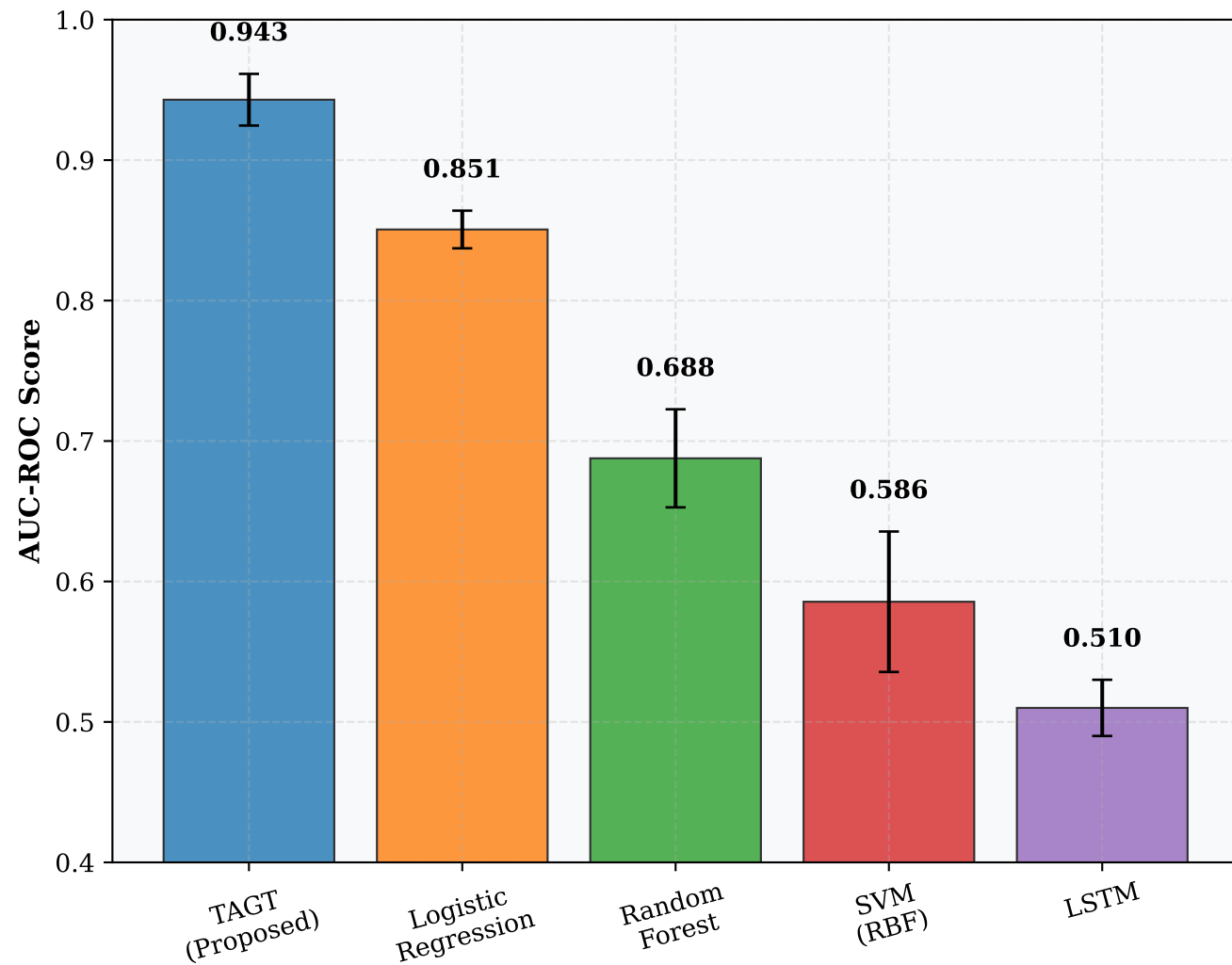
(A) AUC-ROC Performance Comparison
