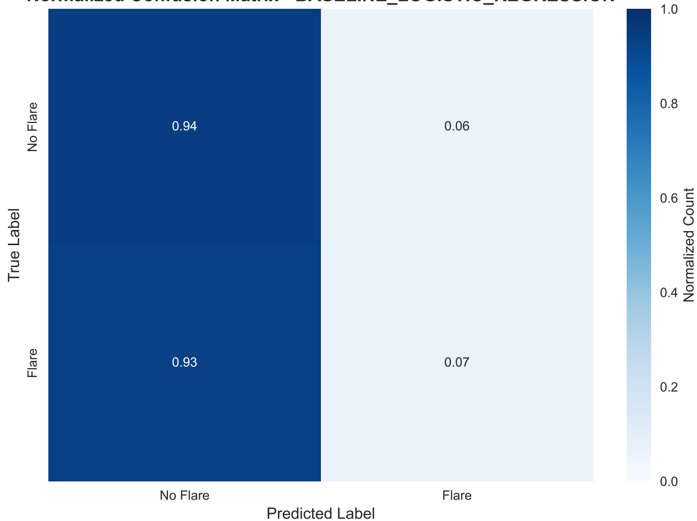
Normalized Confusion Matrix - BASELINE_LOGISTIC_REGRESSION
