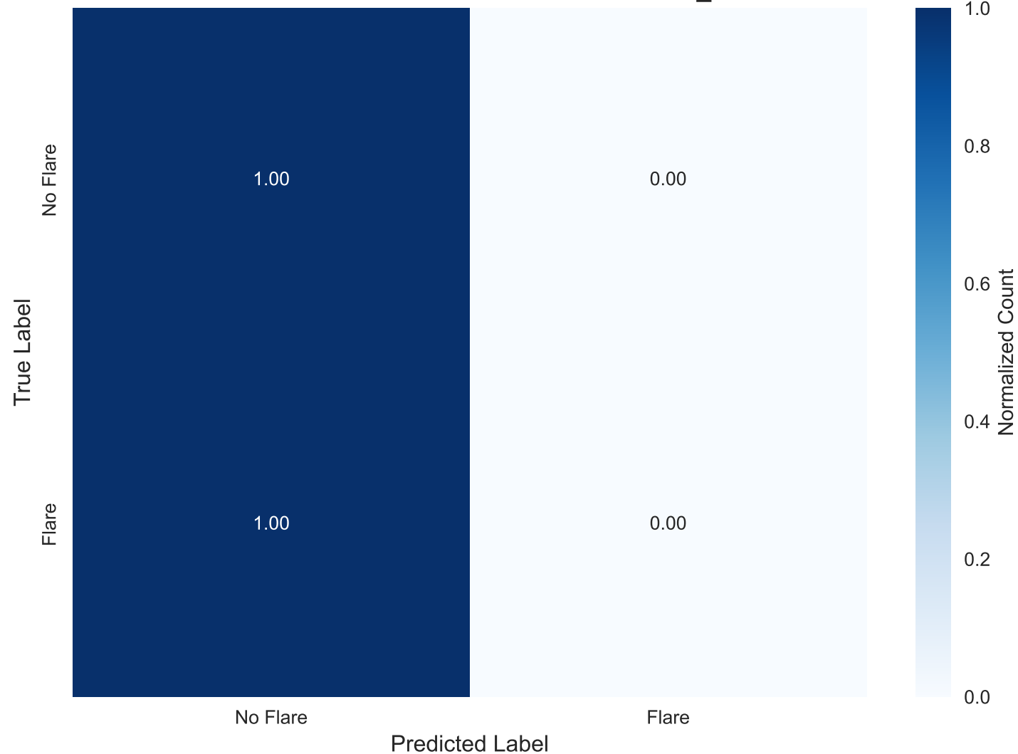
Normalized Confusion Matrix - BASELINE_SVM
