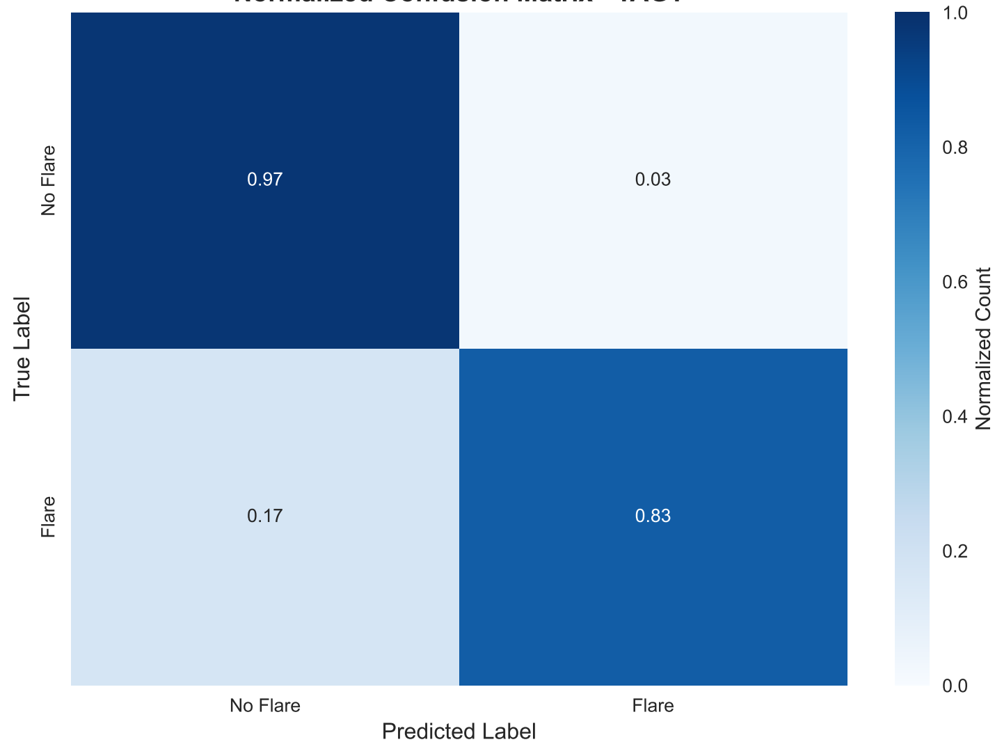
Normalized Confusion Matrix - TAGT
