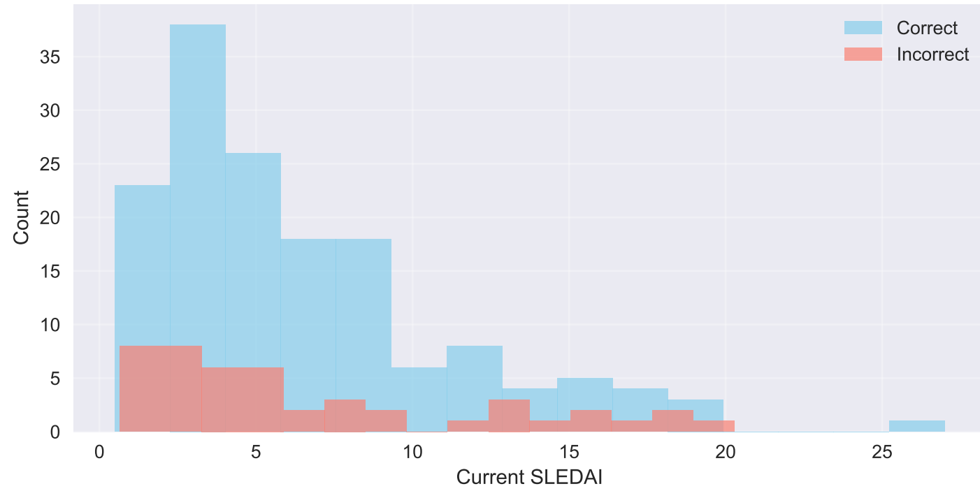
BASELINE_LOGISTIC_REGRESSION: Accuracy vs Current SLEDAI
