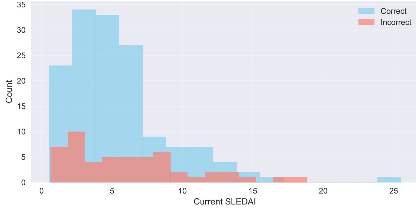
BASELINE_LSTM: Accuracy vs Current SLEDAI
