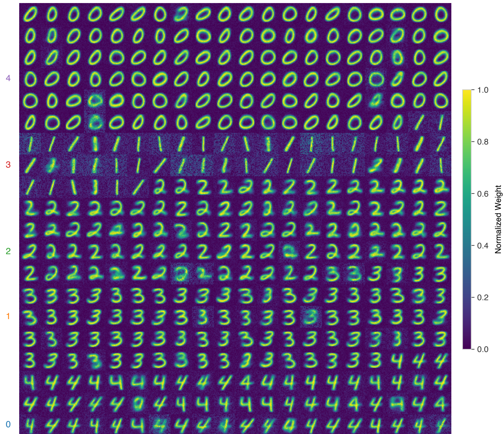
Learned Receptive Fields (400 neurons, sorted by class)
