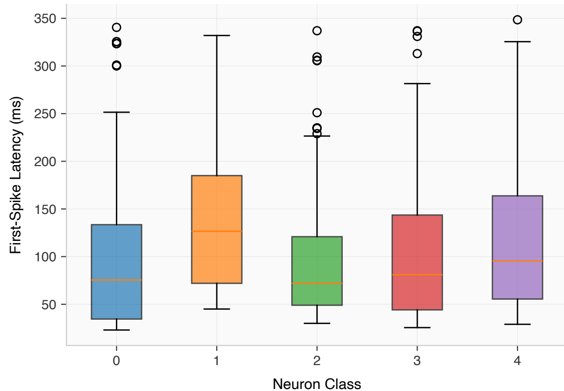
First-Spike Latency by Neuron Class
