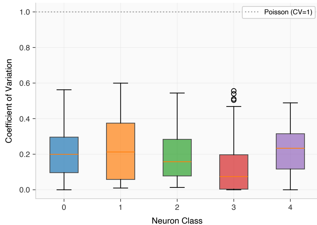
ISI Regularity by Neuron Class
