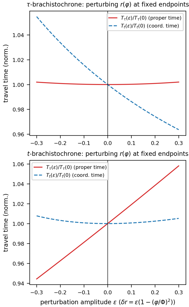
Figure A5. Each branch minimizes its own travel time; t and \tau are distinct curves.
