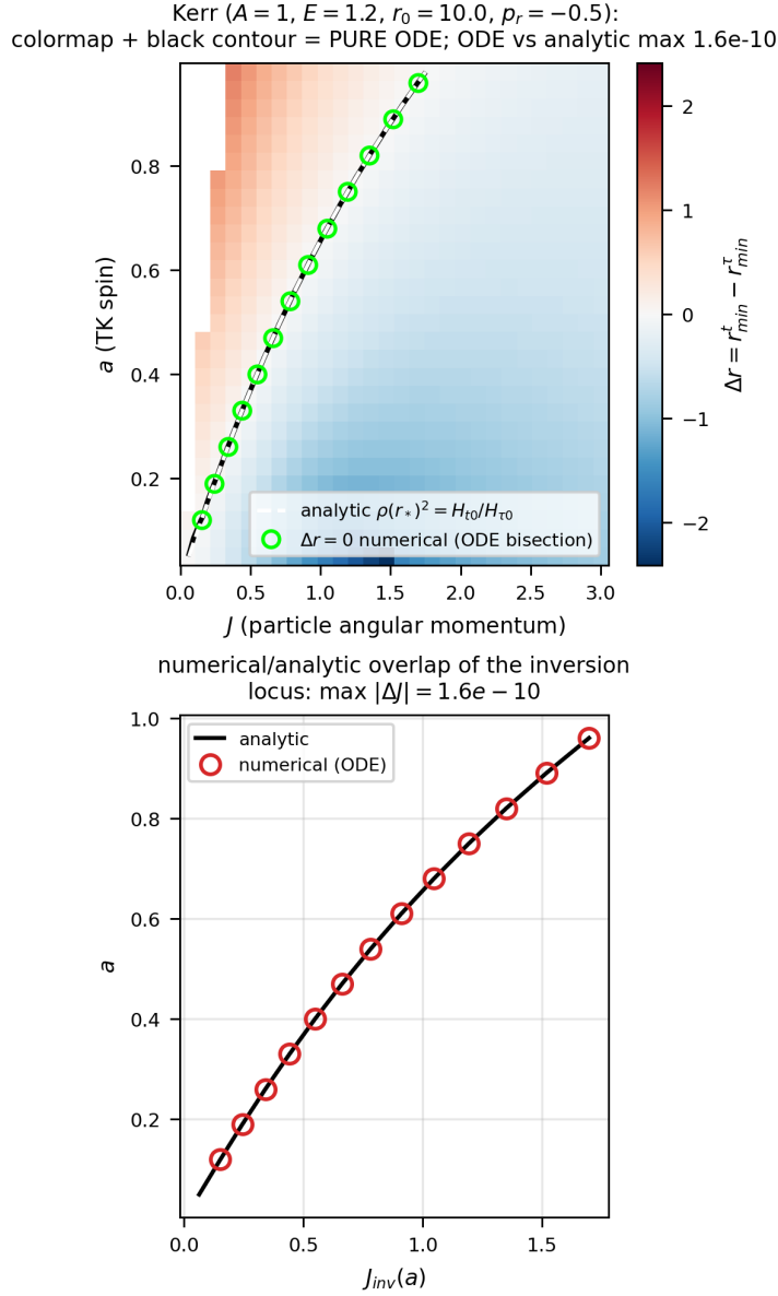
Figure 11. Rotational inversion in the (a, J) plane; ODE locus vs analytic \rho(r_*)^2 = H_{t0}/H_{\tau0} .
