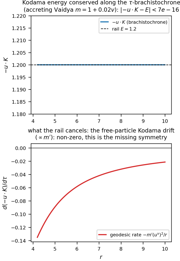
FIG. 4. Kodama energy -u \cdot K = \hat{E} conserved along the \tau -brachistochrone to 6.7 \times 10^{-16} (top); the free-particle drift \propto m' that the rail cancels (bottom).
