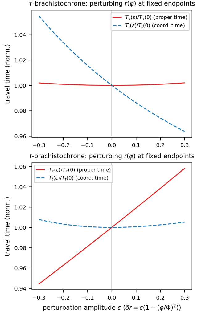
FIG. 19. Each branch minimizes its own travel time; t and \tau are distinct curves.
