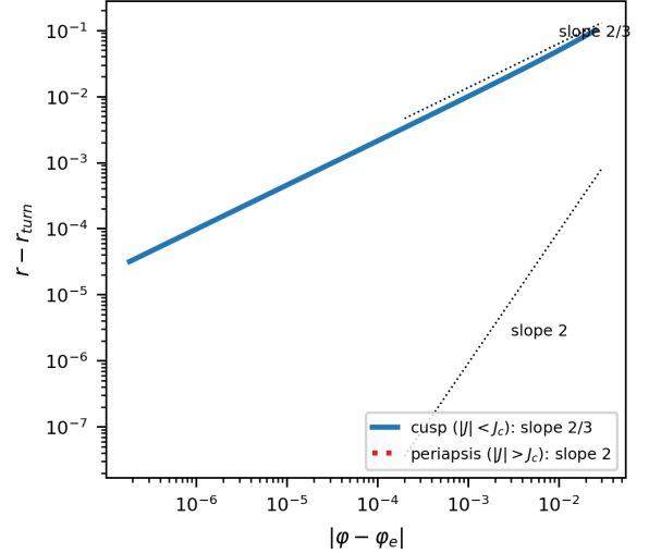
FIG. 10. Reflection at the ergosphere: cusp ( |J| < J_c ), smooth crossing to r_+ in Doran coordinates ( |J| = J_c ), smooth periapsis ( |J| > J_c ); power law 2/3 vs 2 .
