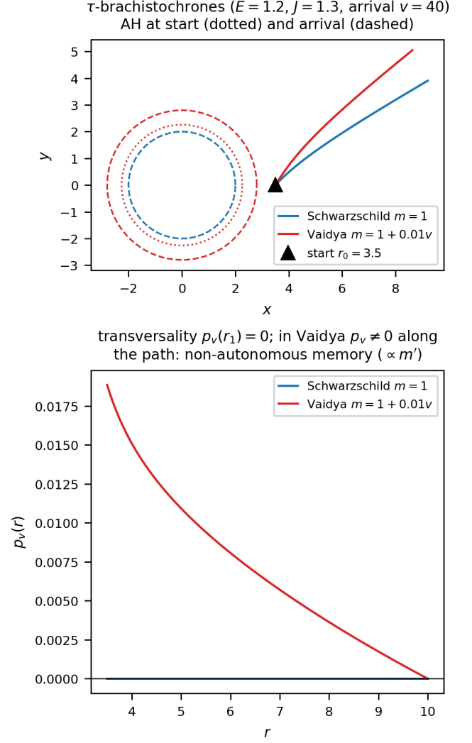
FIG. 5. \tau -brachistochrones Schwarzschild vs Vaidya, and p_v(r) : transversality p_v(r_1) = 0 , non-autonomous memory \propto m' .
