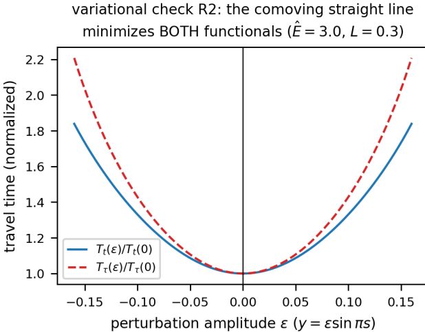
FIG. 3. Variational check: the comoving straight line minimizes both T_t and T_\tau (branch degeneracy).
