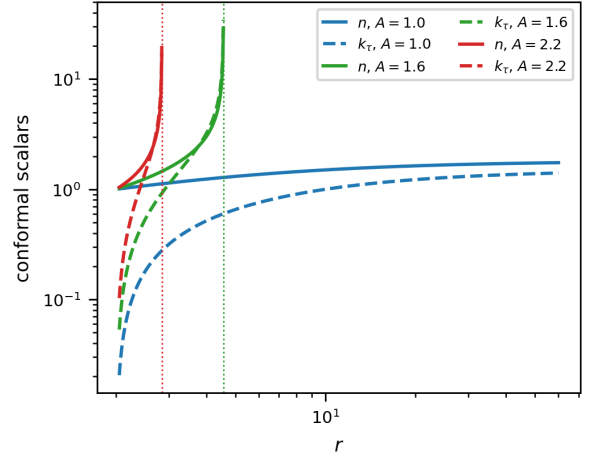
FIG. 8. The three branches: \tau bounces (mirror pair, no wind), \eta spirals (gravitomagnetic wind); breathing conformal scalars n, k_\tau .
