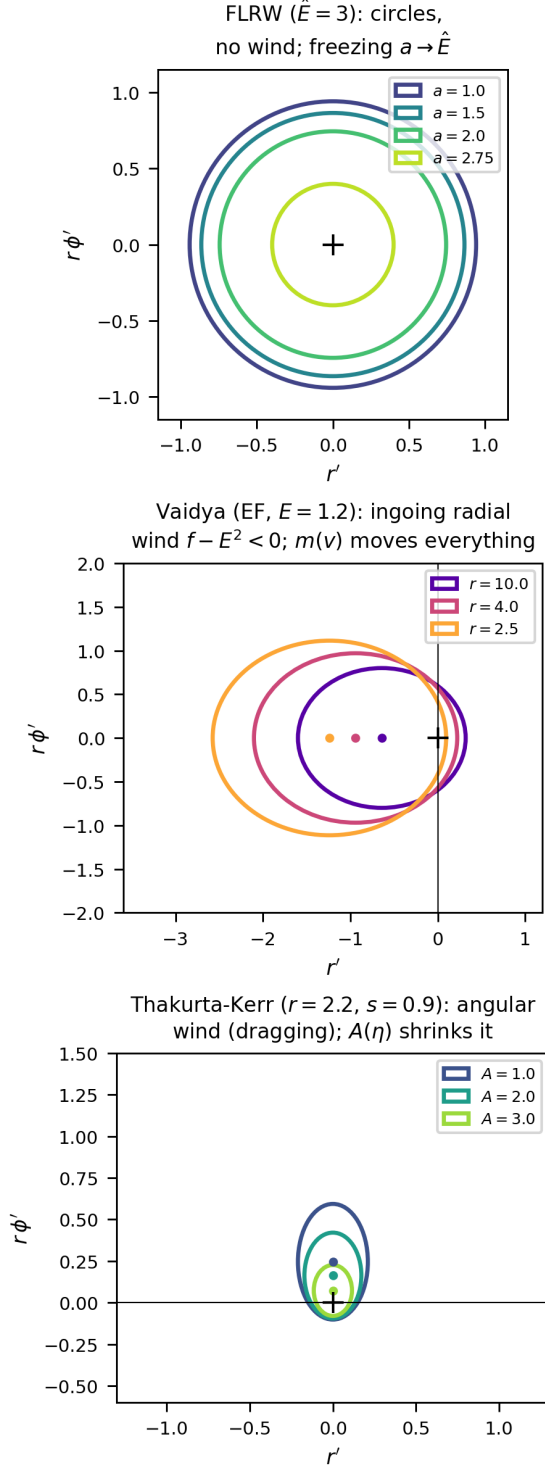
Rail indicatrices (linear constraint n normalization = ellipse): the unifying formalism
