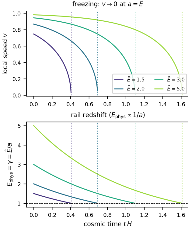
FIG. 2. de Sitter FLRW rail kinematics: local speed v and rail redshift E_{\text{phys}} = \hat{E}/a ; freezing at a = \hat{E} .
