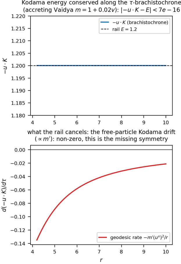
FIG. 4. Kodama energy -u \cdot K = \hat{E} conserved along the \tau -brachistochrone to 6.7 \times 10^{-16} (top); the free-particle drift \propto m' that the rail cancels (bottom).
