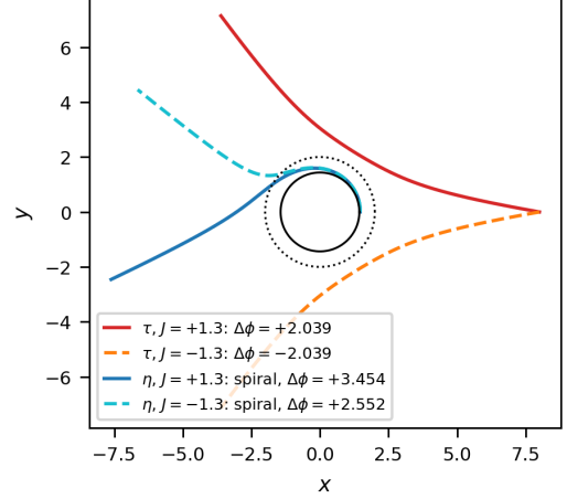
the two scalars breathing on the rigid geometry \alpha_K :
