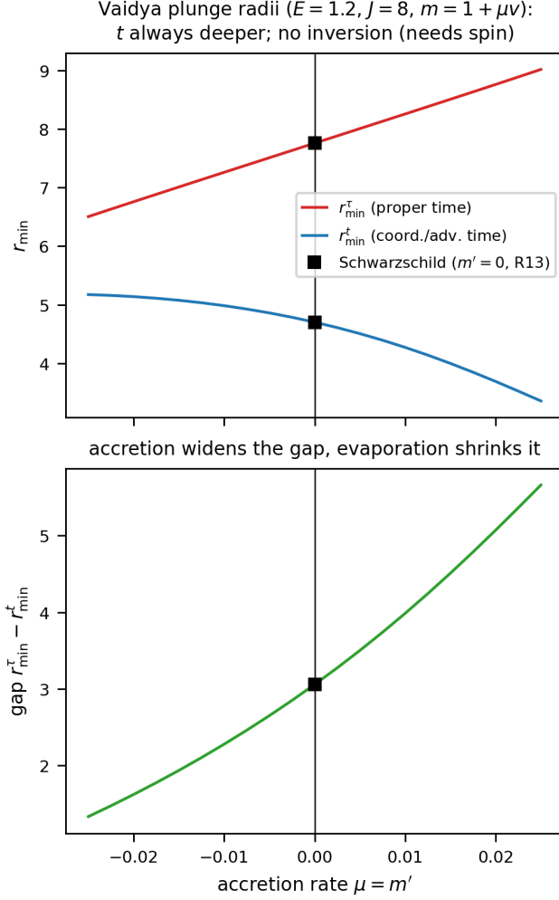
FIG. 6. Plunge radii r_{\min}^{t,\tau} and gap vs \mu = m' ; t deeper, accretion widens the gap.
