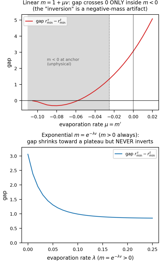
FIG. 7. No physical evaporative inversion: the linear-model sign change lies entirely in the unphysical m < 0 region; with m = e^{-\lambda v} > 0 the gap shrinks but never inverts.
